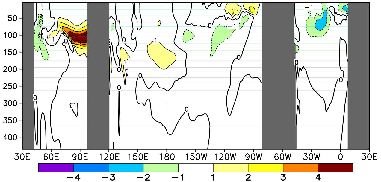
FIGURE T17. Equatorial depth–longitude section of ocean temperature (top) and ocean temperature anomalies (bottom) for JUL 2014. Contour interval is 1°C. Dashed contours in bottom panel indicate negative anomalies. Data are derived from the NCEP’s global ocean data assimilation system version 2 which assimilates oceanic observations into an oceanic GCM (Xue, Y. and Behringer, D.W., 2006: Operational global ocean data assimilation system at NCEP, to be submitted to BAMS). Anomalies are departures from the 1981–2010 base period means.
