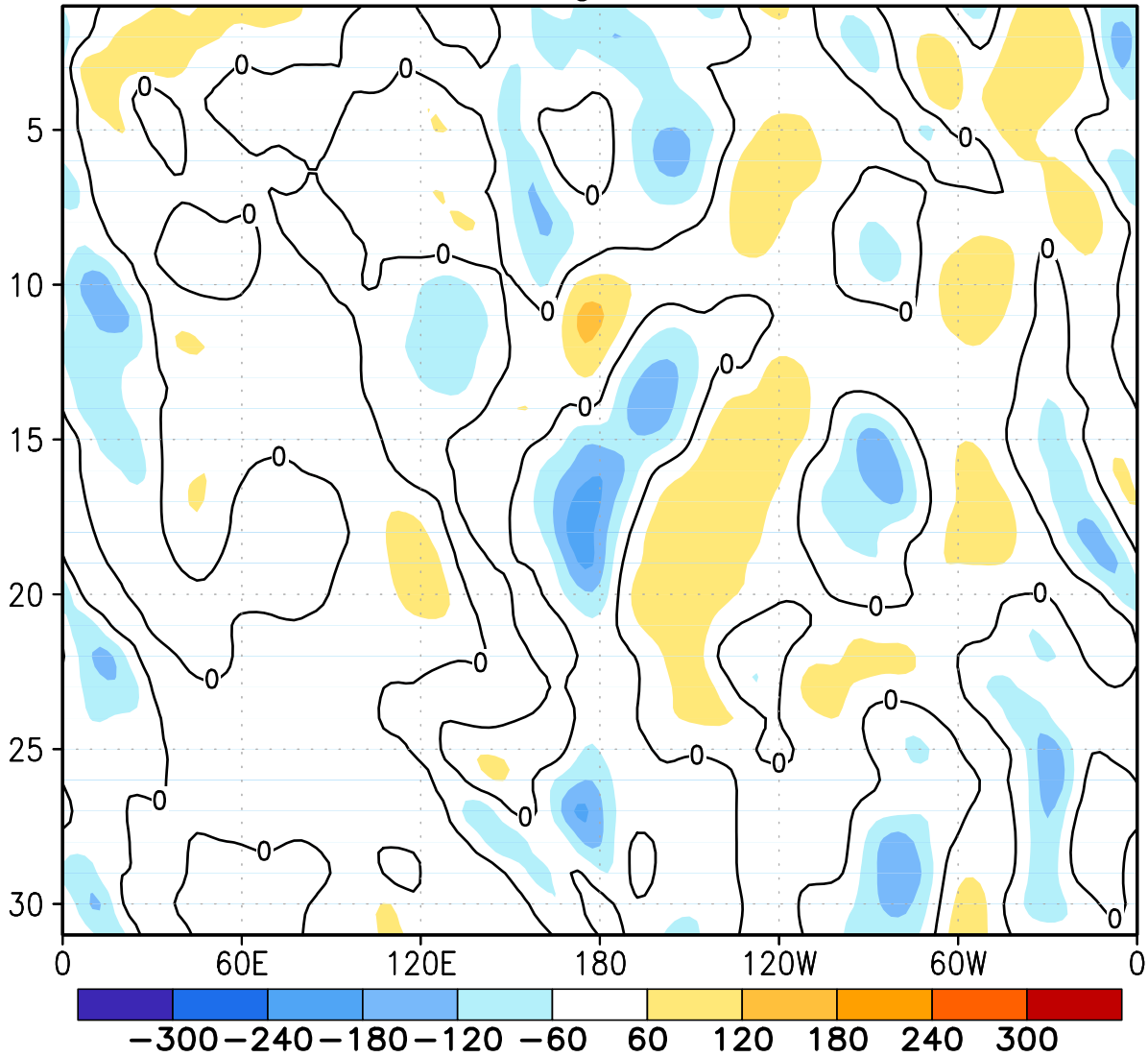
FIGURE E12. Northern Hemisphere: Daily 500-hPa height anomalies for JUL 2014 averaged over the 5° latitude band centered on 40°N. Positive values are indicated by solid contours and dark shading. Negative values are indicated by dashed contours and light shading. Contour interval is 60 m. Anomalies are departures from the 1981-2010 base period daily means.
