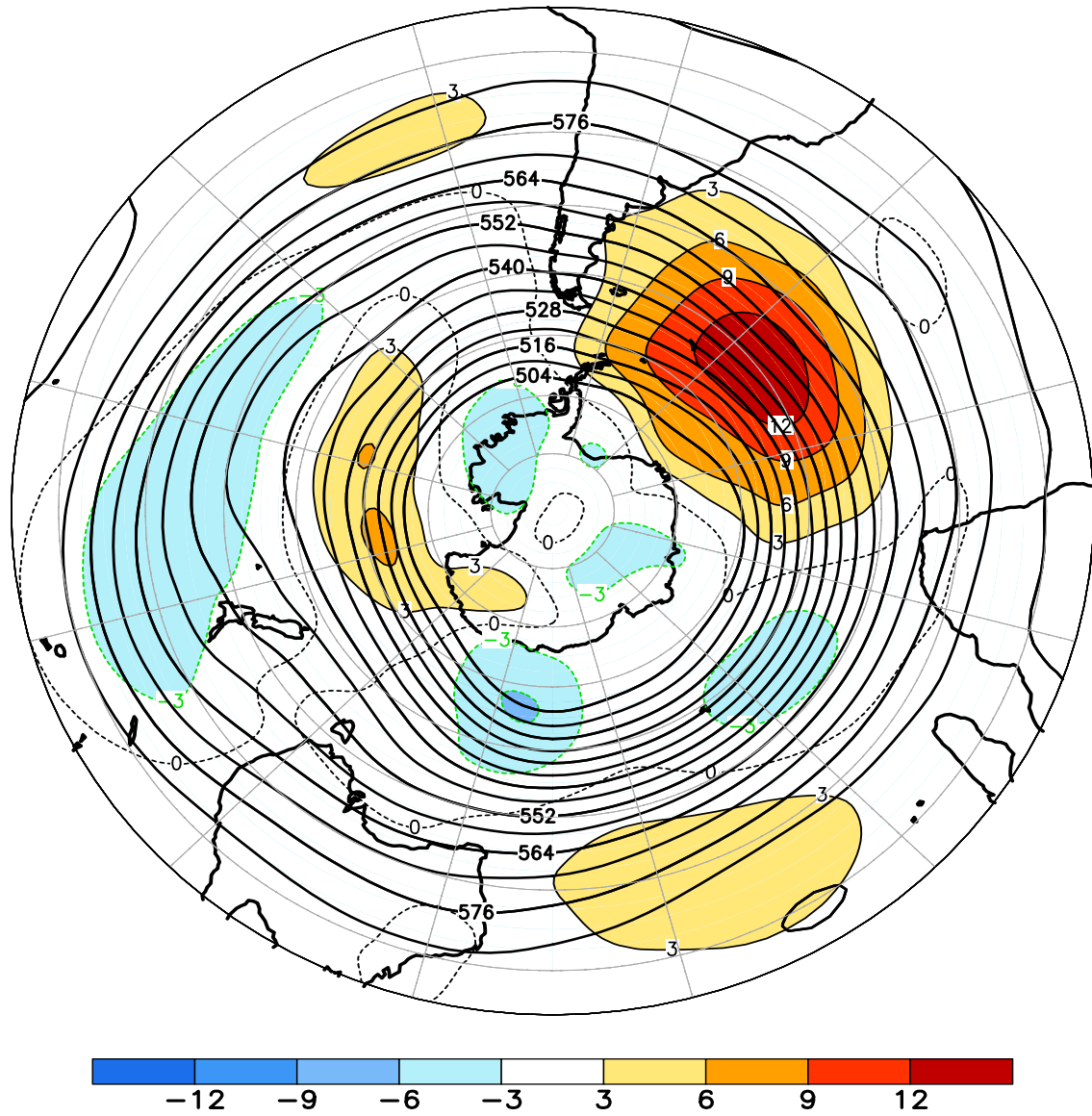
FIGURE E15. Southern Hemisphere mean and anomalous 500-hPa geopotential height (CDAS/Reanalysis) for JUL 2014. Mean heights are denoted by solid contours drawn at an interval of 6 dam. Anomaly contour interval is 3 dam with values less (greater) than -3 dam (3 dam) indicated by dark (light) shading. Anomalies are calculated as departures from the 1981-2010 base period monthly means.
