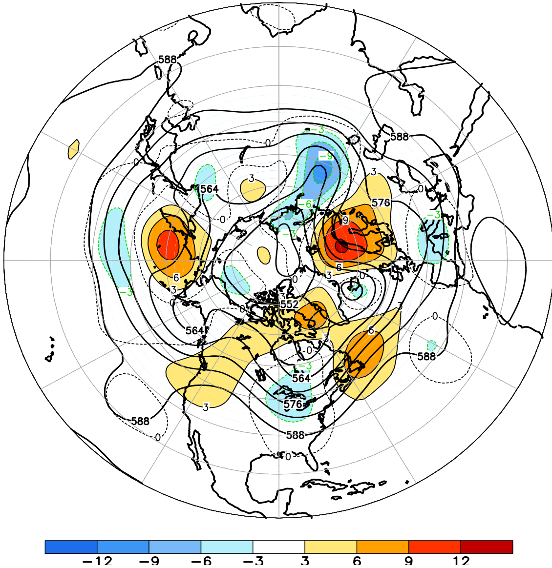
FIGURE E9. Northern Hemisphere mean and anomalous 500-hPa geopotential height (CDAS/Reanalysis) for JUL 2014. Mean heights are denoted by solid contours drawn at an interval of 6 dam. Anomaly contour interval is 3 dam with values less (greater) than -3 dam (3 dam) indicated by dark (light) shading. Anomalies are calculated as departures from the 1981-2010 base period monthly means.
