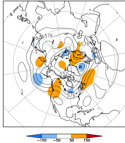
500-hPa Height (dm) & Anomalies (m) (Jul 1–15, 2014)
