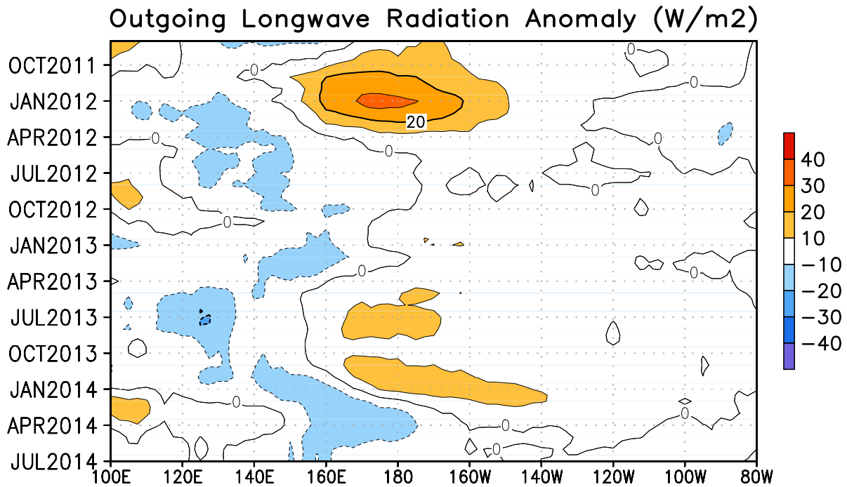
FIGURE T8. Time-longitude section of mean (top) and anomalous (bottom) outgoing longwave radiation (OLR) averaged between 5N-5S. Contour interval is 10 \text{Wm}^{-2} . Dashed contours in bottom panel indicate negative OLR anomalies. Anomalies are departures from the 1981-2010 base period monthly means. The data are smoothed temporally using a 3-month running average.
