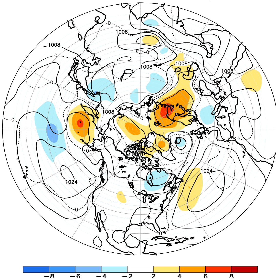
FIGURE E8. Northern Hemisphere mean and anomalous sea level pressure (CDAS/Reanalysis) for JUL 2014. Mean values are denoted by solid contours drawn at an interval of 4 hPa. Anomaly contour interval is 2 hPa with values less (greater) than -2 hPa (2 hPa) indicated by dark (light) shading. Anomalies are calculated as departures from the 1981-2010 base period monthly means.
