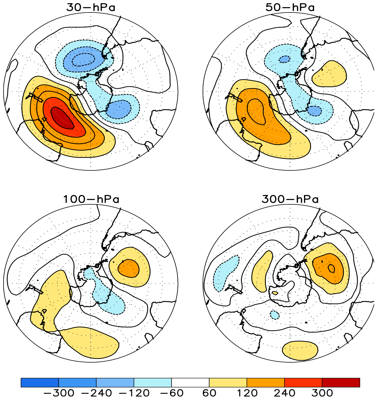
FIGURE S1. Stratospheric height anomalies (m) at selected levels for JUL 2014. Positive values are indicated by solid contours and dark shading. Negative values are indicated by dashed contours and light shading. Contour interval is 60 m. Anomalies are calculated from the 1981-2010 base period means. Winter Hemisphere is shown.
