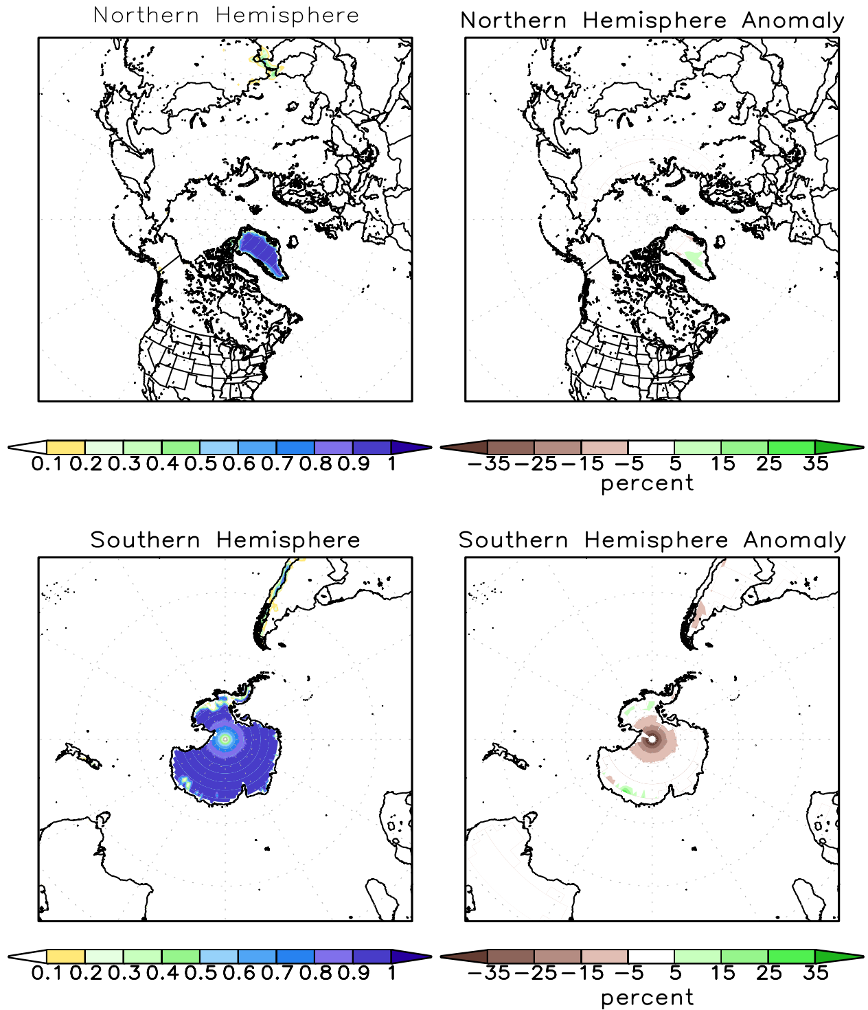
FIGURE A2.2. SSM/I derived snow cover frequency (%) (left) and snow cover anomaly (%) (right) for the month of JUL 2014 based on 1987 - 2010 base period for the Northern Hemisphere (top) and Southern Hemisphere (bottom). It is generated using the algorithm described by Ferraro et. al, 1996, Bull. Amer. Meteor. Soc., vol 77, 891-905.
