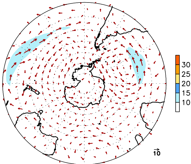
FIGURE E16. Southern Hemisphere mean (left) and anomalous (right) 300-hPa vector wind (CDAS/Reanalysis) for JUL 2014. Mean (anomaly) isotach contour interval is 10 (5) \text{ms}^{-1} . Values greater than 30 \text{ms}^{-1} (left) and 10 \text{ms}^{-1} (rights) are shaded. Anomalies are departures from the 1981-2010 base period monthly means.
