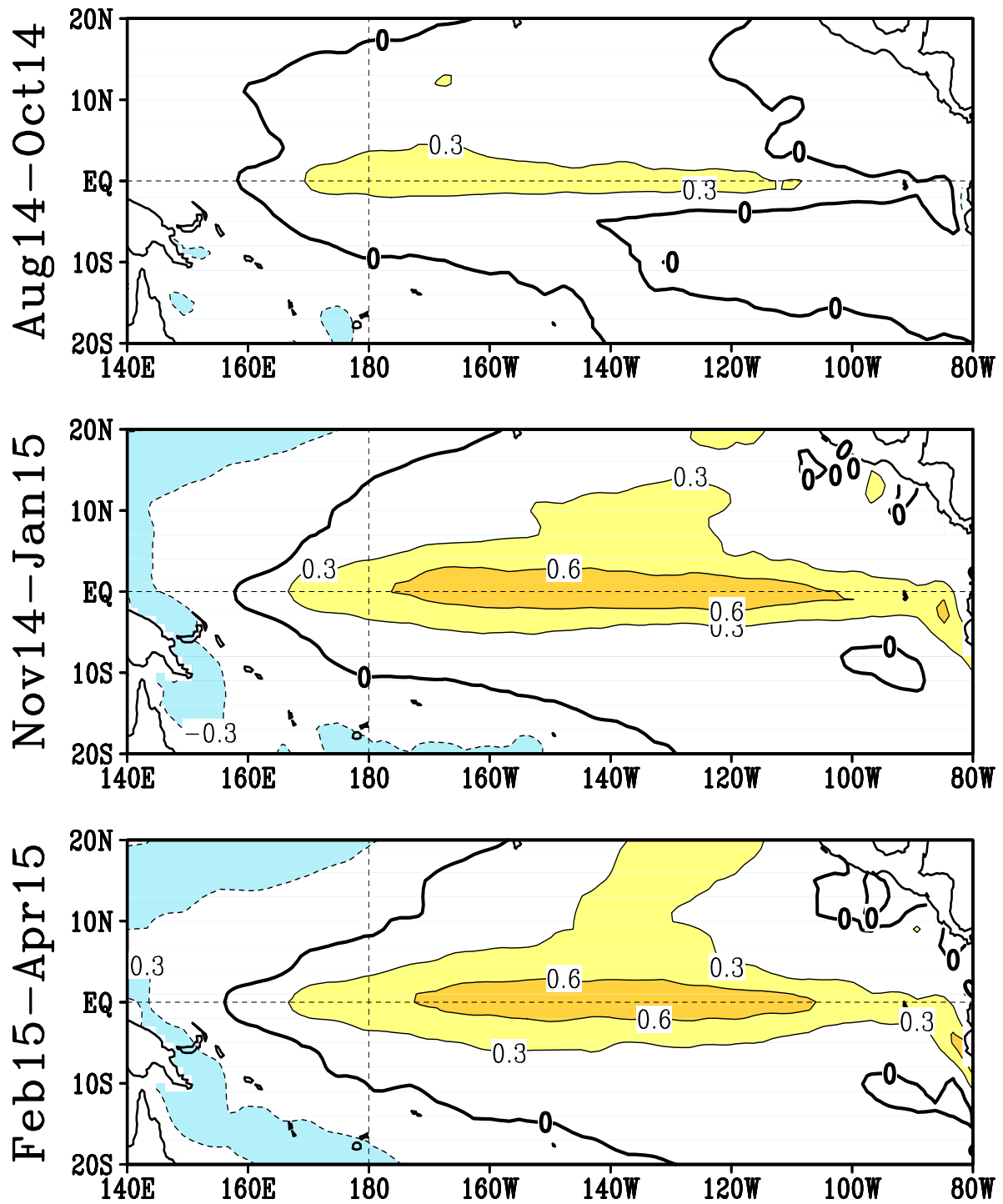
FIGURE F5. Predicted 3-month average sea surface temperature anomalies from the NCEP/CPC Markov model (Xue et al. 2000, J. Climate , 13 , 849-871). The forecast is initiated in JUL 2014 . Contour interval is 0.3C and negative anomalies are indicated by dashed contours. Anomalies are calculated relative to the 1971-2000 climatology.
