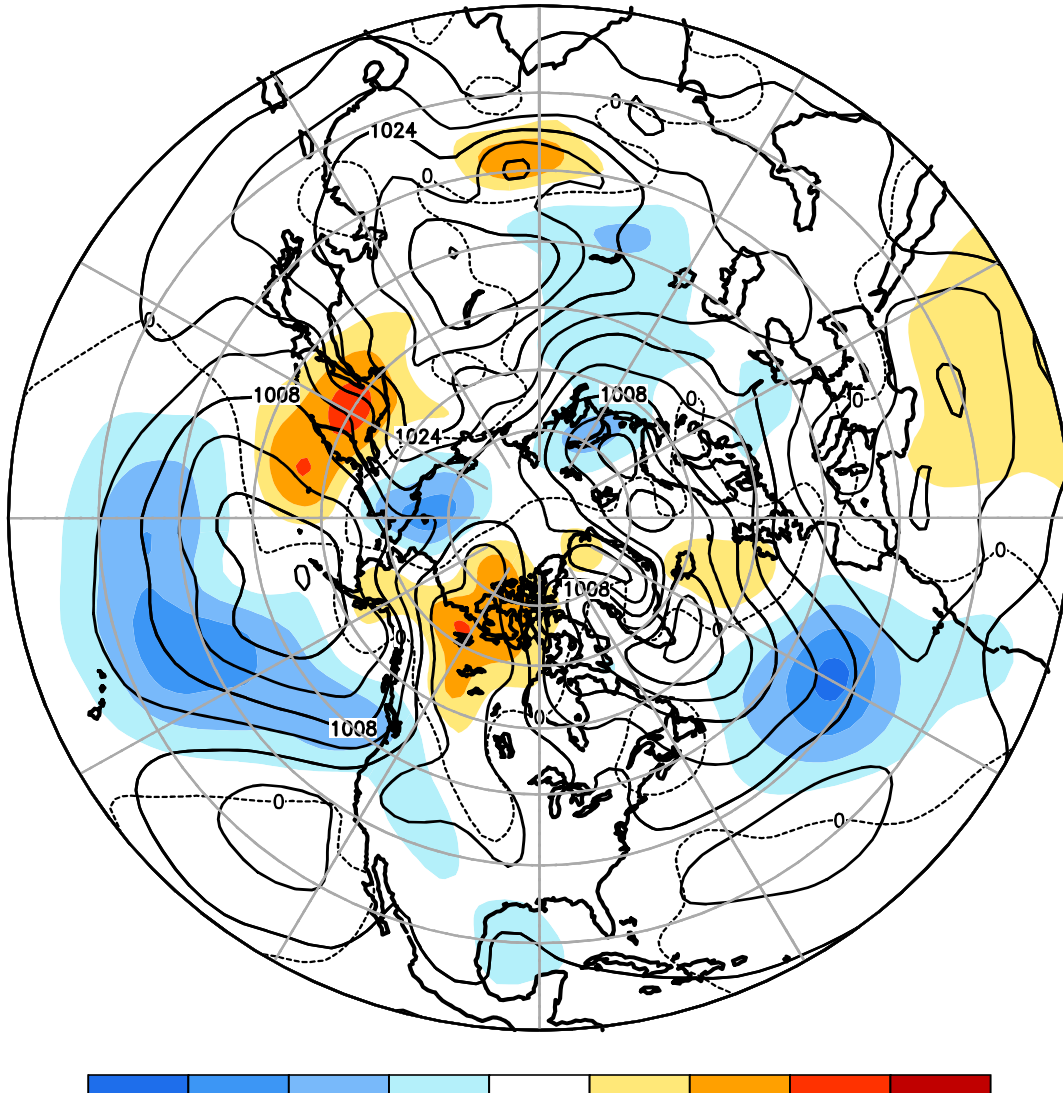
FIGURE E8. Northern Hemisphere mean and anomalous sea level pressure (CDAS/Reanalysis) for JAN 2024. Mean values are denoted by solid contours drawn at an interval of 4 hPa. Anomaly contour interval is 2 hPa with values less (greater) than -2 hPa (2 hPa) indicated by dark (light) shading. Anomalies are calculated as departures from the 1991-2020 base period monthly means.
