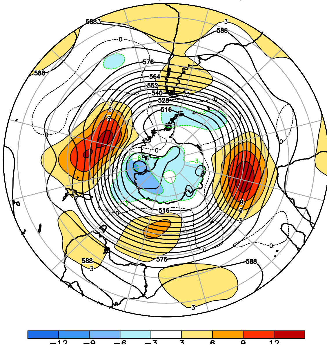
FIGURE E15. Southern Hemisphere mean and anomalous 500-hPa geopotential height (CDAS/Reanalysis) for JAN 2024. Mean heights are denoted by solid contours drawn at an interval of 6 dam. Anomaly contour interval is 3 dam with values less (greater) than -3 dam (3 dam) indicated by dark (light) shading. Anomalies are calculated as departures from the 1991-2020 base period monthly means.
