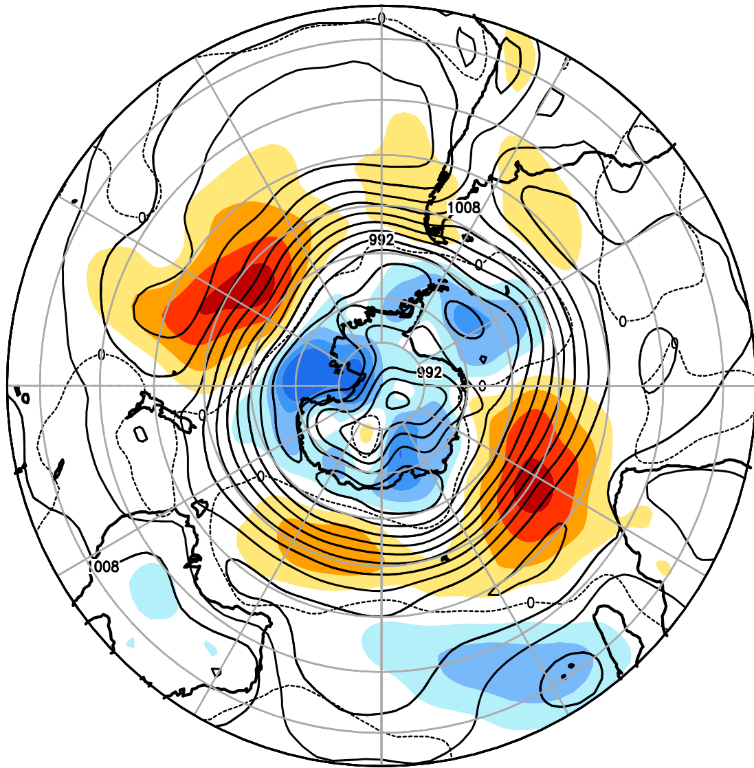
FIGURE E14. Southern Hemisphere mean and anomalous sea level pressure(CDAS/Reanalysis) for JAN 2024. Mean values are denoted by solid contours drawn at an interval of 4 hPa. Anomaly contour interval is 2 hPa with values less (greater) than -2 hPa (2 hPa) indicated by dark (light) shading. Anomalies are calculated as departures from the 1991-2020 base period monthly means.
