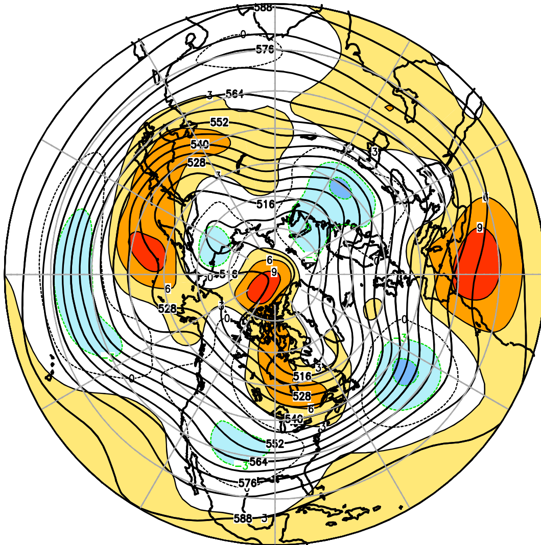
FIGURE E9. Northern Hemisphere mean and anomalous 500-hPa geopotential height (CDAS/Reanalysis) for JAN 2024. Mean heights are denoted by solid contours drawn at an interval of 6 dam. Anomaly contour interval is 3 dam with values less (greater) than -3 dam (3 dam) indicated by dark (light) shading. Anomalies are calculated as departures from the 1991-2020 base period monthly means.
