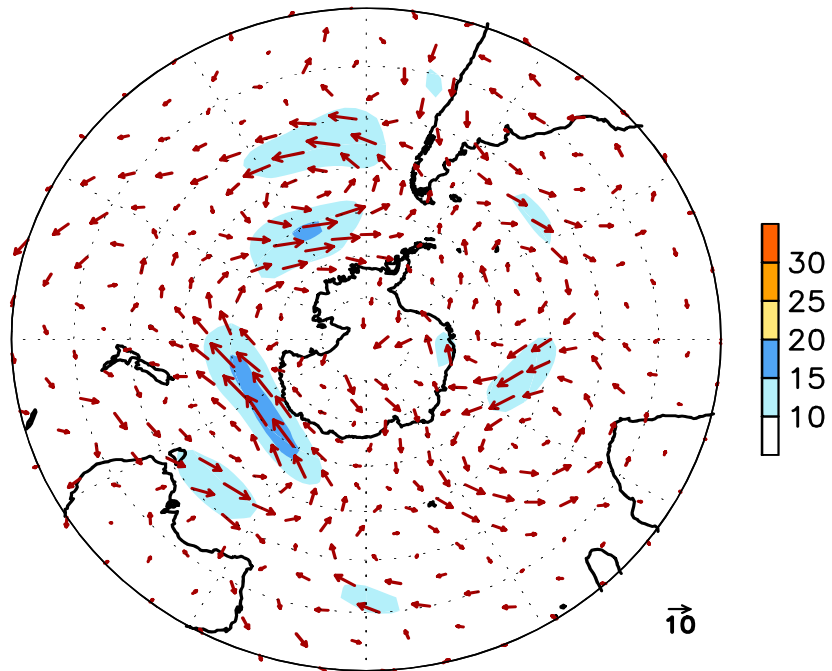
FIGURE E16. Southern Hemisphere mean (left) and anomalous (right) 300-hPa vector wind (CDAS/Reanalysis) for JAN 2022. Mean (anomaly) isotach contour interval is 10 (5) \text{ms}^{-1} . Values greater than 30 \text{ms}^{-1} (left) and 10 \text{ms}^{-1} (rights) are shaded. Anomalies are departures from the 1991-2020 base period monthly means.
