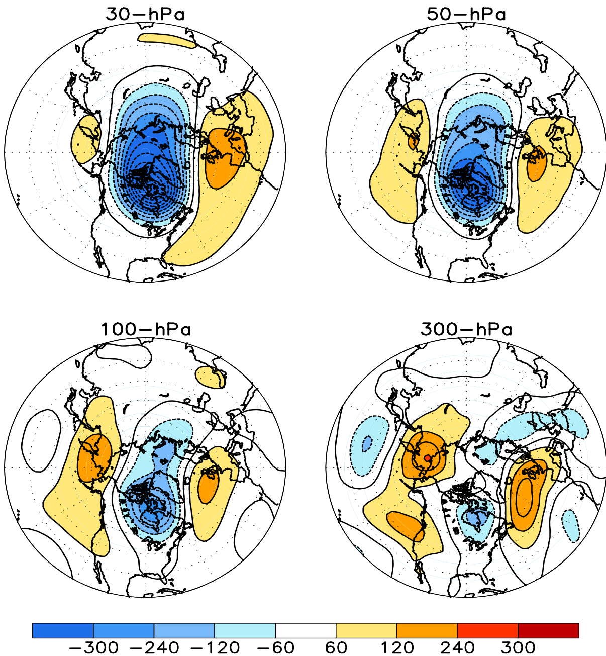
FIGURE S1. Stratospheric height anomalies (m) at selected levels for JAN 2022. Positive values are indicated by solid contours and dark shading. Negative values are indicated by dashed contours and light shading. Contour interval is 60 m. Anomalies are calculated from the 1991-2020 base period means. Winter Hemisphere is shown.
