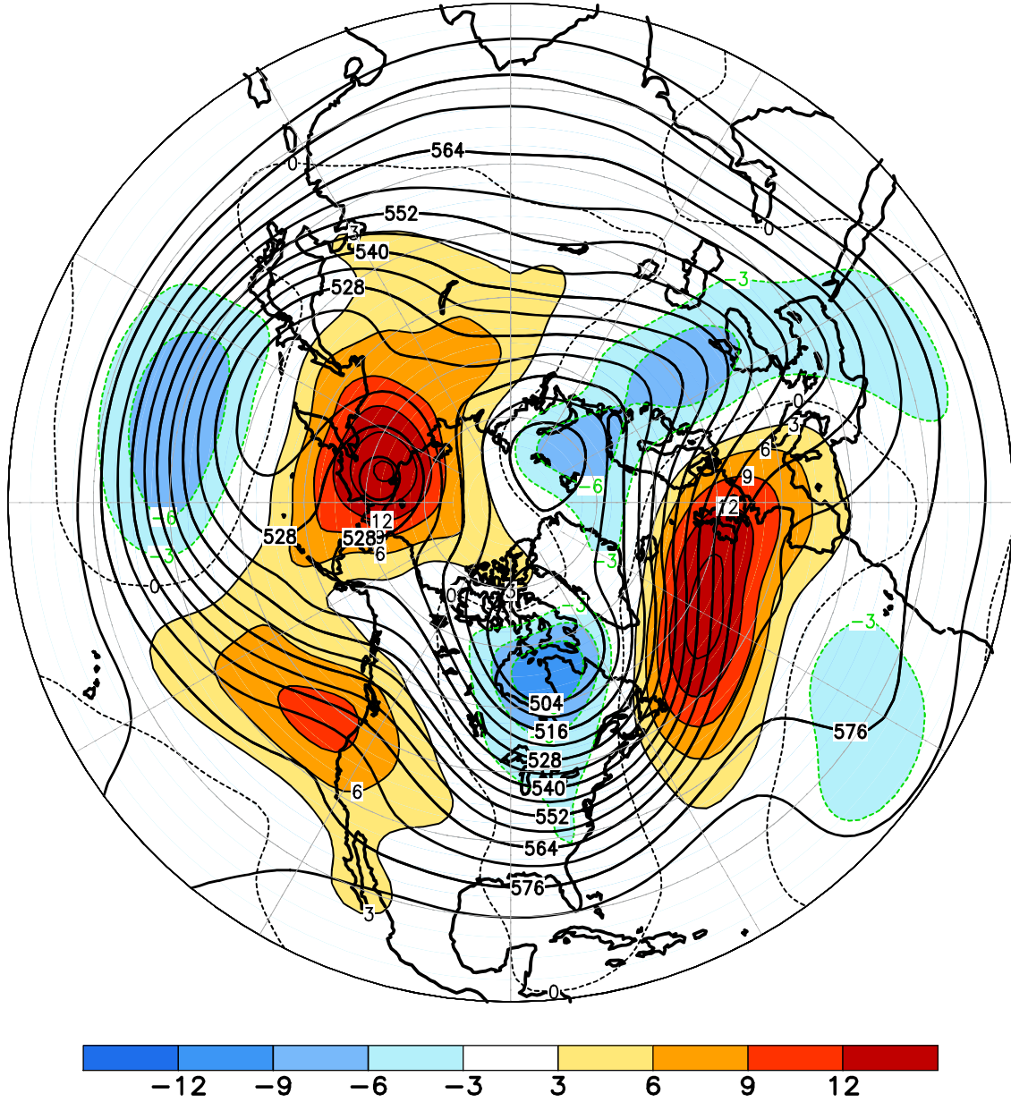
FIGURE E9. Northern Hemisphere mean and anomalous 500-hPa geopotential height (CDAS/Reanalysis) for JAN 2022. Mean heights are denoted by solid contours drawn at an interval of 6 dam. Anomaly contour interval is 3 dam with values less (greater) than -3 dam (3 dam) indicated by dark (light) shading. Anomalies are calculated as departures from the 1991-2020 base period monthly means.
