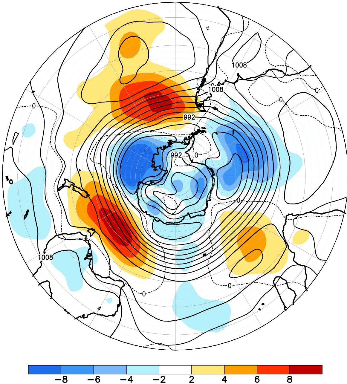
FIGURE E14. Southern Hemisphere mean and anomalous sea level pressure(CDAS/Reanalysis) for JAN 2022. Mean values are denoted by solid contours drawn at an interval of 4 hPa. Anomaly contour interval is 2 hPa with values less (greater) than -2 hPa (2 hPa) indicated by dark (light) shading. Anomalies are calculated as departures from the 1991-2020 base period monthly means.
