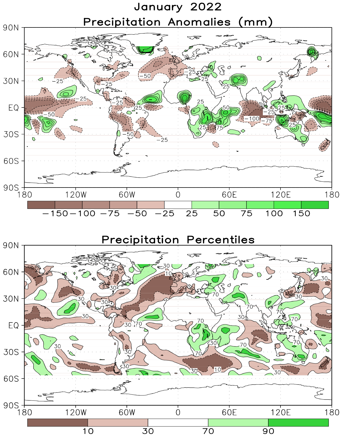
FIGURE E3. Anomalous precipitation (mm, top) and precipitation percentiles based on a Gamma distribution fit to the 1981-2010 base period data (bottom) for JAN 2022. Data are obtained from a merge of raingauge observations and satellite-derived precipitation estimates (Janowiak and Xie 1999, J. Climate , 12 , 3335-3342). Contours are drawn at 200, 100, 50, 25, -25, -50, -100, and -200 mm in top panel. Percentiles are not plotted in regions where mean monthly precipitation is <5mm/month.
