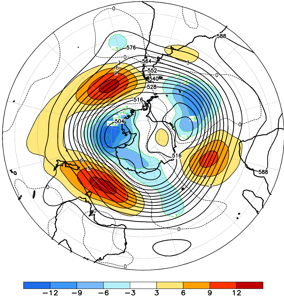
FIGURE E15. Southern Hemisphere mean and anomalous 500-hPa geopotential height (CDAS/Reanalysis) for JAN 2022. Mean heights are denoted by solid contours drawn at an interval of 6 dam. Anomaly contour interval is 3 dam with values less (greater) than -3 dam (3 dam) indicated by dark (light) shading. Anomalies are calculated as departures from the 1991-2020 base period monthly means.
