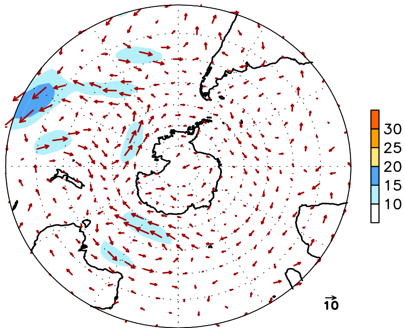
FIGURE E16. Southern Hemisphere mean (left) and anomalous (right) 300-hPa vector wind (CDAS/Reanalysis) for JAN 2021. Mean (anomaly) isotach contour interval is 10 (5) ms -1 . Values greater than 30 ms -1 (left) and 10 ms -1 (rights) are shaded. Anomalies are departures from the 1981-2010 base period monthly means.
