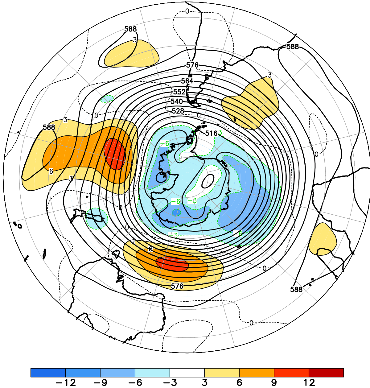
FIGURE E15. Southern Hemisphere mean and anomalous 500-hPa geopotential height (CDAS/Reanalysis) for JAN 2021. Mean heights are denoted by solid contours drawn at an interval of 6 dam. Anomaly contour interval is 3 dam with values less (greater) than -3 dam (3 dam) indicated by dark (light) shading. Anomalies are calculated as departures from the 1981-2010 base period monthly means.
