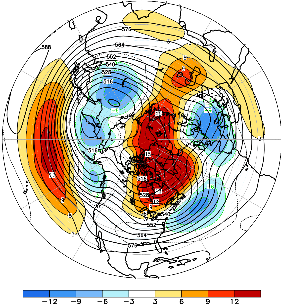
FIGURE E9. Northern Hemisphere mean and anomalous 500-hPa geopotential height (CDAS/Reanalysis) for JAN 2021. Mean heights are denoted by solid contours drawn at an interval of 6 dam. Anomaly contour interval is 3 dam with values less (greater) than -3 dam (3 dam) indicated by dark (light) shading. Anomalies are calculated as departures from the 1981-2010 base period monthly means.
