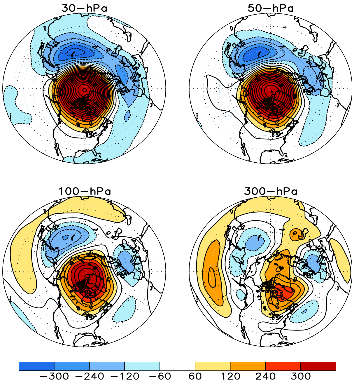
FIGURE S1. Stratospheric height anomalies (m) at selected levels for JAN 2021. Positive values are indicated by solid contours and dark shading. Negative values are indicated by dashed contours and light shading. Contour interval is 60 m. Anomalies are calculated from the 1981-2010 base period means. Winter Hemisphere is shown.
