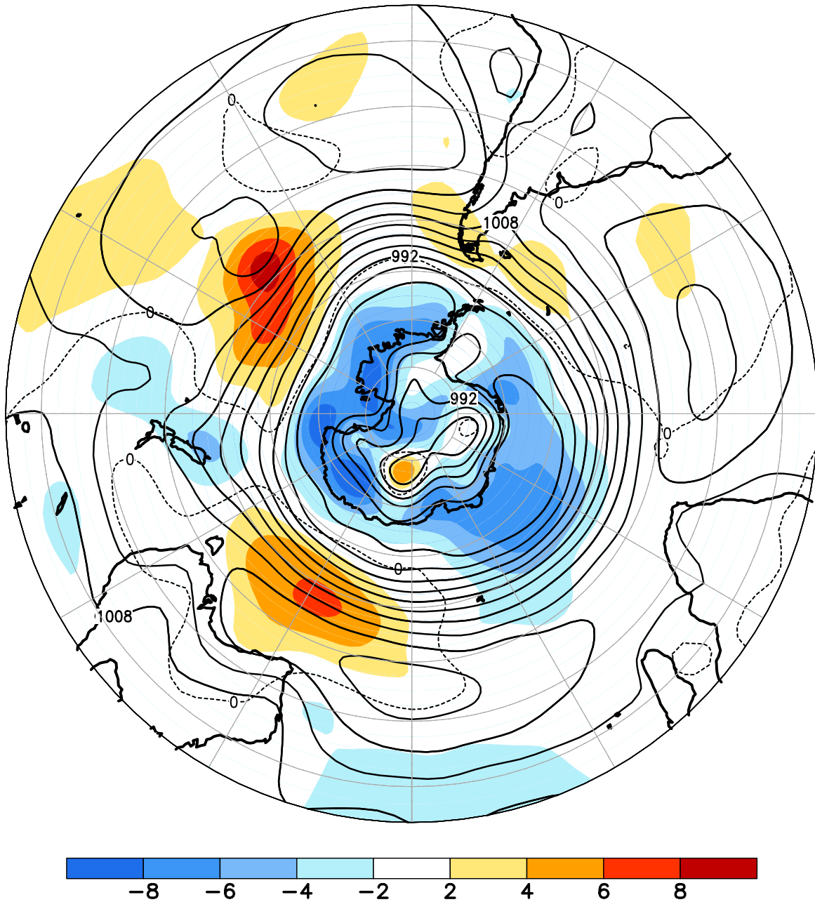
FIGURE E14. Southern Hemisphere mean and anomalous sea level pressure(CDAS/Reanalysis) for JAN 2021. Mean values are denoted by solid contours drawn at an interval of 4 hPa. Anomaly contour interval is 2 hPa with values less (greater) than -2 hPa (2 hPa) indicated by dark (light) shading. Anomalies are calculated as departures from the 1981-2010 base period monthly means.
