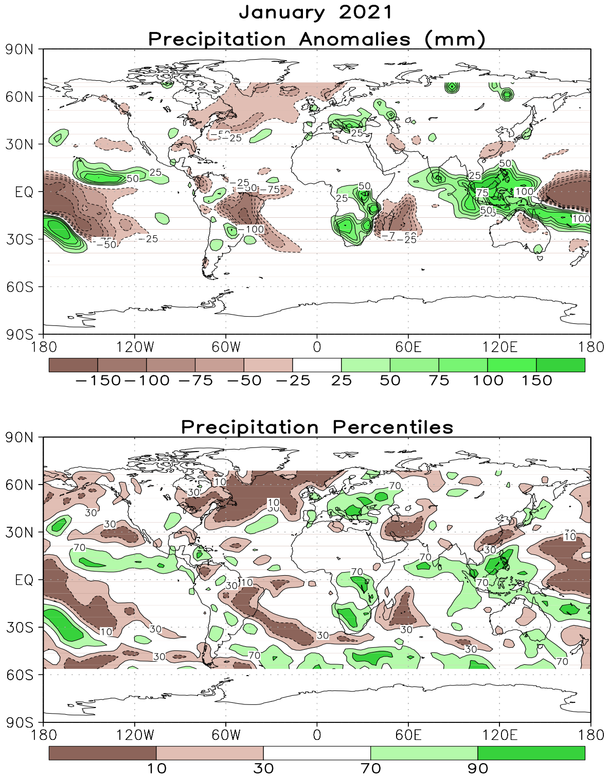
FIGURE E3. Anomalous precipitation (mm, top) and precipitation percentiles based on a Gamma distribution fit to the 1981–2010 base period data (bottom) for JAN 2021. Data are obtained from a merge of raingauge observations and satellite-derived precipitation estimates (Janowiak and Xie 1999, J. Climate , 12 , 3335–3342). Contours are drawn at 200, 100, 50, 25, -25, -50, -100, and -200 mm in top panel. Percentiles are not plotted in regions where mean monthly precipitation is <5mm/month.
