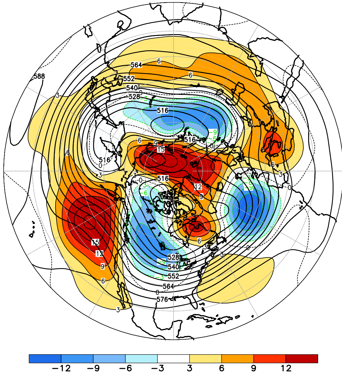
FIGURE E9. Northern Hemisphere mean and anomalous 500-hPa geopotential height (CDAS/Reanalysis) for FEB 2021. Mean heights are denoted by solid contours drawn at an interval of 6 dam. Anomaly contour interval is 3 dam with values less (greater) than -3 dam (3 dam) indicated by dark (light) shading. Anomalies are calculated as departures from the 1981-2010 base period monthly means.
