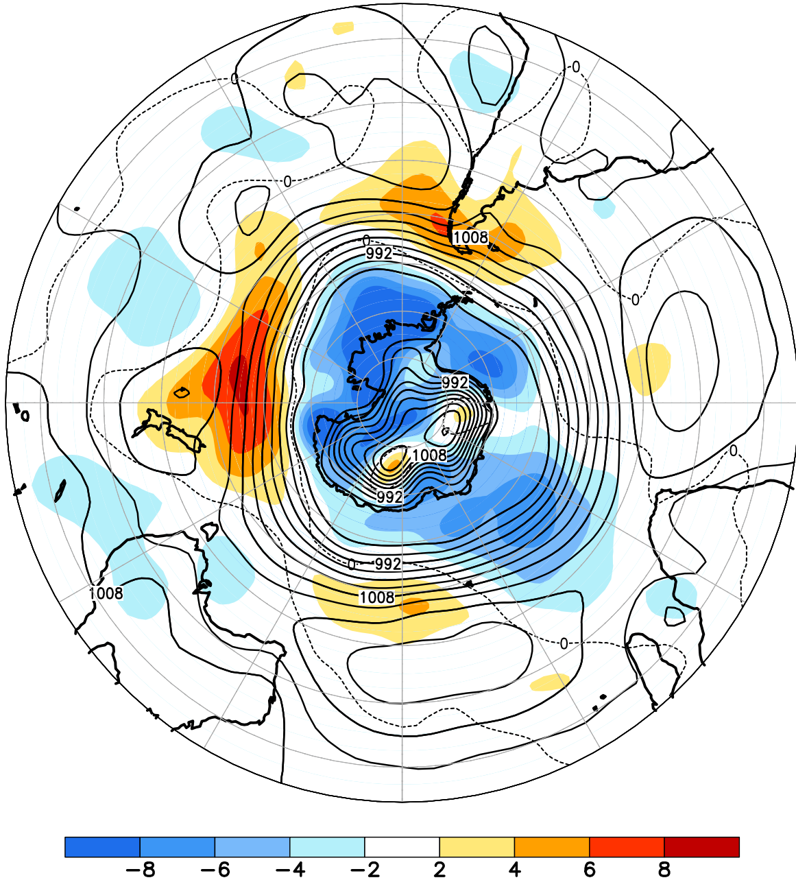
FIGURE E14. Southern Hemisphere mean and anomalous sea level pressure(CDAS/Reanalysis) for FEB 2021. Mean values are denoted by solid contours drawn at an interval of 4 hPa. Anomaly contour interval is 2 hPa with values less (greater) than -2 hPa (2 hPa) indicated by dark (light) shading. Anomalies are calculated as departures from the 1981-2010 base period monthly means.
