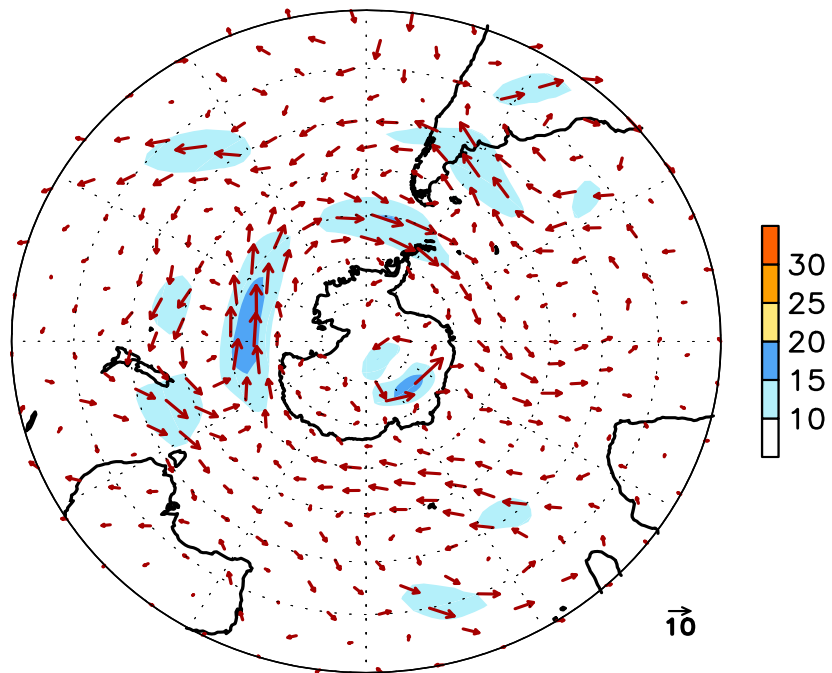
FIGURE E16. Southern Hemisphere mean (left) and anomalous (right) 300-hPa vector wind (CDAS/Reanalysis) for FEB 2021. Mean (anomaly) isotach contour interval is 10 (5) \text{ms}^{-1} . Values greater than 30 \text{ms}^{-1} (left) and 10 \text{ms}^{-1} (rights) are shaded. Anomalies are departures from the 1981-2010 base period monthly means.
