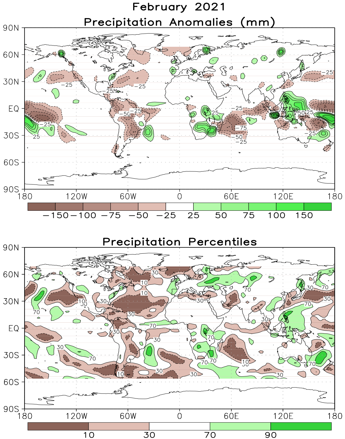
FIGURE E3. Anomalous precipitation (mm, top) and precipitation percentiles based on a Gamma distribution fit to the 1981–2010 base period data (bottom) for FEB 2021. Data are obtained from a merge of raingauge observations and satellite-derived precipitation estimates (Janowiak and Xie 1999, J. Climate , 12 , 3335–3342). Contours are drawn at 200, 100, 50, 25, -25, -50, -100, and -200 mm in top panel. Percentiles are not plotted in regions where mean monthly precipitation is <5mm/month.
