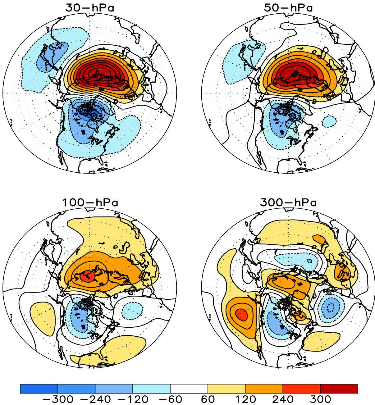
FIGURE S1. Stratospheric height anomalies (m) at selected levels for FEB 2021. Positive values are indicated by solid contours and dark shading. Negative values are indicated by dashed contours and light shading. Contour interval is 60 m. Anomalies are calculated from the 1981-2010 base period means. Winter Hemisphere is shown.
