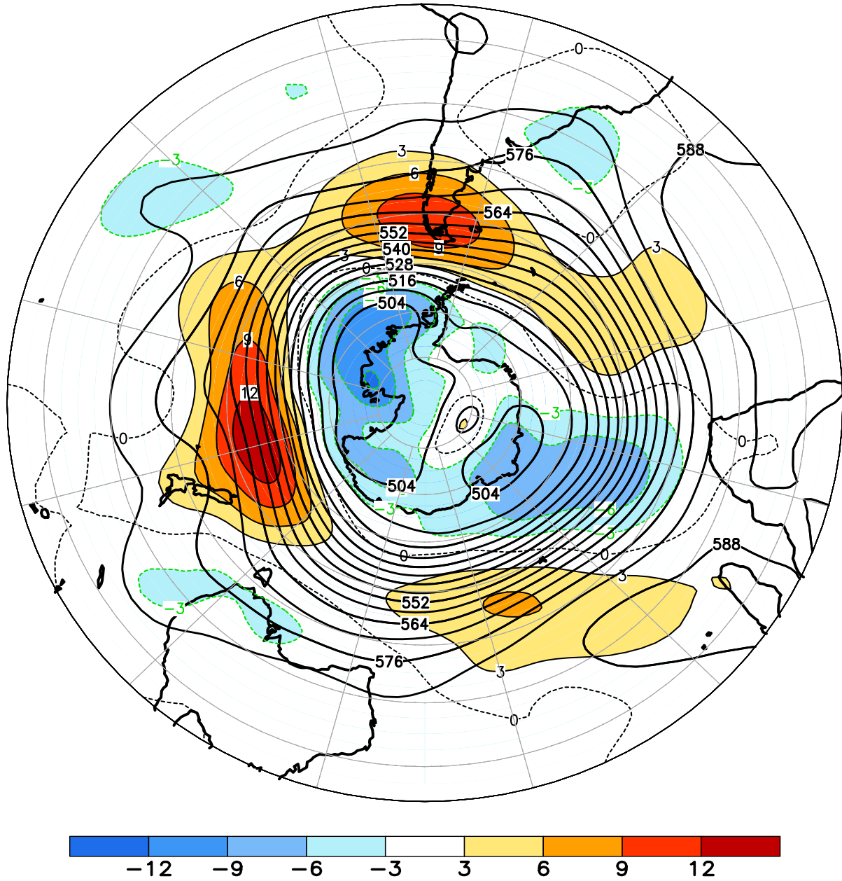
FIGURE E15. Southern Hemisphere mean and anomalous 500-hPa geopotential height (CDAS/Reanalysis) for FEB 2021. Mean heights are denoted by solid contours drawn at an interval of 6 dam. Anomaly contour interval is 3 dam with values less (greater) than -3 dam (3 dam) indicated by dark (light) shading. Anomalies are calculated as departures from the 1981-2010 base period monthly means.
