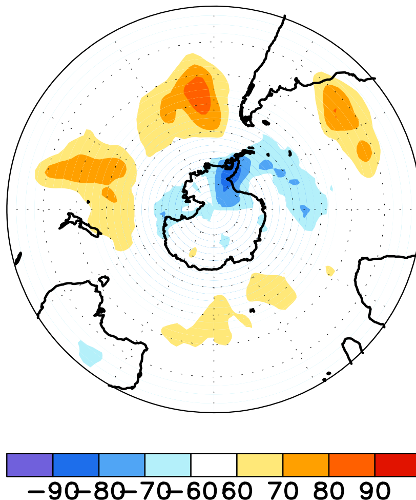
FIGURE E17. Southern Hemisphere percentage of days during FEB 2014 in which 500-hPa height anomalies greater than 15 m (red) and less than -15 m (blue) were observed. Values greater than 70% are shaded and contour in-
