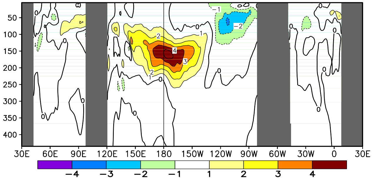
FIGURE T17. Equatorial depth–longitude section of ocean temperature (top) and ocean temperature anomalies (bottom) for FEB 2014. Contour interval is 1°C. Dashed contours in bottom panel indicate negative anomalies. Data are derived from the NCEP’s global ocean data assimilation system version 2 which assimilates oceanic observations into an oceanic GCM (Xue, Y. and Behringer, D.W., 2006: Operational global ocean data assimilation system at NCEP, to be submitted to BAMS). Anomalies are departures from the 1981–2010 base period means.
