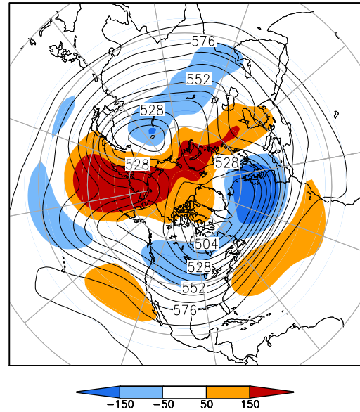
500-hPa Height (dm) & Anomalies (m) (Feb 1–15, 2014)
