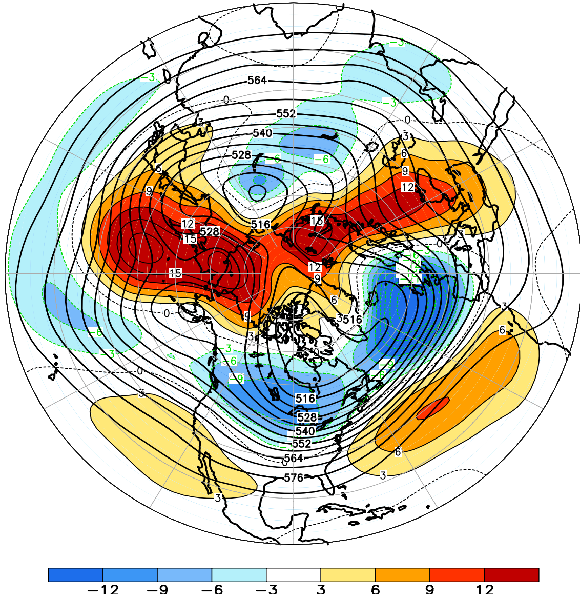
FIGURE E9. Northern Hemisphere mean and anomalous 500-hPa geopotential height (CDAS/Reanalysis) for FEB 2014. Mean heights are denoted by solid contours drawn at an interval of 6 dam. Anomaly contour interval is 3 dam with values less (greater) than -3 dam (3 dam) indicated by dark (light) shading. Anomalies are calculated as departures from the 1981-2010 base period monthly means.
