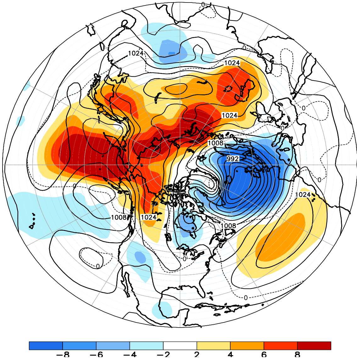
FIGURE E8. Northern Hemisphere mean and anomalous sea level pressure (CDAS/Reanalysis) for FEB 2014. Mean values are denoted by solid contours drawn at an interval of 4 hPa. Anomaly contour interval is 2 hPa with values less (greater) than -2 hPa (2 hPa) indicated by dark (light) shading. Anomalies are calculated as departures from the 1981-2010 base period monthly means.
