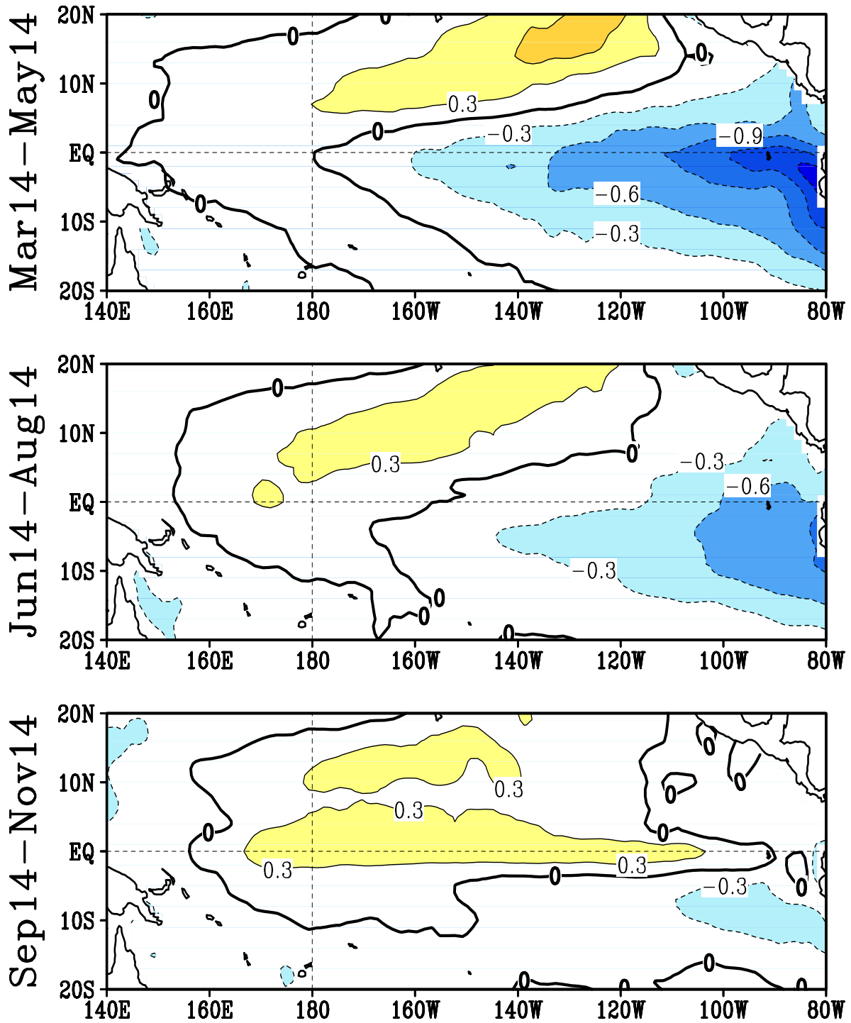
FIGURE F5. Predicted 3-month average sea surface temperature anomalies from the NCEP/CPC Markov model (Xue et al. 2000, J. Climate , 13 , 849-871). The forecast is initiated in FEB 2014 . Contour interval is 0.3C and negative anomalies are indicated by dashed contours. Anomalies are calculated relative to the 1971-2000 climatology.
