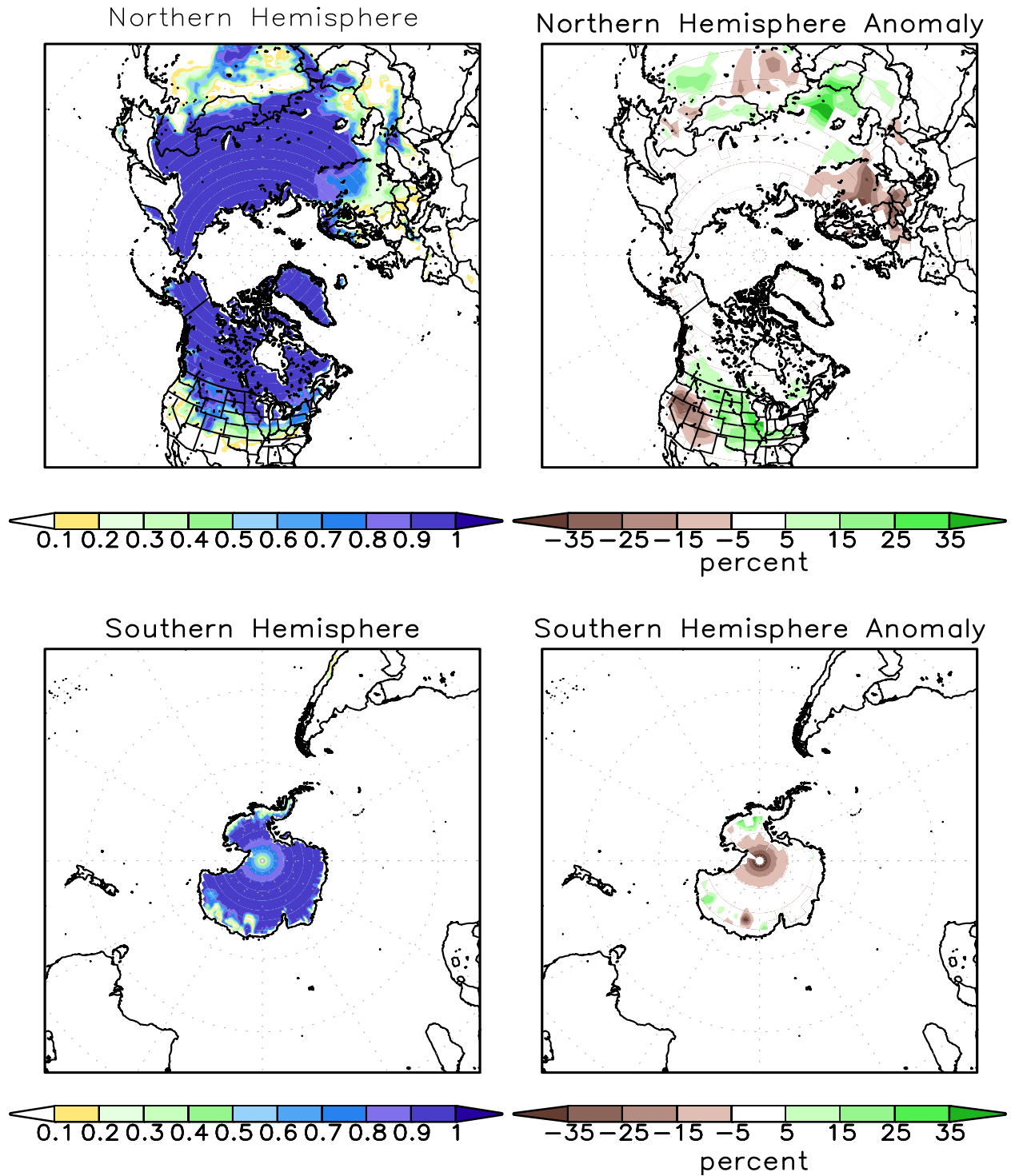
FIGURE A2.2. SSM/I derived snow cover frequency (%) (left) and snow cover anomaly (%) (right) for the month of FEB 2014 based on 1987 - 2010 base period for the Northern Hemisphere (top) and Southern Hemisphere (bottom). It is generated using the algorithm described by Ferraro et. al, 1996, Bull. Amer. Meteor. Soc., vol 77, 891-905.
