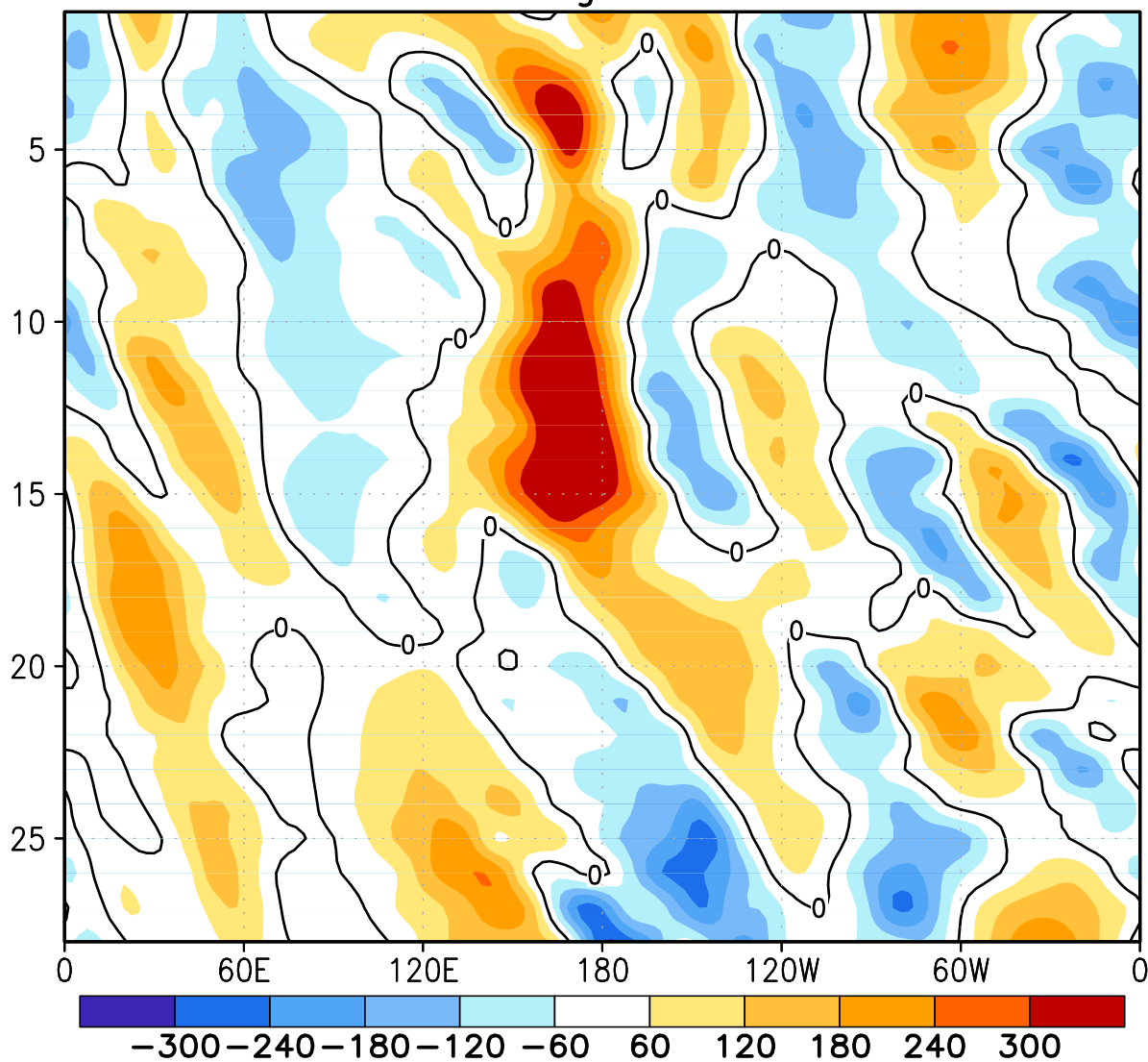
FIGURE E12. Northern Hemisphere: Daily 500-hPa height anomalies for FEB 2014 averaged over the 5° latitude band centered on 40°N. Positive values are indicated by solid contours and dark shading. Negative values are indicated by dashed contours and light shading. Contour interval is 60 m. Anomalies are departures from the 1981-2010 base period daily means.
