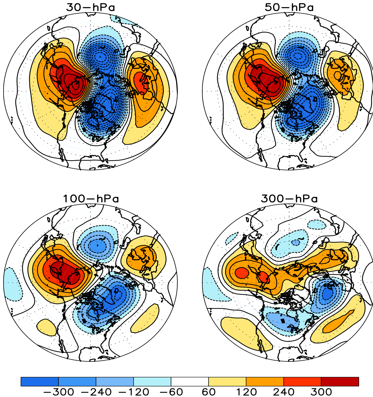
FIGURE S1. Stratospheric height anomalies (m) at selected levels for FEB 2014. Positive values are indicated by solid contours and dark shading. Negative values are indicated by dashed contours and light shading. Contour interval is 60 m. Anomalies are calculated from the 1981-2010 base period means. Winter Hemisphere is shown.
