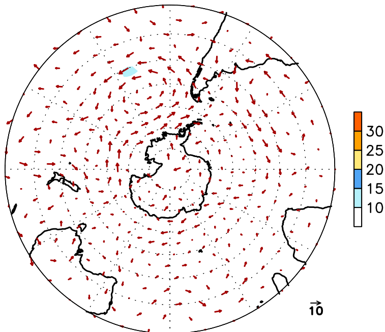
FIGURE E16. Southern Hemisphere mean (left) and anomalous (right) 300-hPa vector wind (CDAS/Reanalysis) for FEB 2014. Mean (anomaly) isotach contour interval is 10 (5) \text{ms}^{-1} . Values greater than 30 \text{ms}^{-1} (left) and 10 \text{ms}^{-1} (rights) are shaded. Anomalies are departures from the 1981-2010 base period monthly means.
