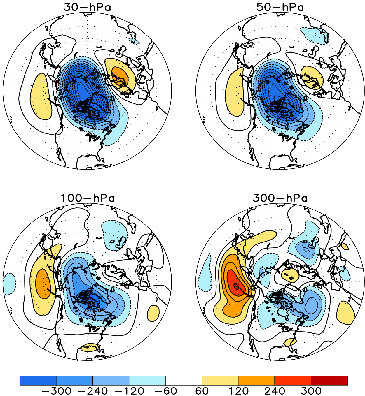
FIGURE S1. Stratospheric height anomalies (m) at selected levels for FEB 2011. Positive values are indicated by solid contours and dark shading. Negative values are indicated by dashed contours and light shading. Contour interval is 60 m. Anomalies are calculated from the 1981-2010 base period means. Winter Hemisphere is shown.
