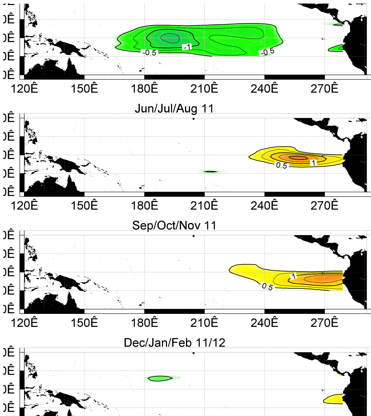
FIGURE F11. SST anomaly forecast for the equatorial Pacific from the Hybrid Coupled Model (HCM) developed by the Scripps Institution of Oceanography and the Max-Plank Institut fuer Meteorologie.
