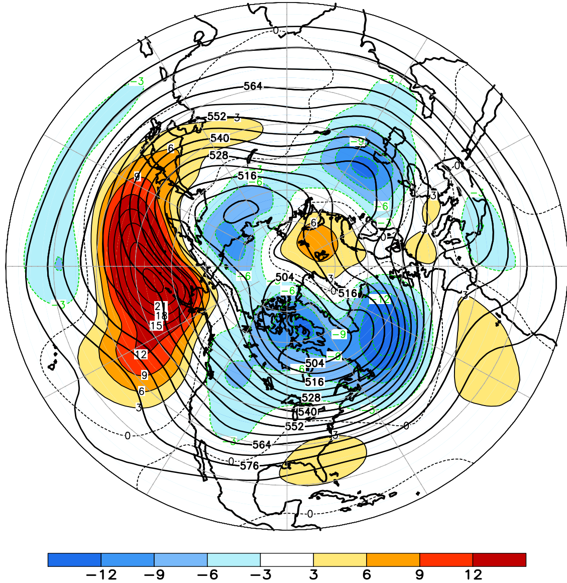
FIGURE E9. Northern Hemisphere mean and anomalous 500-hPa geopotential height (CDAS/Reanalysis) for FEB 2011. Mean heights are denoted by solid contours drawn at an interval of 6 dam. Anomaly contour interval is 3 dam with values less (greater) than -3 dam (3 dam) indicated by dark (light) shading. Anomalies are calculated as departures from the 1981-2010 base period monthly means.
