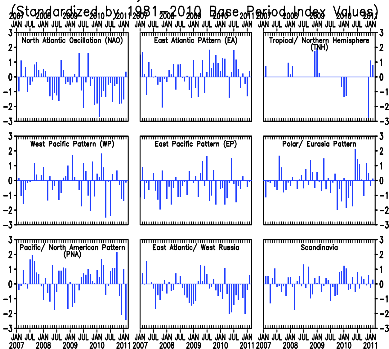
FIGURE E7. Standardized monthly Northern Hemisphere teleconnection indices. The teleconnection patterns are calculated from a Rotated Principal Component Analysis (RPCA) applied to monthly standardized 500-hPa height anomalies during the 1981–2010 base period. To obtain these patterns, ten leading unrotated modes are first calculated for each calendar month by using the monthly height anomaly fields for the three-month period centered on that month: [i.e., The July modes are calculated from the June, July, and August standardized monthly anomalies]. A Varimax spatial rotation of the ten leading unrotated modes for each calendar month results in 120 rotated modes (12 months x 10 modes per month) that yield ten primary teleconnection patterns. The teleconnection indices are calculated by first projecting the standardized monthly anomalies onto the teleconnection patterns corresponding to that month (eight or nine teleconnection patterns are seen in each calendar month). The indices are then solved for simultaneously using a Least-Squares approach. In this approach, the indices are the solution to the Least-Squares system of equations which explains the maximum spatial structure of the observed height anomaly field during the month. The indices are then standardized for each pattern and calendar month independently. No index value exists when the teleconnection pattern does not appear as one of the ten leading rotated EOF's valid for that month.
