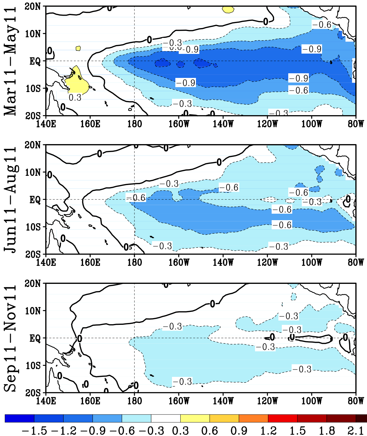
FIGURE F5. Predicted 3-month average sea surface temperature anomalies from the NCEP/CPC Markov model (Xue et al. 2000, J. Climate , 13 , 849-871). The forecast is initiated in FEB 2011 . Contour interval is 0.3C and negative anomalies are indicated by dashed contours. Anomalies are calculated relative to the 1971-2000 climatology.
