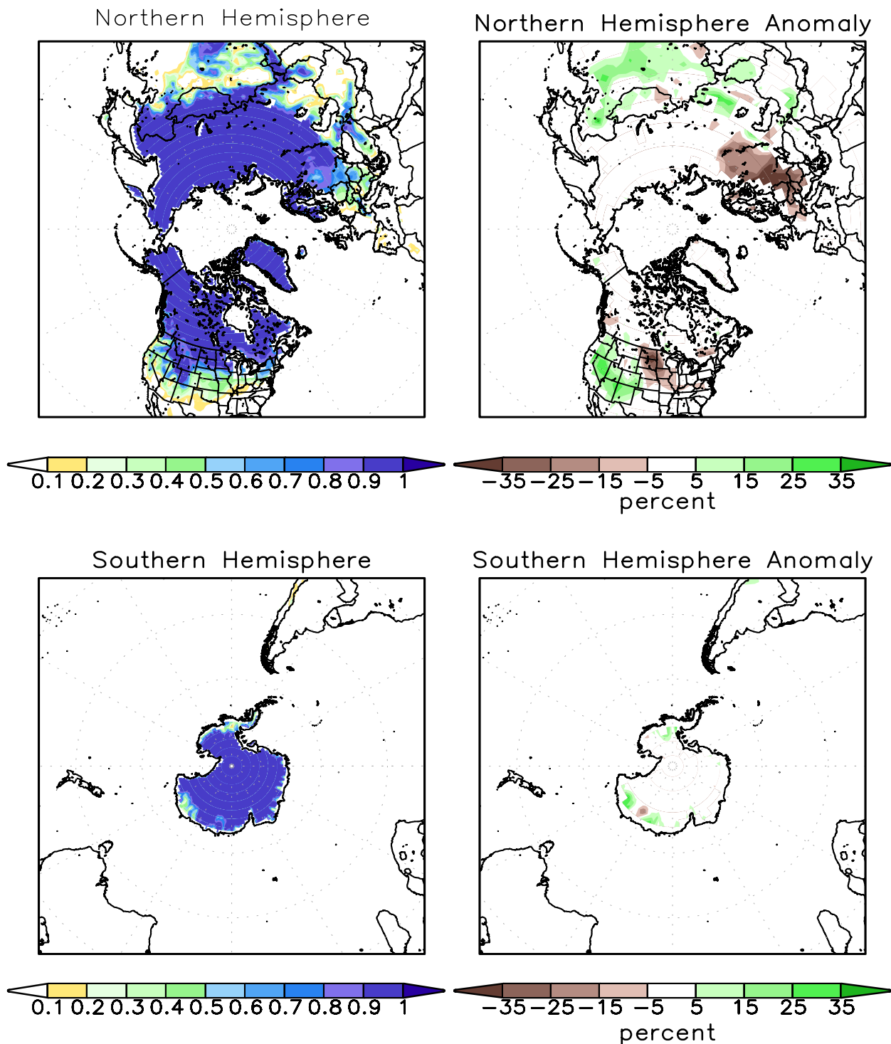
FIGURE A2.2. SSM/I derived snow cover frequency (%) (left) and snow cover anomaly (%) (right) for the month of FEB 2011 based on 1987 - 2010 base period for the Northern Hemisphere (top) and Southern Hemisphere (bottom). It is generated using the algorithm described by Ferraro et. al, 1996, Bull. Amer. Meteor. Soc., vol 77, 891-905.
