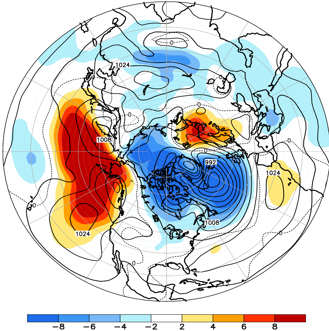
FIGURE E8. Northern Hemisphere mean and anomalous sea level pressure (CDAS/Reanalysis) for FEB 2011. Mean values are denoted by solid contours drawn at an interval of 4 hPa. Anomaly contour interval is 2 hPa with values less (greater) than -2 hPa (2 hPa) indicated by dark (light) shading. Anomalies are calculated as departures from the 1981-2010 base period monthly means.
