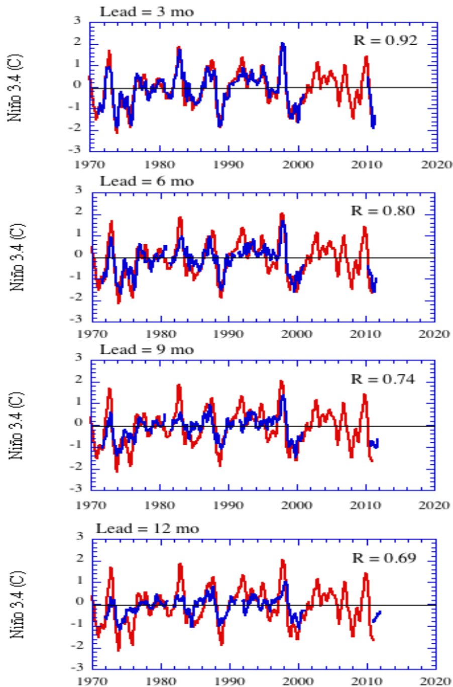
FIGURE F10. Predictions of Niño 3.4 SSTA (blue solid line) and verification (solid red line). The Niño3.4 Index was calculated in the area 6N-6S, 170W-120W. The 1980-2010 climatology was subtracted from ERSST data between 1950 and 2010, after which they were projected onto 20 EOFs containing 90% of the variance. Significant 1950-2010 trends were subtracted from the corresponding PCs, the forecast was made on the detrended anomalies, after which the trend was added to the forecast. Cross-validated forecasts for 2001-2010 are not shown because that decade was necessary to get a good estimate of the trend, thus precluding legitimate cross-validation. Cross-validated forecasts shown before 2001 use trends estimated using data outside the verification period.
