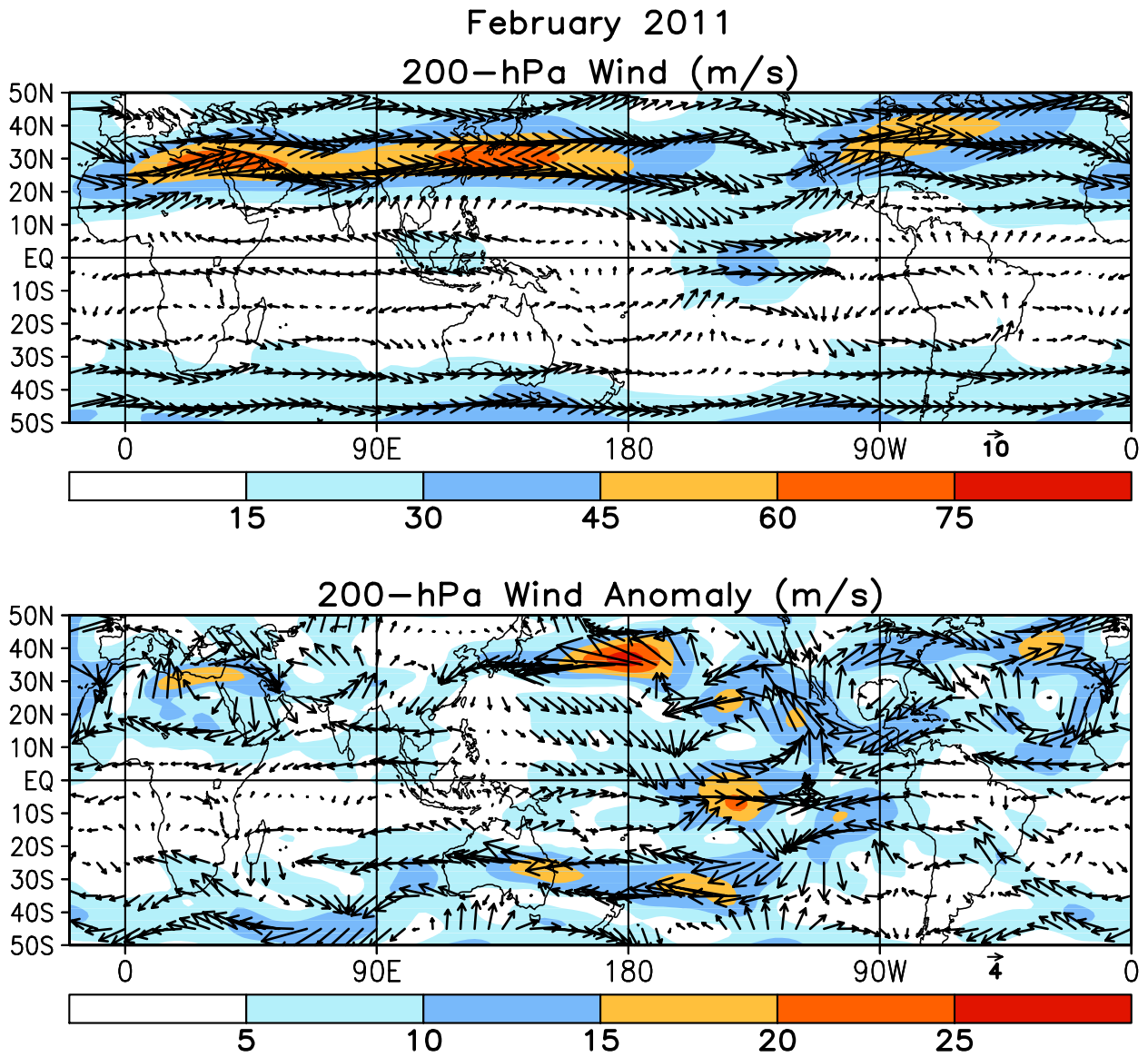
FIGURE T21. Mean (top) and anomalous (bottom) 200-hPa vector wind (CDAS/Reanalysis) for FEB 2011. Contour interval for isotachs is 15 \text{ ms}^{-1} (top) and 5 \text{ ms}^{-1} (bottom). Anomalies are departures from 1981-2010 base period monthly means.
