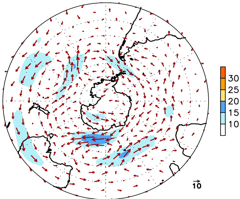
FIGURE E16. Southern Hemisphere mean (left) and anomalous (right) 300-hPa vector wind (CDAS/Reanalysis) for FEB 2011. Mean (anomaly) isotach contour interval is 10 (5) \text{ms}^{-1} . Values greater than 30 \text{ms}^{-1} (left) and 10 \text{ms}^{-1} (rights) are shaded. Anomalies are departures from the 1981-2010 base period monthly means.
