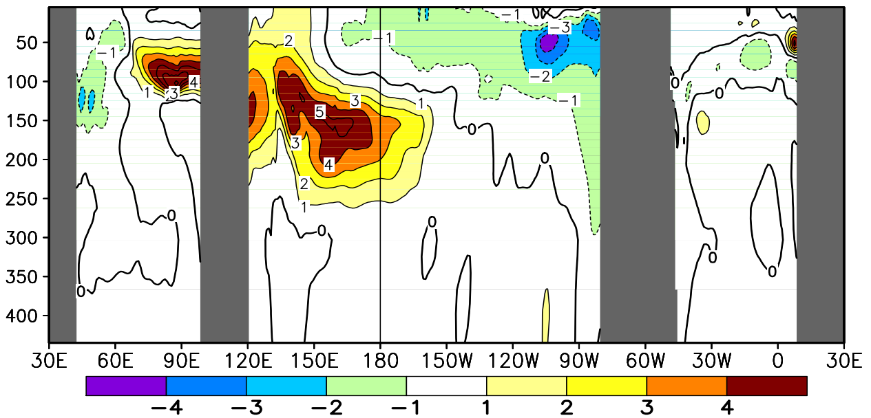
FIGURE T17. Equatorial depth–longitude section of ocean temperature (top) and ocean temperature anomalies (bottom) for FEB 2011. Contour interval is 1°C. Dashed contours in bottom panel indicate negative anomalies. Data are derived from the NCEP’s global ocean data assimilation system version 2 which assimilates oceanic observations into an oceanic GCM (Xue, Y. and Behringer, D.W., 2006: Operational global ocean data assimilation system at NCEP, to be submitted to BAMS). Anomalies are departures from the 1981–2010 base period means.
