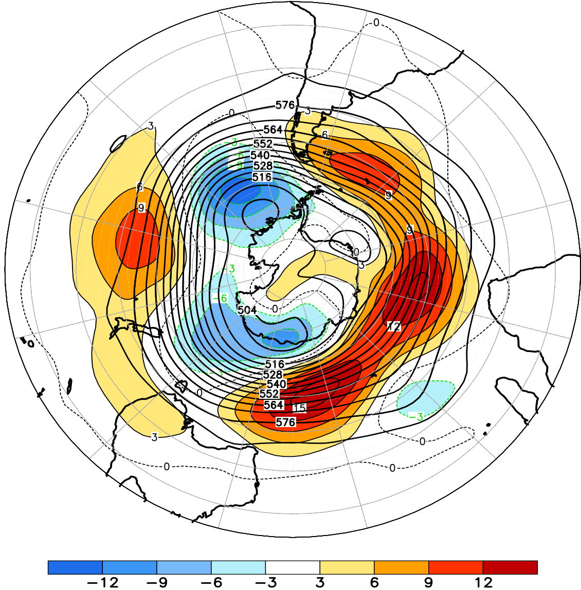
FIGURE E15. Southern Hemisphere mean and anomalous 500-hPa geopotential height (CDAS/Reanalysis) for FEB 2011. Mean heights are denoted by solid contours drawn at an interval of 6 dam. Anomaly contour interval is 3 dam with values less (greater) than -3 dam (3 dam) indicated by dark (light) shading. Anomalies are calculated as departures from the 1981-2010 base period monthly means.
