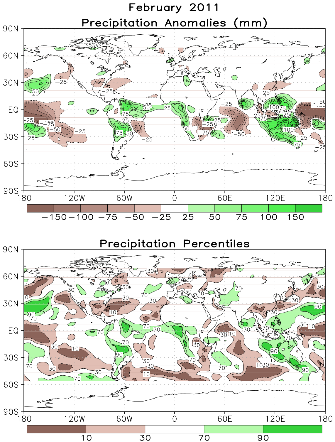
FIGURE E3. Anomalous precipitation (mm, top) and precipitation percentiles based on a Gamma distribution fit to the 1981–2010 base period data (bottom) for FEB 2011. Data are obtained from a merge of raingauge observations and satellite-derived precipitation estimates (Janowiak and Xie 1999, J. Climate , 12 , 3335–3342). Contours are drawn at 200, 100, 50, 25, -25, -50, -100, and -200 mm in top panel. Percentiles are not plotted in regions where mean monthly precipitation is <5mm/month.
