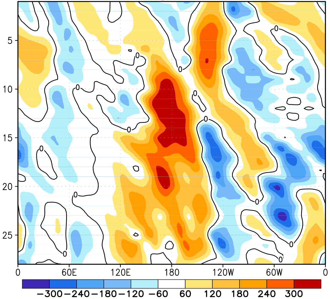
FIGURE E12. Northern Hemisphere: Daily 500-hPa height anomalies for FEB 2011 averaged over the 5° latitude band centered on 40°N. Positive values are indicated by solid contours and dark shading. Negative values are indicated by dashed contours and light shading. Contour interval is 60 m. Anomalies are departures from the 1981-2010 base period daily means.
