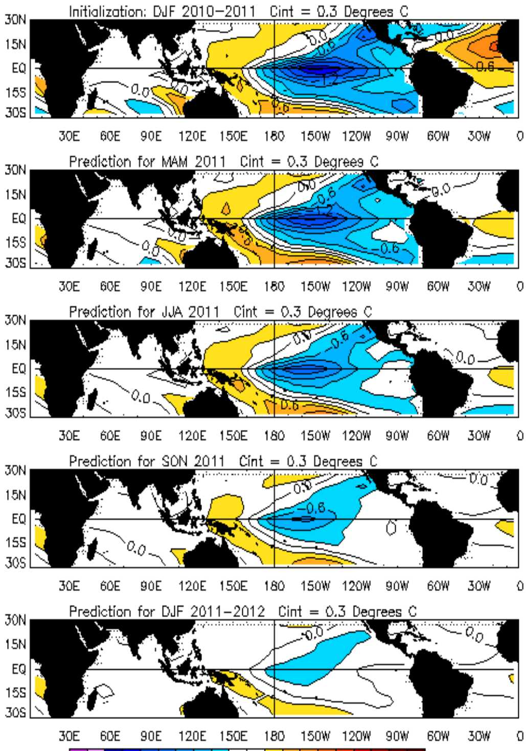
FIGURE F9. Forecast of tropical SST anomalies from the Linear Inverse Modeling technique of Penland and Magorian (1993: J. Climate , 6, 1067-1076). The contour interval is 0.3C. Anomalies are calculated relative to the 1981-2010 climatology and are projected onto 20 leading EOFs.
