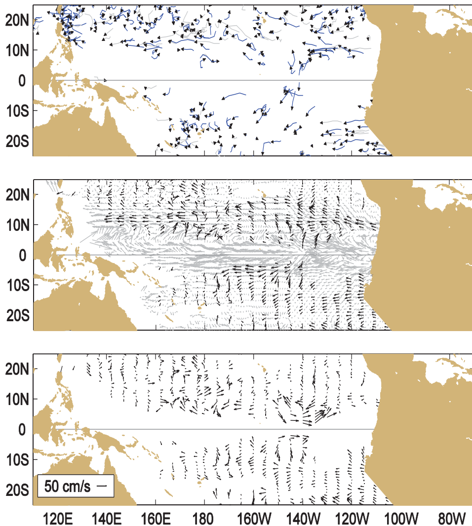
Figure A1.1 Top: Movements of drifting buoys in the tropical Pacific Ocean during Feb 2011. The linear segments of each trajectory represent a one week displacement. Trajectories of buoys which have lost their subsurface drogues are gray; those with drogues are black.
