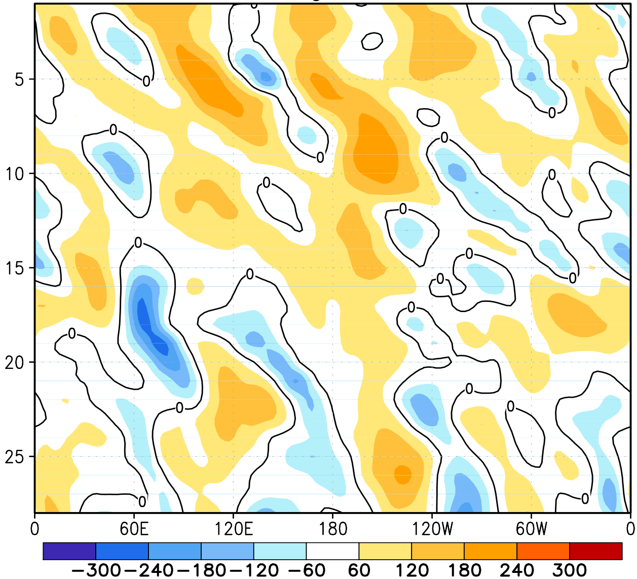
FIGURE E18. Southern Hemisphere: Daily 500-hPa height anomalies for FEB 2011 averaged over the 5° latitude band centered on 40°S. Positive values are indicated by solid contours and dark shading. Negative values are indicated by dashed contours and light shading. Contour interval is 60 m. Anomalies are departures from the 1981-2010 base period daily means.
