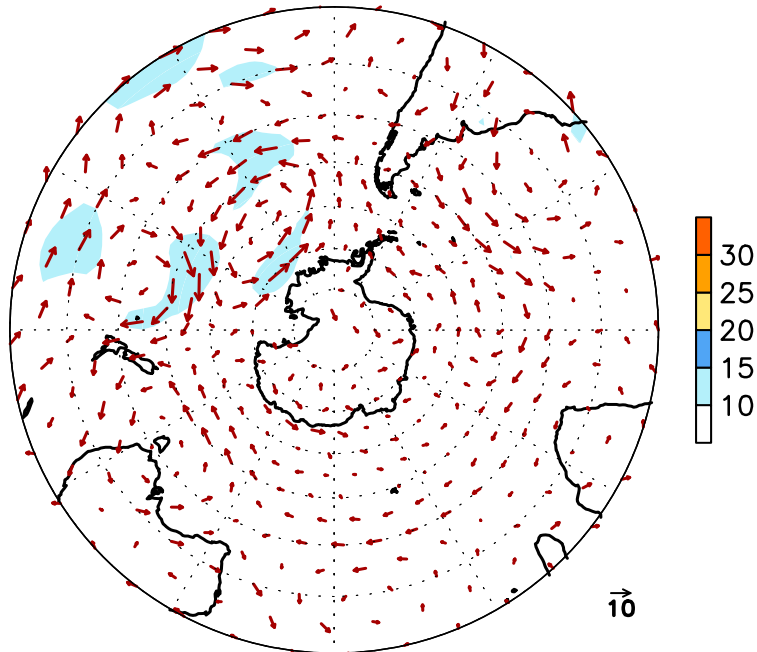
FIGURE E16. Southern Hemisphere mean (left) and anomalous (right) 300-hPa vector wind (CDAS/Reanalysis) for DEC 2015. Mean (anomaly) isotach contour interval is 10 (5) \text{ms}^{-1} . Values greater than 30 \text{ms}^{-1} (left) and 10 \text{ms}^{-1} (rights) are shaded. Anomalies are departures from the 1981-2010 base period monthly means.
