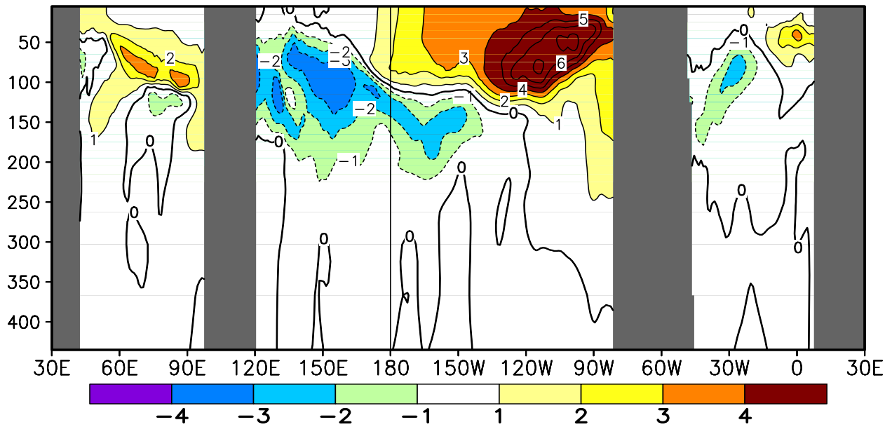
FIGURE T17. Equatorial depth–longitude section of ocean temperature (top) and ocean temperature anomalies (bottom) for DEC 2015. Contour interval is 1°C. Dashed contours in bottom panel indicate negative anomalies. Data are derived from the NCEP’s global ocean data assimilation system version 2 which assimilates oceanic observations into an oceanic GCM (Xue, Y. and Behringer, D.W., 2006: Operational global ocean data assimilation system at NCEP, to be submitted to BAMS). Anomalies are departures from the 1981–2010 base period means.
