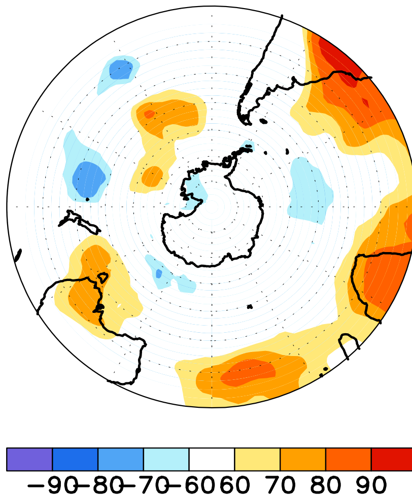
FIGURE E17. Southern Hemisphere percentage of days during DEC 2015 in which 500-hPa height anomalies greater than 15 m (red) and less than -15 m (blue) were observed. Values greater than 70% are shaded and contour in-
