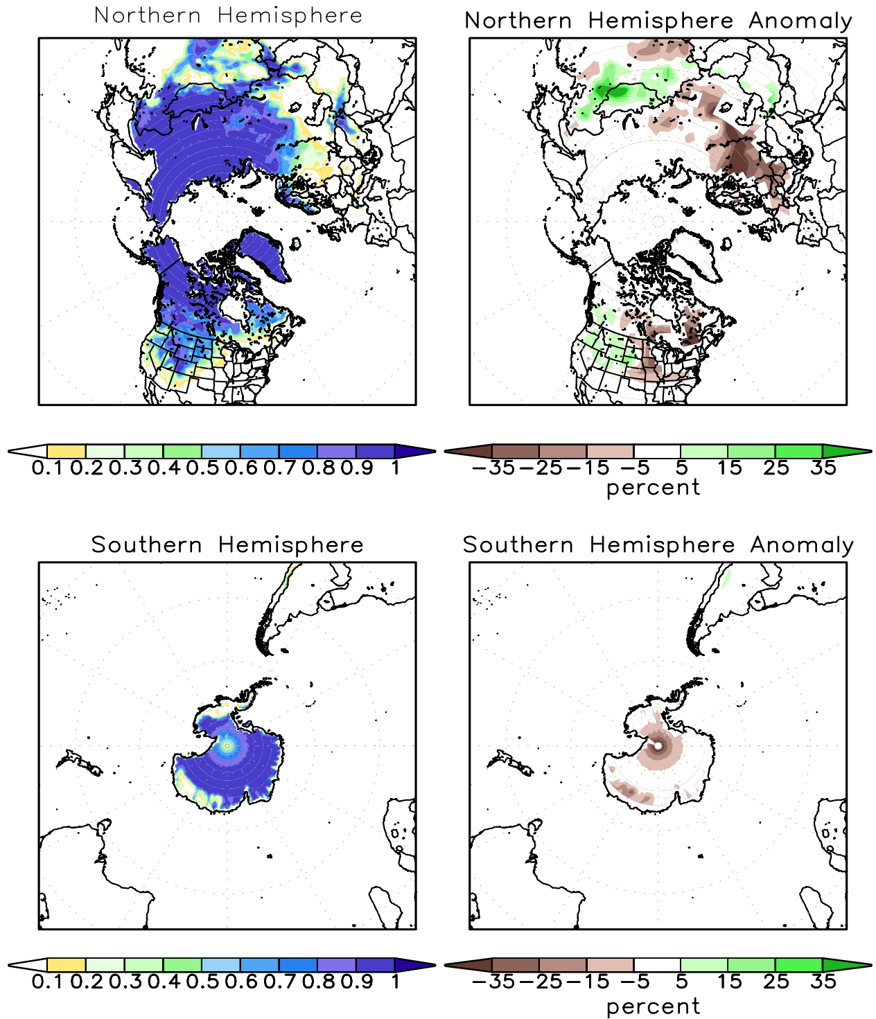
FIGURE A2.2. SSM/I derived snow cover frequency (%) (left) and snow cover anomaly (%) (right) for the month of DEC 2015 based on 1987 - 2010 base period for the Northern Hemisphere (top) and Southern Hemisphere (bottom). It is generated using the algorithm described by Ferraro et. al, 1996, Bull. Amer. Meteor. Soc., vol 77, 891-905.
