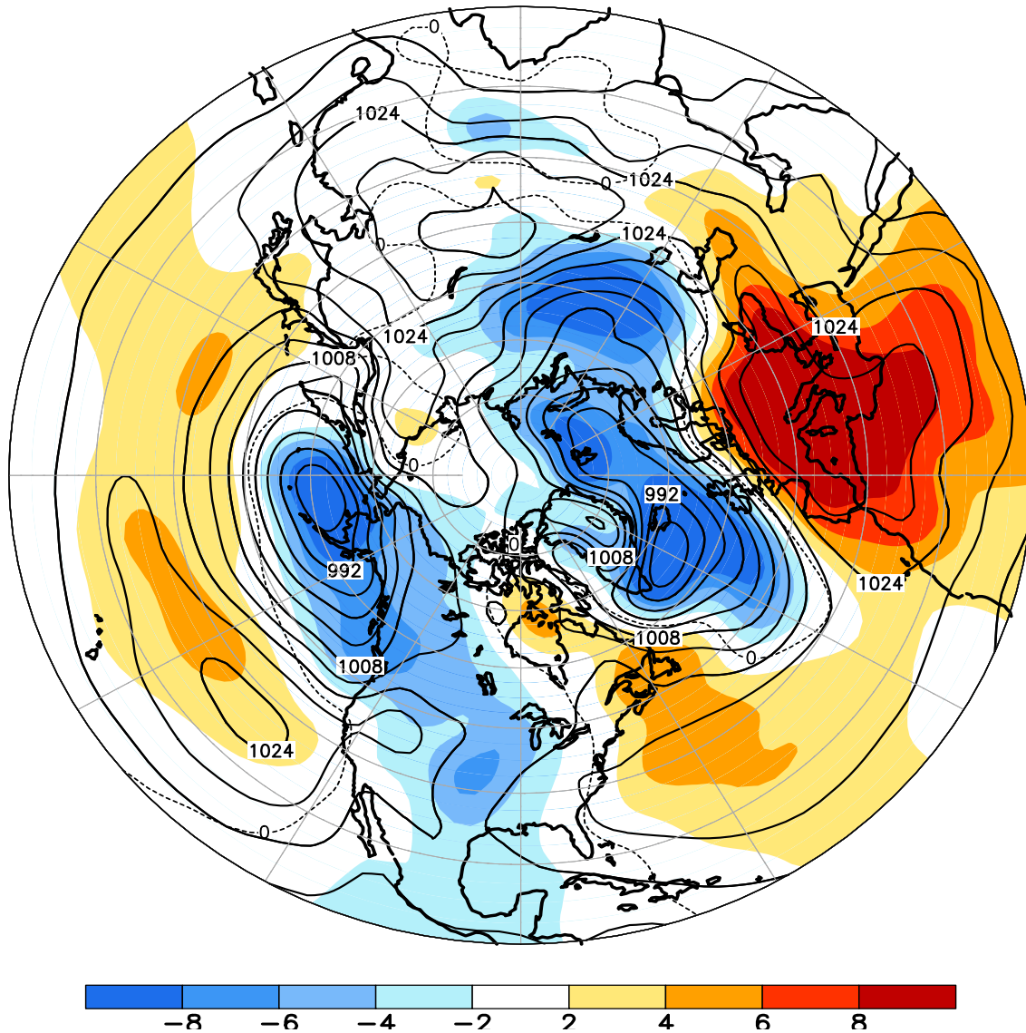
FIGURE E8. Northern Hemisphere mean and anomalous sea level pressure (CDAS/Reanalysis) for DEC 2015. Mean values are denoted by solid contours drawn at an interval of 4 hPa. Anomaly contour interval is 2 hPa with values less (greater) than -2 hPa (2 hPa) indicated by dark (light) shading. Anomalies are calculated as departures from the 1981-2010 base period monthly means.
