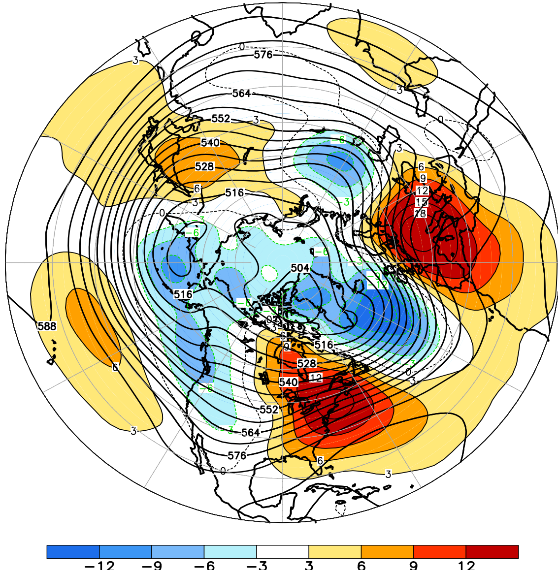
FIGURE E9. Northern Hemisphere mean and anomalous 500-hPa geopotential height (CDAS/Reanalysis) for DEC 2015. Mean heights are denoted by solid contours drawn at an interval of 6 dam. Anomaly contour interval is 3 dam with values less (greater) than -3 dam (3 dam) indicated by dark (light) shading. Anomalies are calculated as departures from the 1981-2010 base period monthly means.
