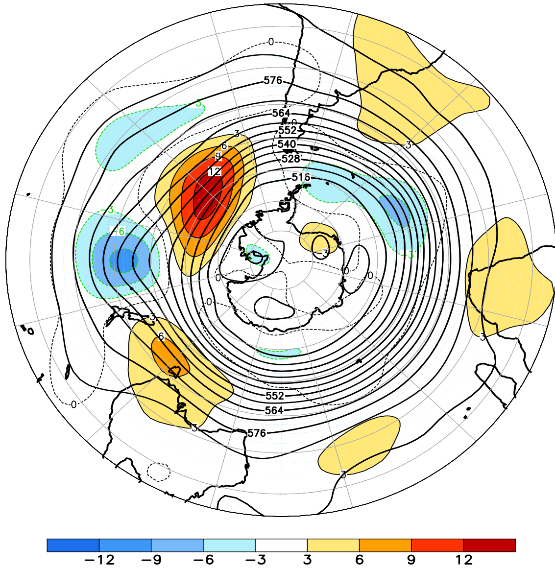
FIGURE E15. Southern Hemisphere mean and anomalous 500-hPa geopotential height (CDAS/Reanalysis) for DEC 2015. Mean heights are denoted by solid contours drawn at an interval of 6 dam. Anomaly contour interval is 3 dam with values less (greater) than -3 dam (3 dam) indicated by dark (light) shading. Anomalies are calculated as departures from the 1981-2010 base period monthly means.
