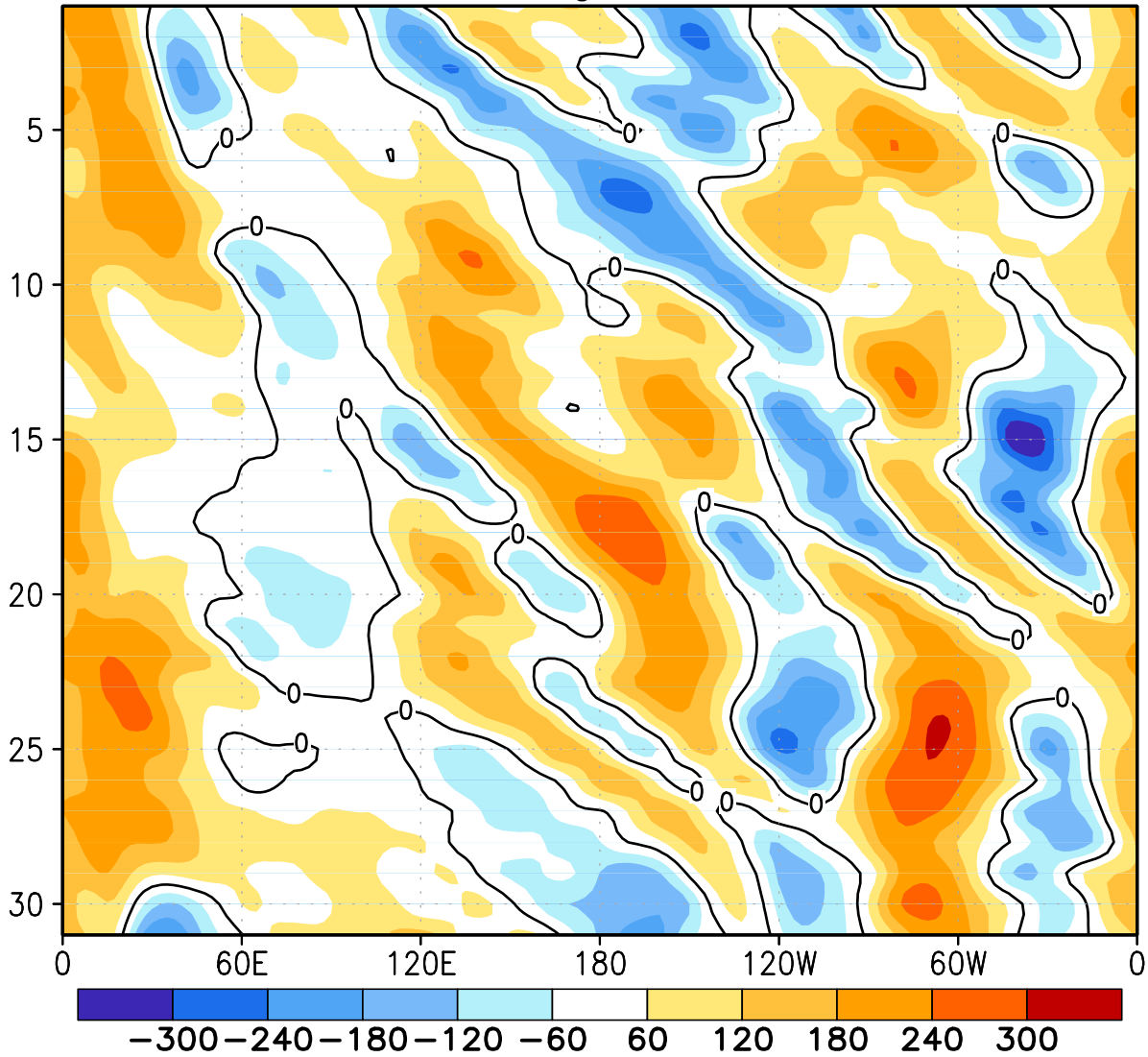
FIGURE E12. Northern Hemisphere: Daily 500-hPa height anomalies for DEC 2015 averaged over the 5° latitude band centered on 40°N. Positive values are indicated by solid contours and dark shading. Negative values are indicated by dashed contours and light shading. Contour interval is 60 m. Anomalies are departures from the 1981-2010 base period daily means.
