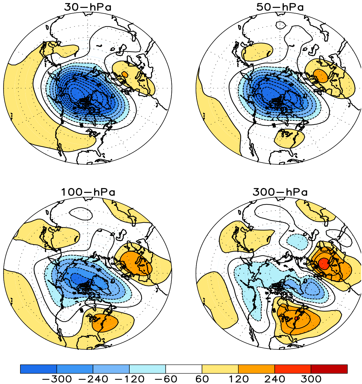
FIGURE S1. Stratospheric height anomalies (m) at selected levels for DEC 2015. Positive values are indicated by solid contours and dark shading. Negative values are indicated by dashed contours and light shading. Contour interval is 60 m. Anomalies are calculated from the 1981-2010 base period means. Winter Hemisphere is shown.
