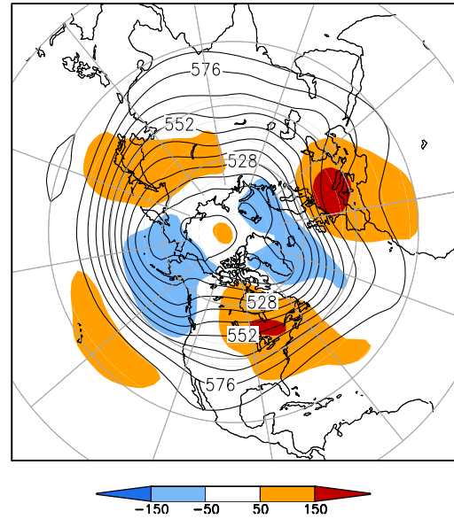
500-hPa Height (dm) & Anomalies (m) (Dec 1–15, 2015)
