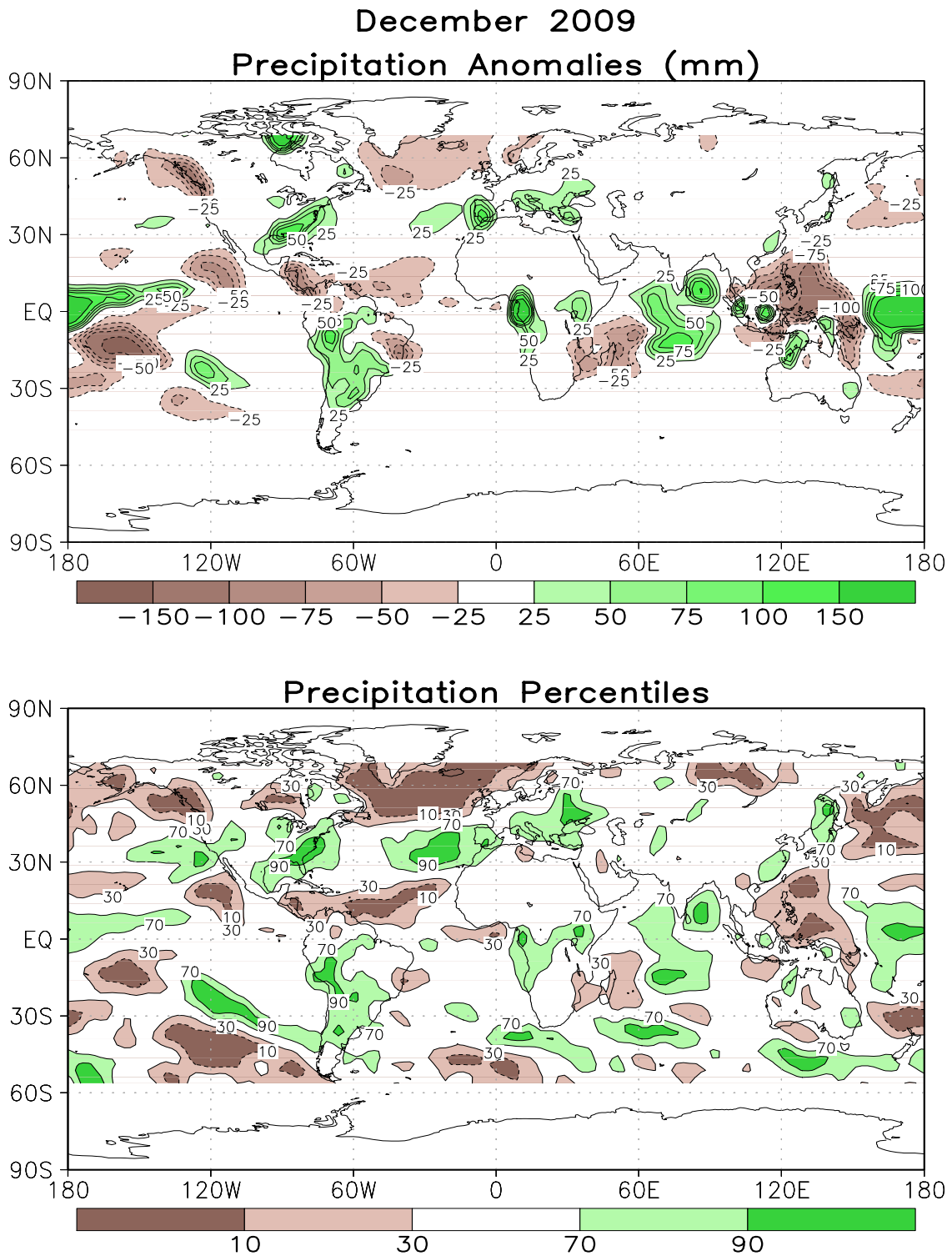
FIGURE E3. Anomalous precipitation (mm, top) and precipitation percentiles based on a Gamma distribution fit to the 1979–2000 base period data (bottom) for DEC 2009. Data are obtained from a merge of raingauge observations and satellite-derived precipitation estimates (Janowiak and Xie 1999, J. Climate , 12 , 3335–3342). Contours are drawn at 200, 100, 50, 25, -25, -50, -100, and -200 mm in top panel. Percentiles are not plotted in regions where mean monthly precipitation is <5mm/month.
