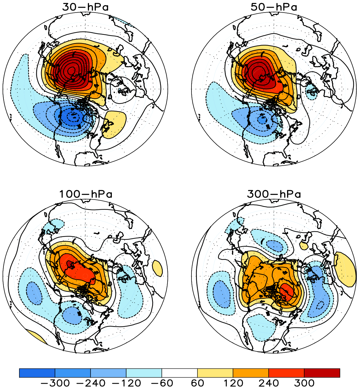
FIGURE S1. Stratospheric height anomalies (m) at selected levels for DEC 2009. Positive values are indicated by solid contours and dark shading. Negative values are indicated by dashed contours and light shading. Contour interval is 60 m. Anomalies are calculated from the 1979–95 base period means. Winter Hemisphere is shown.
