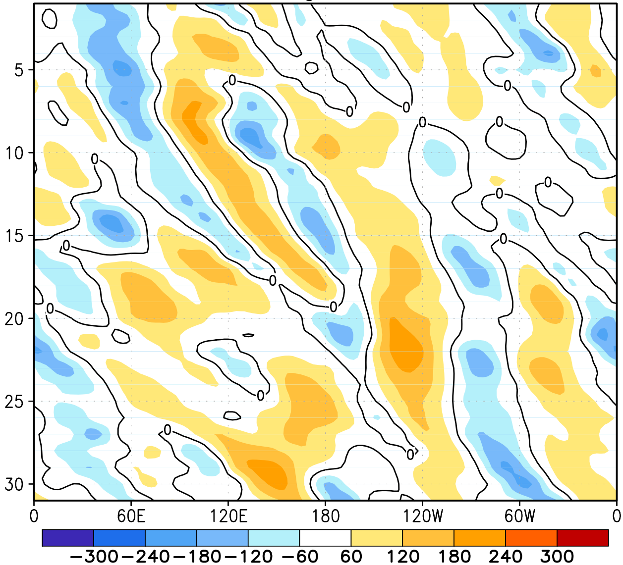
FIGURE E18. Southern Hemisphere: Daily 500-hPa height anomalies for DEC 2009 averaged over the 5° latitude band centered on 40°S. Positive values are indicated by solid contours and dark shading. Negative values are indicated by dashed contours and light shading. Contour interval is 60 m. Anomalies are departures from the 1979-95 base period daily means.
