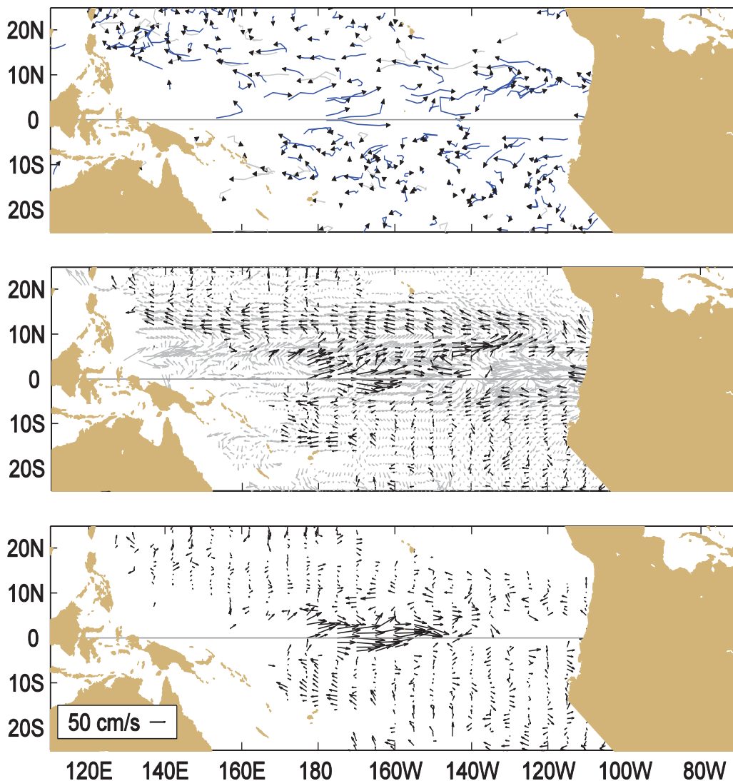
Figure A1.1 Top: Movements of drifting buoys in the tropical Pacific Ocean during December 2009. The linear segments of each trajectory represent a one week displacement. Trajectories of buoys which have lost their subsurface drogues are gray; those with drogues are black.
