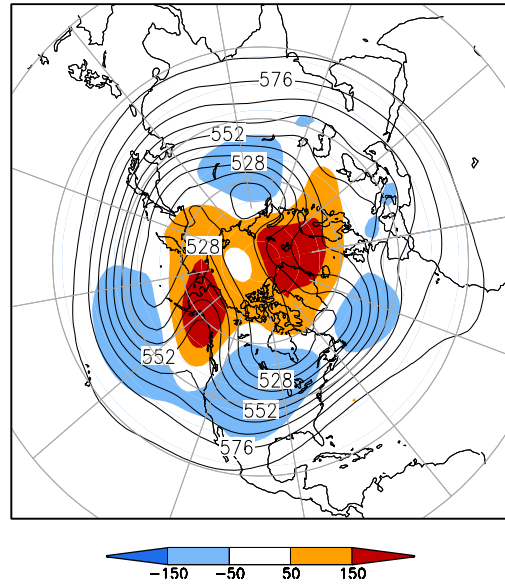
500-hPa Height (dm) & Anomalies (m) (Dec 1–15, 2009)
