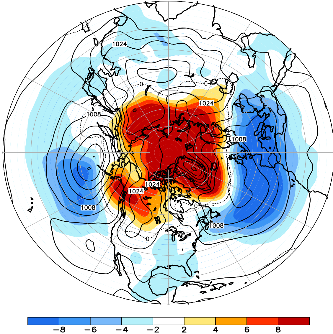
FIGURE E8. Northern Hemisphere mean and anomalous sea level pressure (CDAS/Reanalysis) for DEC 2009. Mean values are denoted by solid contours drawn at an interval of 4 hPa. Anomaly contour interval is 2 hPa with values less (greater) than -2 hPa (2 hPa) indicated by dark (light) shading. Anomalies are calculated as departures from the 1979-95 base period monthly means.
