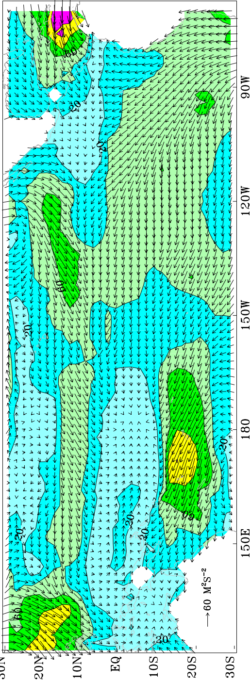
Near-real-time Objective FSU Pseudo-stress Magnitude and Vectors (10m) December 2009
