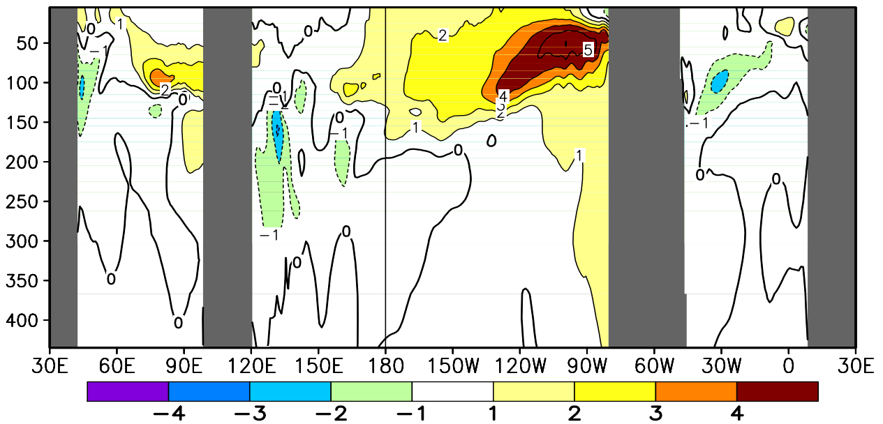
FIGURE T17. Equatorial depth–longitude section of ocean temperature (top) and ocean temperature anomalies (bottom) for DEC 2009. Contour interval is 1°C. Dashed contours in bottom panel indicate negative anomalies. Data are derived from the NCEP’s global ocean data assimilation system version 2 which assimilates oceanic observations into an oceanic GCM (Xue, Y. and Behringer, D.W., 2006: Operational global ocean data assimilation system at NCEP, to be submitted to BAMS). Anomalies are departures from the 1982–2004 base period means.
