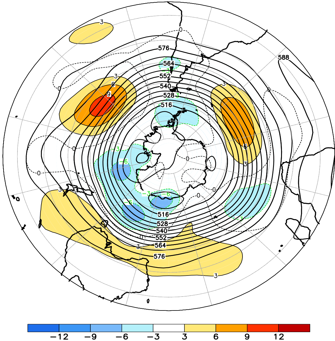
FIGURE E15. Southern Hemisphere mean and anomalous 500-hPa geopotential height (CDAS/Reanalysis) for DEC 2009. Mean heights are denoted by solid contours drawn at an interval of 6 dam. Anomaly contour interval is 3 dam with values less (greater) than -3 dam (3 dam) indicated by dark (light) shading. Anomalies are calculated as departures from the 1979-95 base period monthly means.
