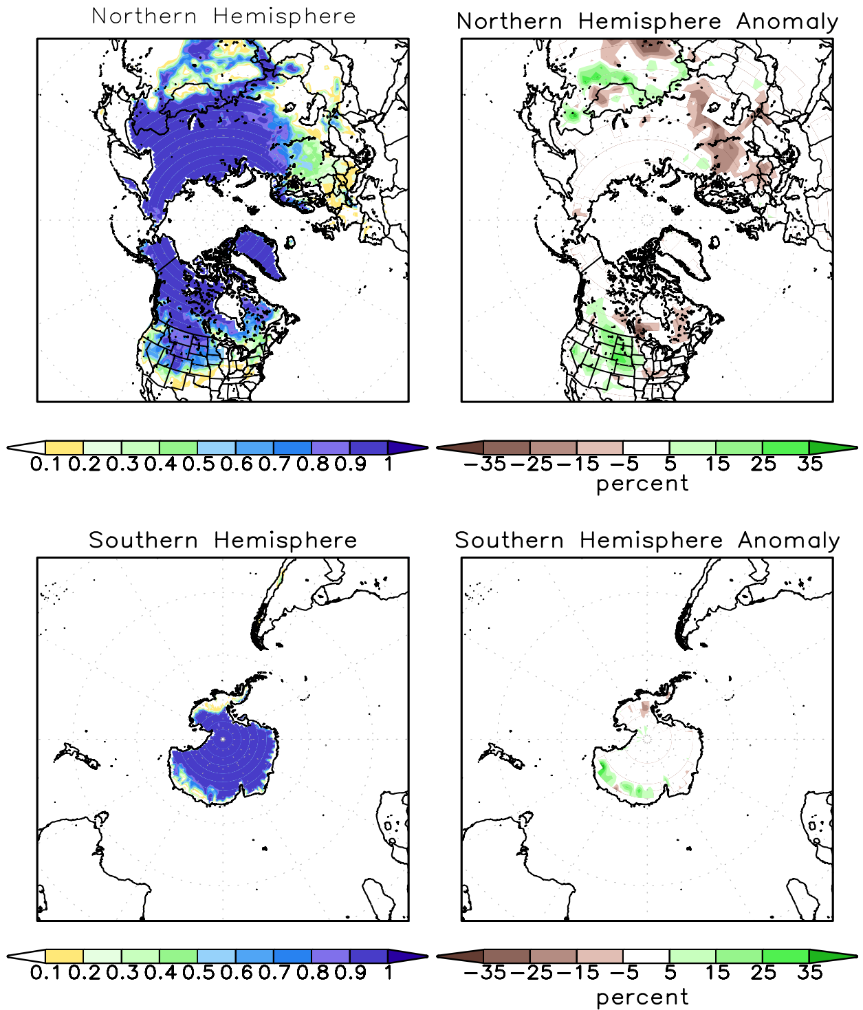
FIGURE A2.2. SSM/I derived snow cover frequency (%) (left) and snow cover anomaly (%) (right) for the month of DEC 2009 based on 1987 - 2006 base period for the Northern Hemisphere (top) and Southern Hemisphere (bottom). It is generated using the algorithm described by Ferraro et. al, 1996, Bull. Amer. Meteor. Soc., vol 77, 891-905.
