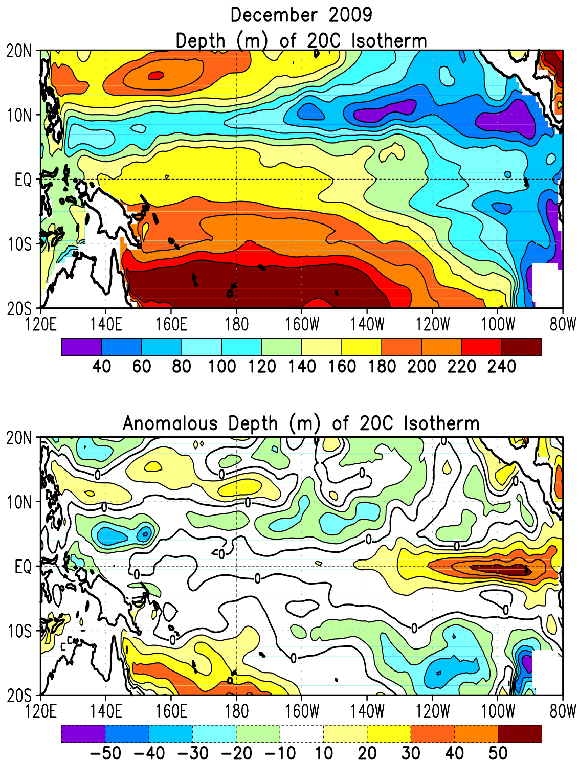
FIGURE T16. Mean (top) and anomalous (bottom) depth of the 20°C isotherm for DEC 2009. Contour interval is 40 m (top) and 10 m (bottom). Dashed contours in bottom panel indicate negative anomalies. Data are derived from the NCEP's global ocean data assimilation system version 2 which assimilates oceanic observations into an oceanic GCM (Xue, Y. and Behringer, D.W., 2006: Operational global ocean data assimilation system at NCEP, to be submitted to BAMS). Anomalies are departures from the 1982–2004 base period means.
