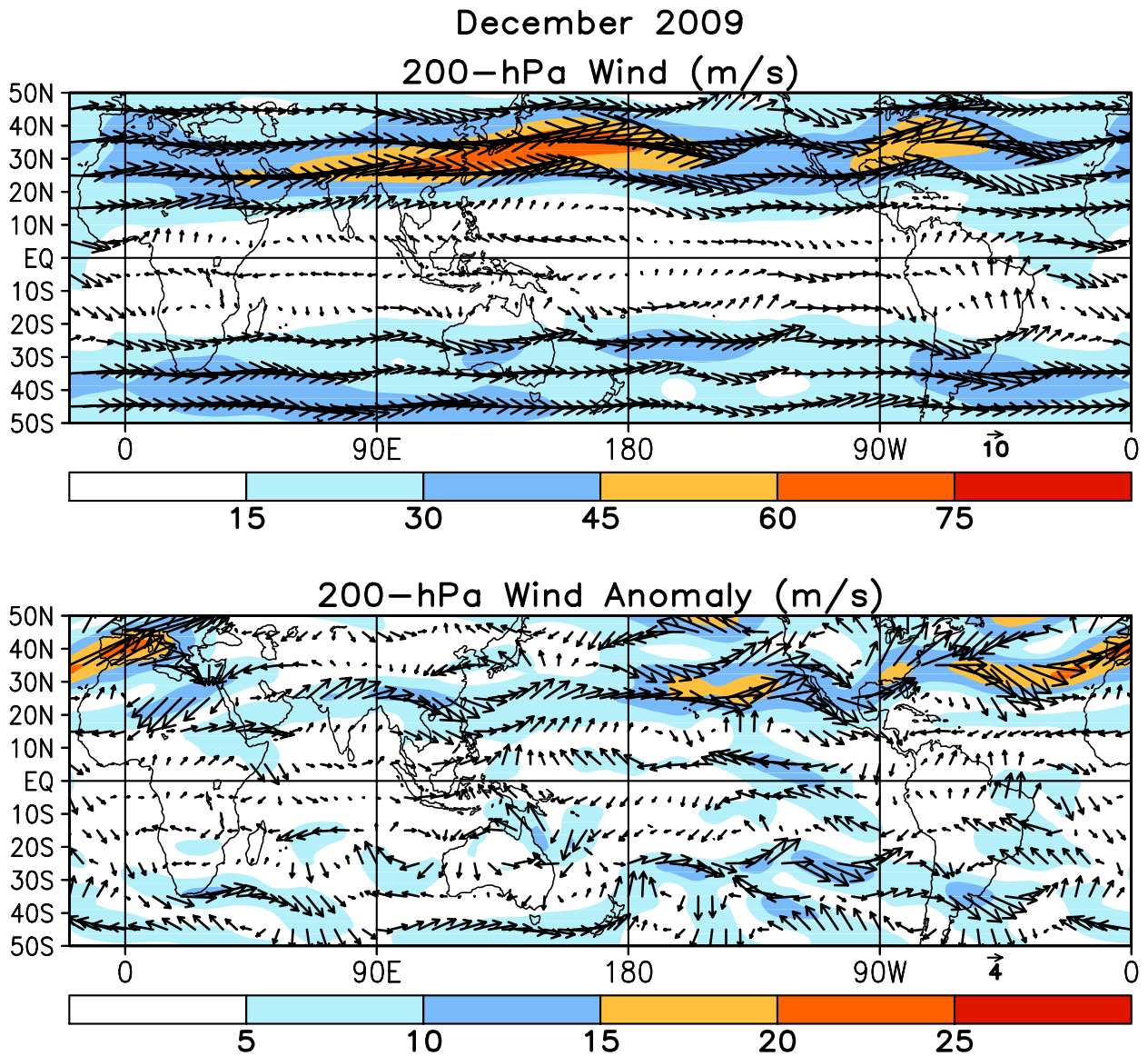
FIGURE T21. Mean (top) and anomalous (bottom) 200-hPa vector wind (CDAS/Reanalysis) for DEC 2009. Contour interval for isotachs is 15 \text{ ms}^{-1} (top) and 5 \text{ ms}^{-1} (bottom). Anomalies are departures from 1979–95 base period monthly means.
