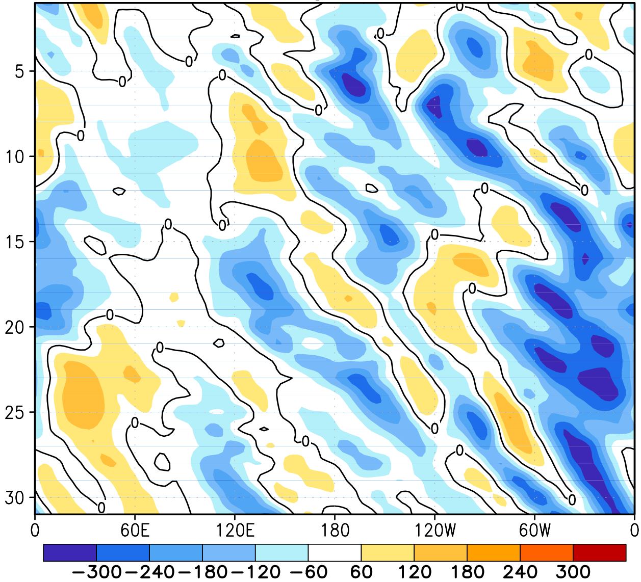
FIGURE E12. Northern Hemisphere: Daily 500-hPa height anomalies for DEC 2009 averaged over the 5° latitude band centered on 40°N. Positive values are indicated by solid contours and dark shading. Negative values are indicated by dashed contours and light shading. Contour interval is 60 m. Anomalies are departures from the 1979-95 base period daily means.
