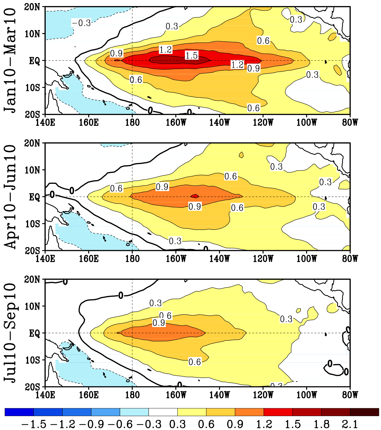
FIGURE F5. Predicted 3-month average sea surface temperature anomalies from the NCEP/CPC Markov model (Xue et al. 2000, J. Climate , 13 , 849-871). The forecast is initiated in DEC 2009 . Contour interval is 0.3C and negative anomalies are indicated by dashed contours. Anomalies are calculated relative to the 1971-2000 climatology.
