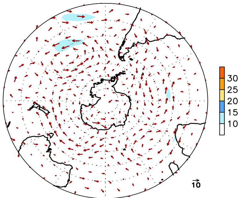
FIGURE E16. Southern Hemisphere mean (left) and anomalous (right) 300-hPa vector wind (CDAS/Reanalysis) for DEC 2009. Mean (anomaly) isotach contour interval is 10 (5) \text{ms}^{-1} . Values greater than 30 \text{ms}^{-1} (left) and 10 \text{ms}^{-1} (rights) are shaded. Anomalies are departures from the 1979-95 base period monthly means.
