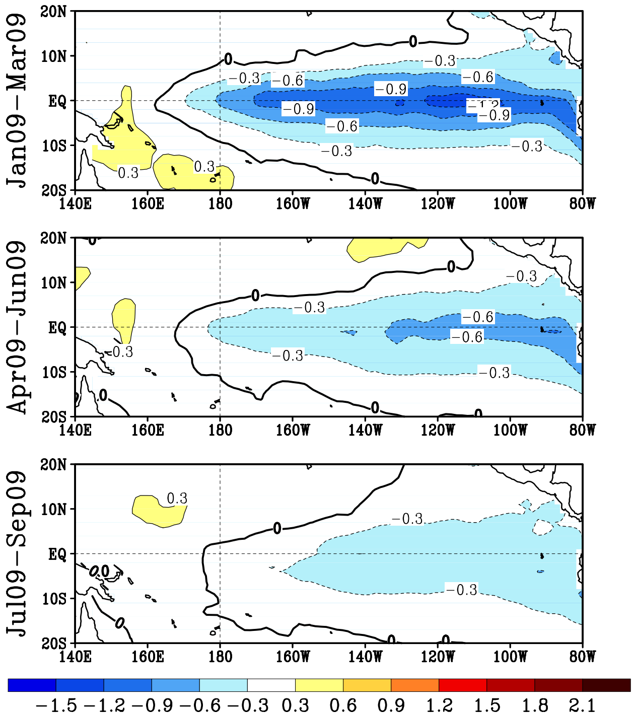
FIGURE F5. Predicted 3-month average sea surface temperature anomalies from the NCEP/CPC Markov model (Xue et al. 2000, J. Climate , 13 , 849-871). The forecast is initiated in DEC 2008 . Contour interval is 0.3C and negative anomalies are indicated by dashed contours. Anomalies are calculated relative to the 1971-2000 climatology.
