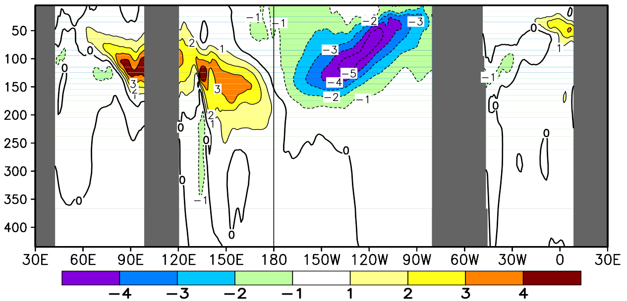
FIGURE T17. Equatorial depth–longitude section of ocean temperature (top) and ocean temperature anomalies (bottom) for DEC 2008. Contour interval is 1°C. Dashed contours in bottom panel indicate negative anomalies. Data are derived from the NCEP’s global ocean data assimilation system version 2 which assimilates oceanic observations into an oceanic GCM (Xue, Y. and Behringer, D.W., 2006: Operational global ocean data assimilation system at NCEP, to be submitted to BAMS). Anomalies are departures from the 1982–2004 base period means.
