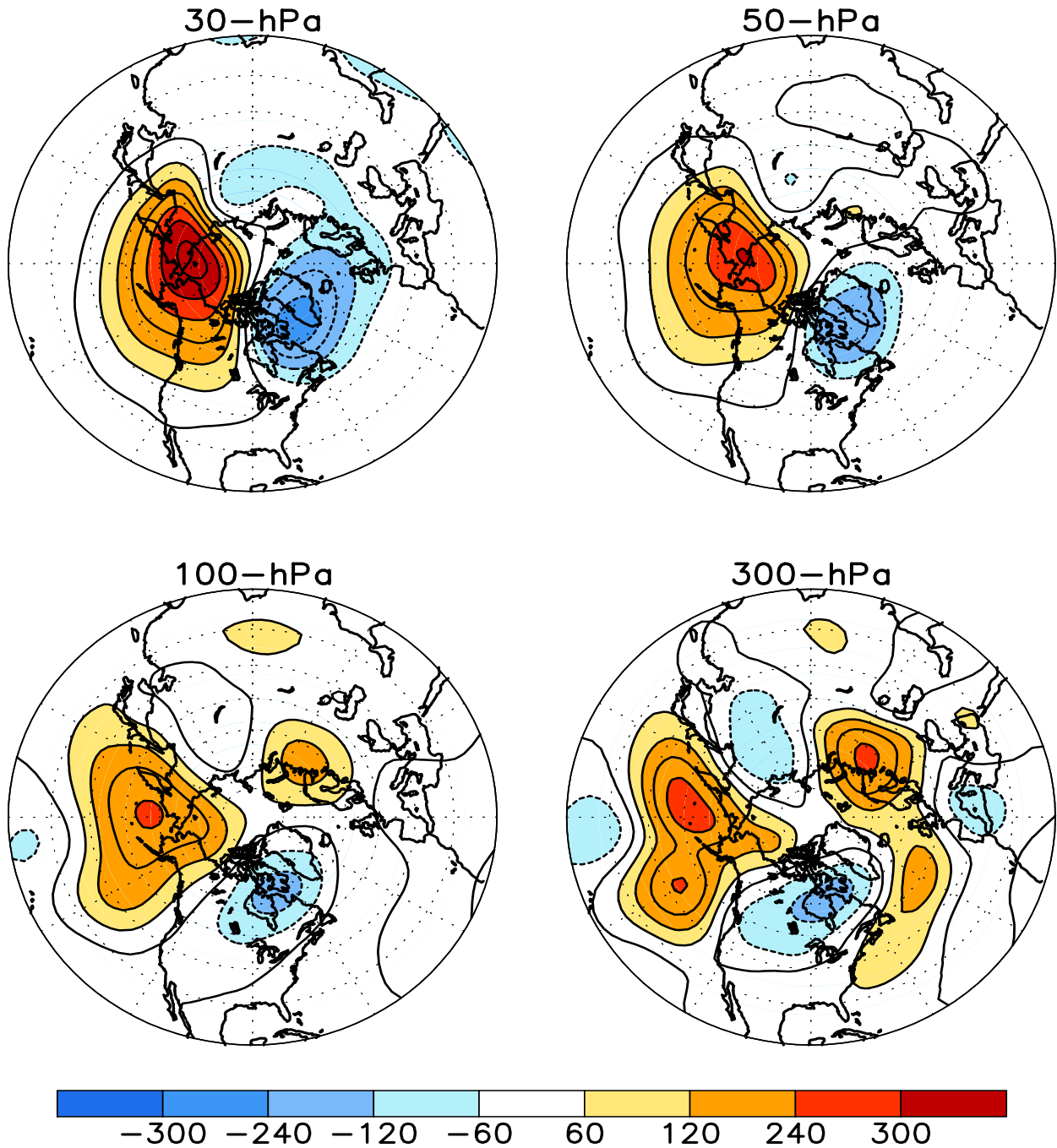
FIGURE S1. Stratospheric height anomalies (m) at selected levels for DEC 2008. Positive values are indicated by solid contours and dark shading. Negative values are indicated by dashed contours and light shading. Contour interval is 60 m. Anomalies are calculated from the 1979–95 base period means. Winter Hemisphere is shown.
