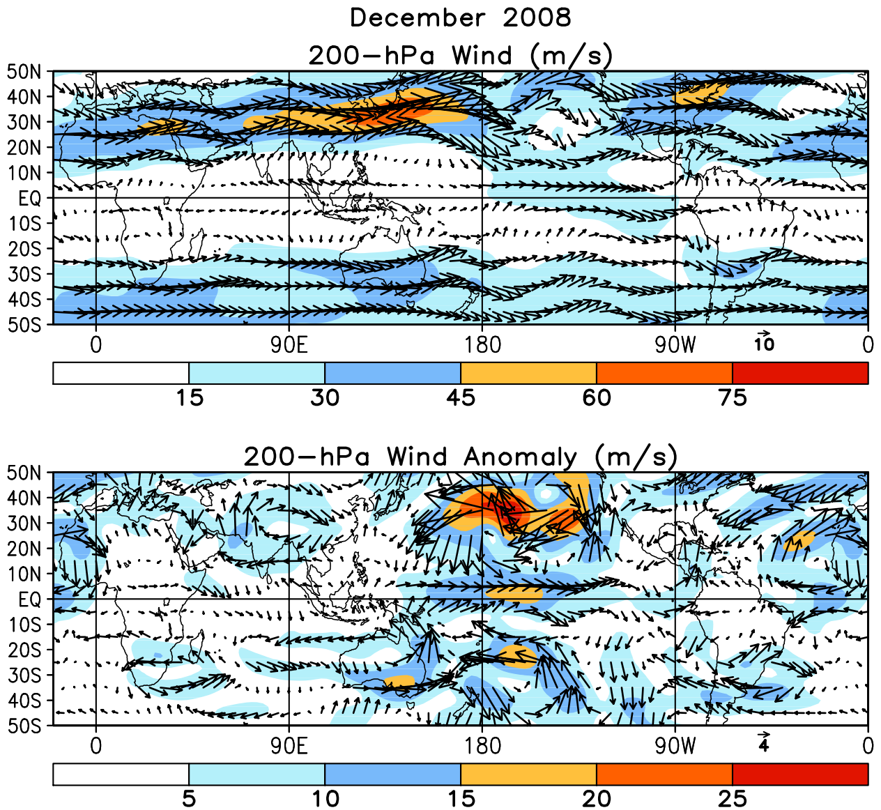
FIGURE T21. Mean (top) and anomalous (bottom) 200-hPa vector wind (CDAS/Reanalysis) for DEC 2008. Contour interval for isotachs is 15 \text{ ms}^{-1} (top) and 5 \text{ ms}^{-1} (bottom). Anomalies are departures from 1979–95 base period monthly means.
