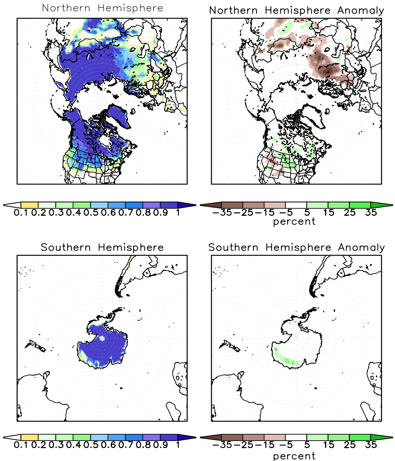
FIGURE A2.2. SSM/I derived snow cover frequency (%) (left) and snow cover anomaly (%) (right) for the month of DEC 2008 based on 1987 - 2006 base period for the Northern Hemisphere (top) and Southern Hemisphere (bottom). It is generated using the algorithm described by Ferraro et. al, 1996, Bull. Amer. Meteor. Soc., vol 77, 891-905.
