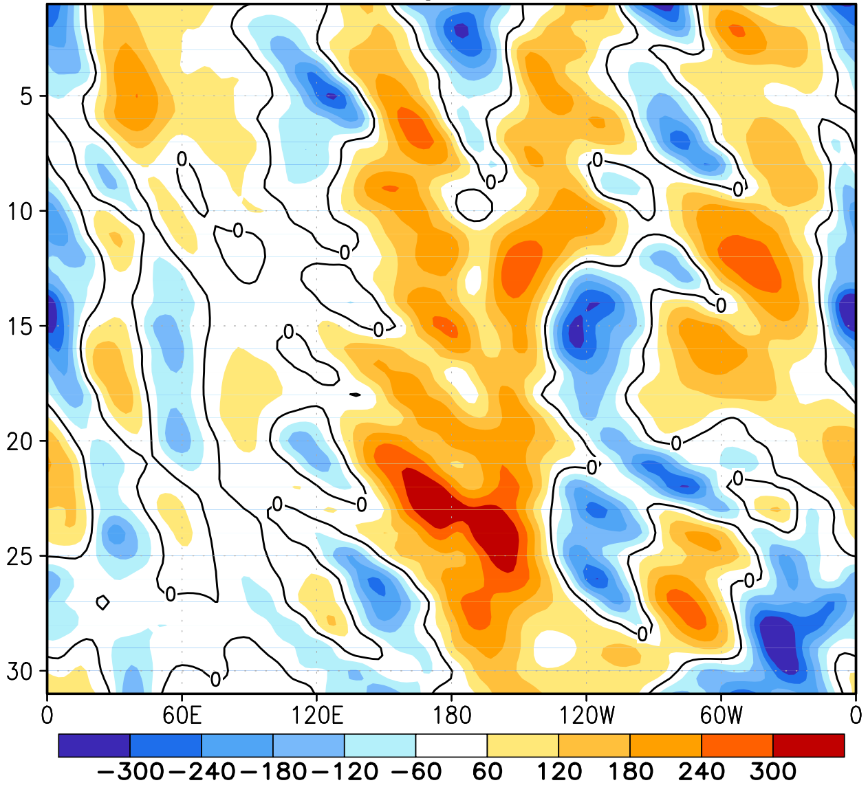
FIGURE E12. Northern Hemisphere: Daily 500-hPa height anomalies for DEC 2008 averaged over the 5° latitude band centered on 40°N. Positive values are indicated by solid contours and dark shading. Negative values are indicated by dashed contours and light shading. Contour interval is 60 m. Anomalies are departures from the 1979-95 base period daily means.
