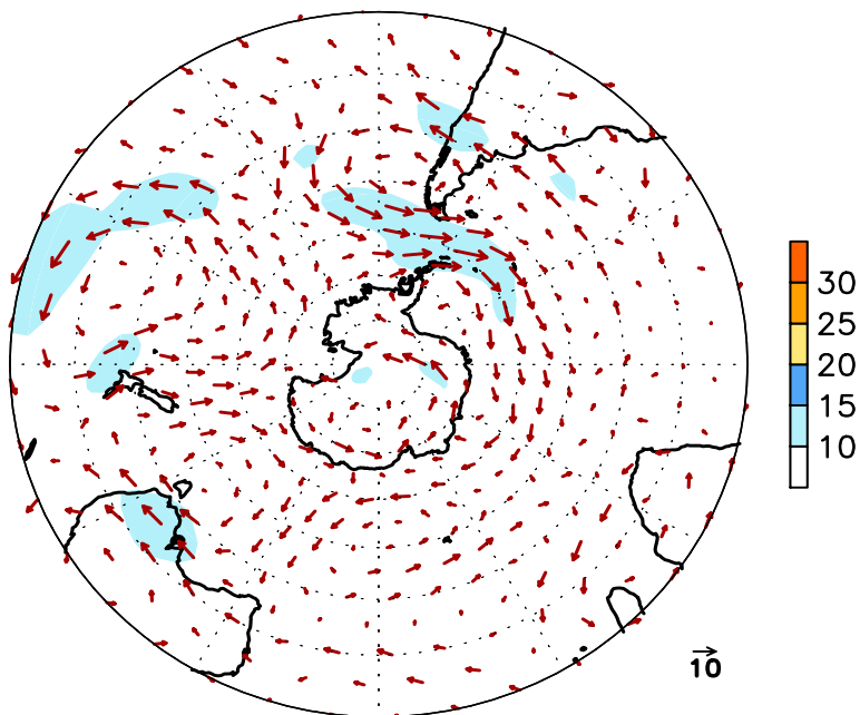
FIGURE E16. Southern Hemisphere mean (left) and anomalous (right) 300-hPa vector wind (CDAS/Reanalysis) for DEC 2008. Mean (anomaly) isotach contour interval is 10 (5) \text{ms}^{-1} . Values greater than 30 \text{ms}^{-1} (left) and 10 \text{ms}^{-1} (rights) are shaded. Anomalies are departures from the 1979-95 base period monthly means.
