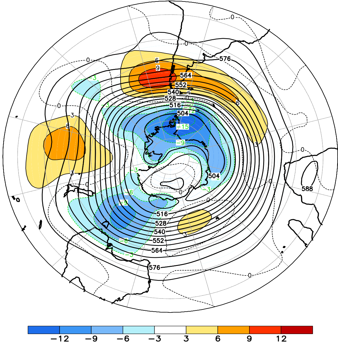
FIGURE E15. Southern Hemisphere mean and anomalous 500-hPa geopotential height (CDAS/Reanalysis) for DEC 2008. Mean heights are denoted by solid contours drawn at an interval of 6 dam. Anomaly contour interval is 3 dam with values less (greater) than -3 dam (3 dam) indicated by dark (light) shading. Anomalies are calculated as departures from the 1979-95 base period monthly means.
