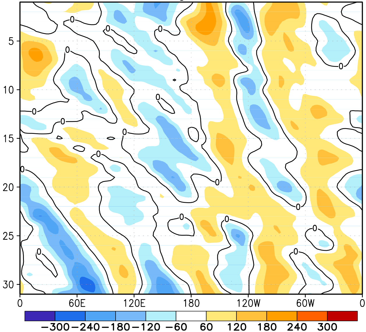
FIGURE E18. Southern Hemisphere: Daily 500-hPa height anomalies for DEC 2008 averaged over the 5° latitude band centered on 40°S. Positive values are indicated by solid contours and dark shading. Negative values are indicated by dashed contours and light shading. Contour interval is 60 m. Anomalies are departures from the 1979-95 base period daily means.
