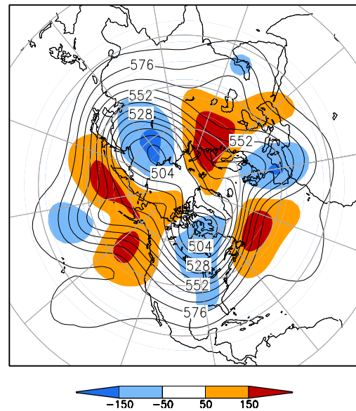
500-hPa Height (dm) & Anomalies (m) (Dec 1–15, 2008)
