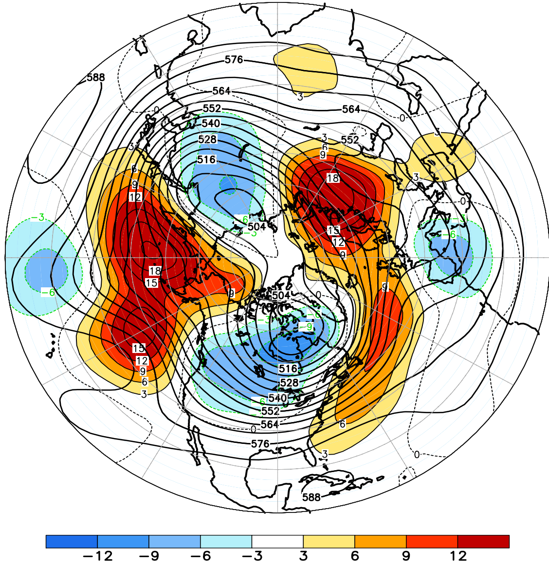
FIGURE E9. Northern Hemisphere mean and anomalous 500-hPa geopotential height (CDAS/Reanalysis) for DEC 2008. Mean heights are denoted by solid contours drawn at an interval of 6 dam. Anomaly contour interval is 3 dam with values less (greater) than -3 dam (3 dam) indicated by dark (light) shading. Anomalies are calculated as departures from the 1979-95 base period monthly means.
