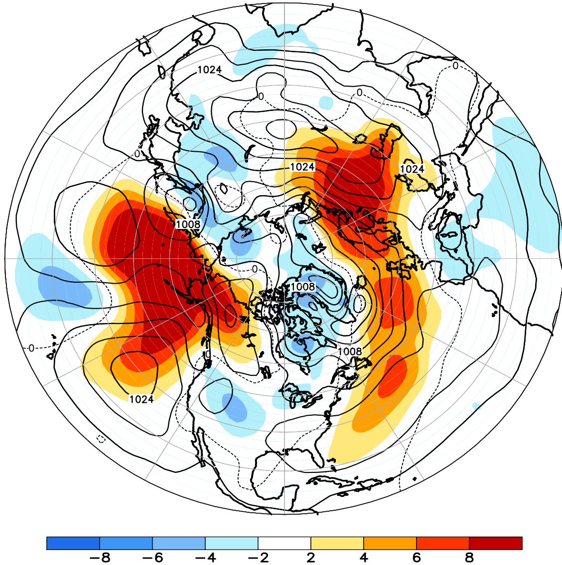
FIGURE E8. Northern Hemisphere mean and anomalous sea level pressure (CDAS/Reanalysis) for DEC 2008. Mean values are denoted by solid contours drawn at an interval of 4 hPa. Anomaly contour interval is 2 hPa with values less (greater) than -2 hPa (2 hPa) indicated by dark (light) shading. Anomalies are calculated as departures from the 1979-95 base period monthly means.
