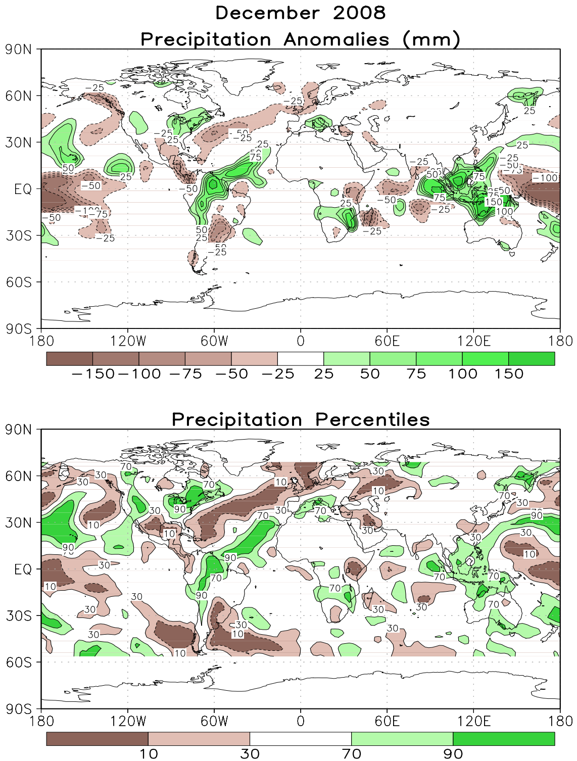
FIGURE E3. Anomalous precipitation (mm, top) and precipitation percentiles based on a Gamma distribution fit to the 1979–2000 base period data (bottom) for DEC 2008. Data are obtained from a merge of raingauge observations and satellite-derived precipitation estimates (Janowiak and Xie 1999, J. Climate , 12 , 3335–3342). Contours are drawn at 200, 100, 50, 25, -25, -50, -100, and -200 mm in top panel. Percentiles are not plotted in regions where mean monthly precipitation is <5mm/month.
