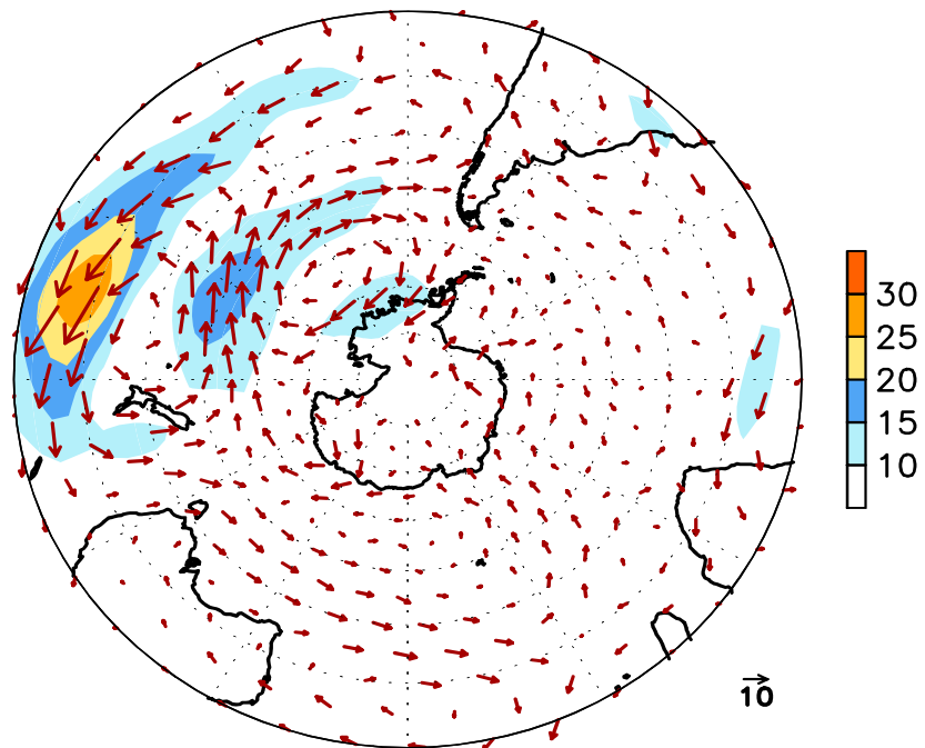
FIGURE E16. Southern Hemisphere mean (left) and anomalous (right) 300-hPa vector wind (CDAS/Reanalysis) for AUG 2022. Mean (anomaly) isotach contour interval is 10 (5) \text{ms}^{-1} . Values greater than 30 \text{ms}^{-1} (left) and 10 \text{ms}^{-1} (rights) are shaded. Anomalies are departures from the 1991-2020 base period monthly means.
