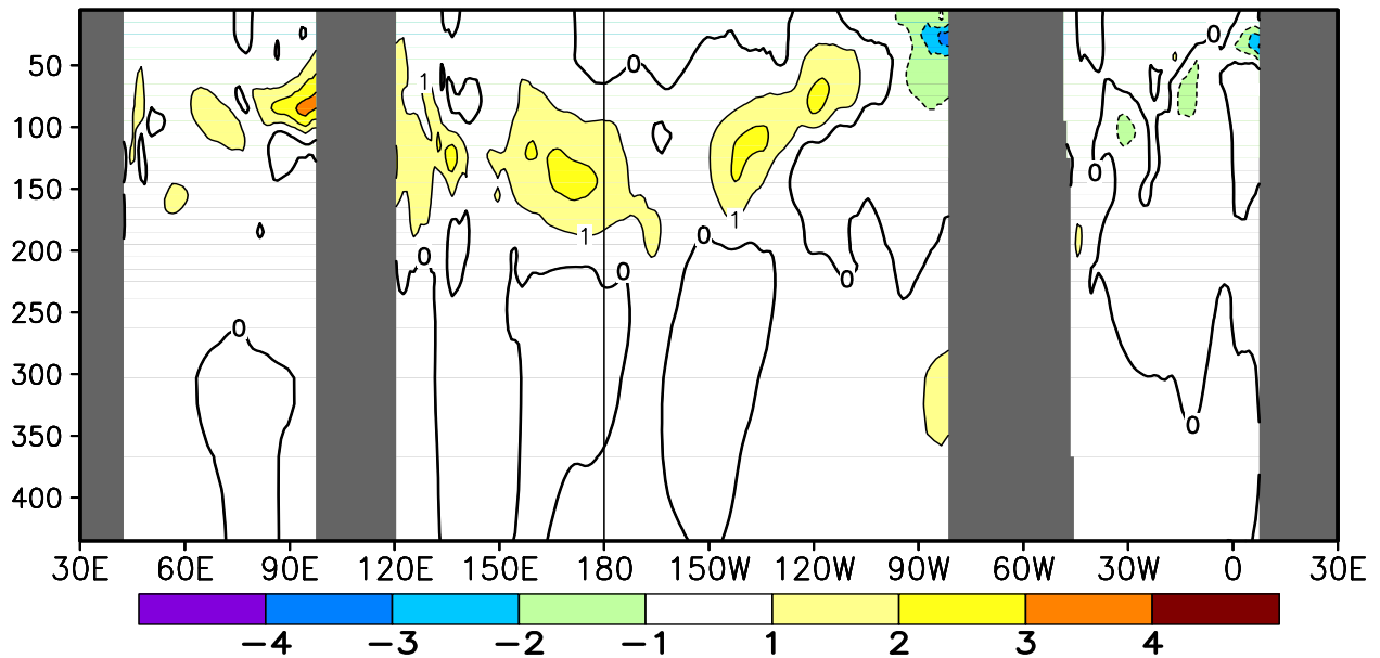
FIGURE T17. Equatorial depth–longitude section of ocean temperature (top) and ocean temperature anomalies (bottom) for AUG 2013. Contour interval is 1°C. Dashed contours in bottom panel indicate negative anomalies. Data are derived from the NCEP’s global ocean data assimilation system version 2 which assimilates oceanic observations into an oceanic GCM (Xue, Y. and Behringer, D.W., 2006: Operational global ocean data assimilation system at NCEP, to be submitted to BAMS). Anomalies are departures from the 1981–2010 base period means.
