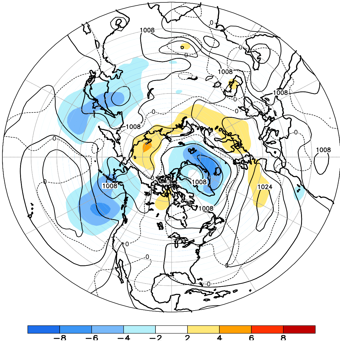
FIGURE E8. Northern Hemisphere mean and anomalous sea level pressure (CDAS/Reanalysis) for AUG 2013. Mean values are denoted by solid contours drawn at an interval of 4 hPa. Anomaly contour interval is 2 hPa with values less (greater) than -2 hPa (2 hPa) indicated by dark (light) shading. Anomalies are calculated as departures from the 1981-2010 base period monthly means.
