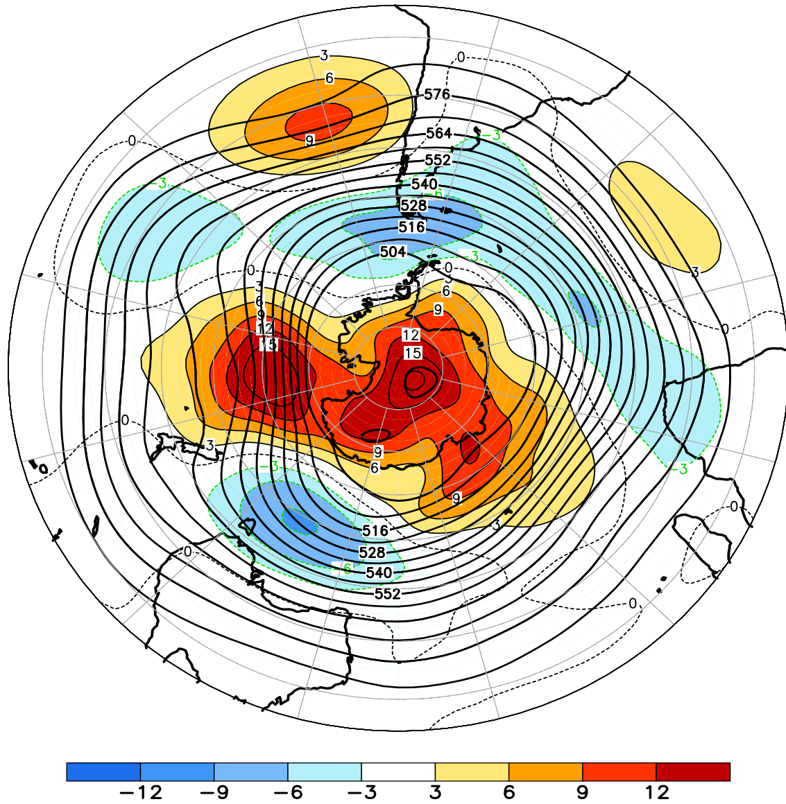
FIGURE E15. Southern Hemisphere mean and anomalous 500-hPa geopotential height (CDAS/Reanalysis) for AUG 2013. Mean heights are denoted by solid contours drawn at an interval of 6 dam. Anomaly contour interval is 3 dam with values less (greater) than -3 dam (3 dam) indicated by dark (light) shading. Anomalies are calculated as departures from the 1981-2010 base period monthly means.
