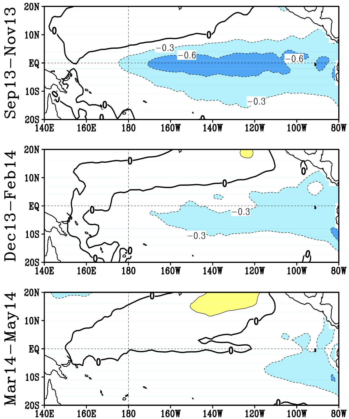
FIGURE F5. Predicted 3-month average sea surface temperature anomalies from the NCEP/CPC Markov model (Xue et al. 2000, J. Climate , 13 , 849-871). The forecast is initiated in AUG 2013. Contour interval is 0.3C and negative anomalies are indicated by dashed contours. Anomalies are calculated relative to the 1971-2000 climatology.
