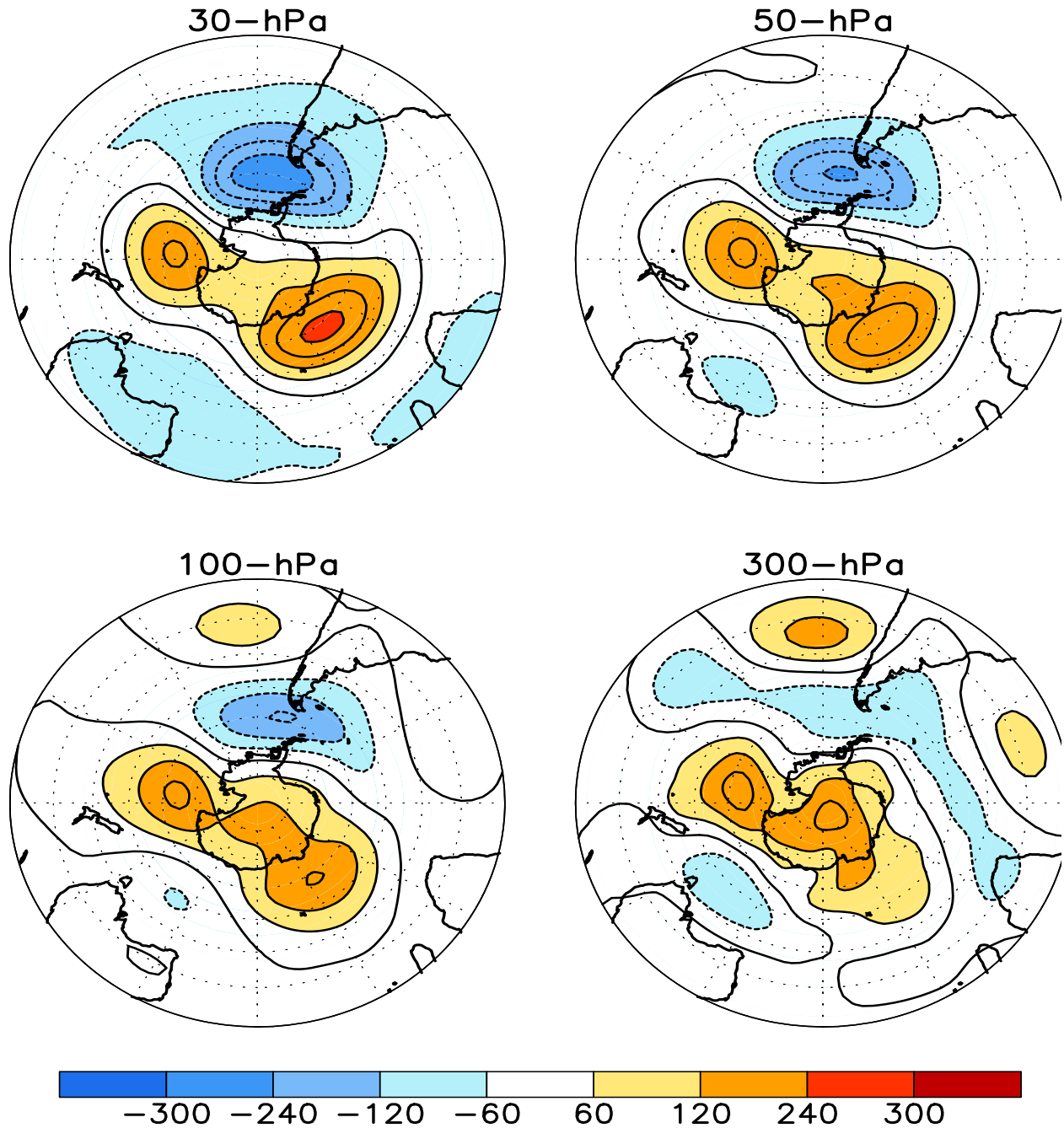
FIGURE S1. Stratospheric height anomalies (m) at selected levels for AUG 2013. Positive values are indicated by solid contours and dark shading. Negative values are indicated by dashed contours and light shading. Contour interval is 60 m. Anomalies are calculated from the 1981-2010 base period means. Winter Hemisphere is shown.
