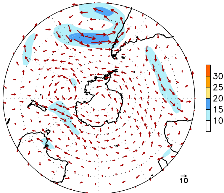
FIGURE E16. Southern Hemisphere mean (left) and anomalous (right) 300-hPa vector wind (CDAS/Reanalysis) for AUG 2013. Mean (anomaly) isotach contour interval is 10 (5) \text{ms}^{-1} . Values greater than 30 \text{ms}^{-1} (left) and 10 \text{ms}^{-1} (rights) are shaded. Anomalies are departures from the 1981-2010 base period monthly means.
