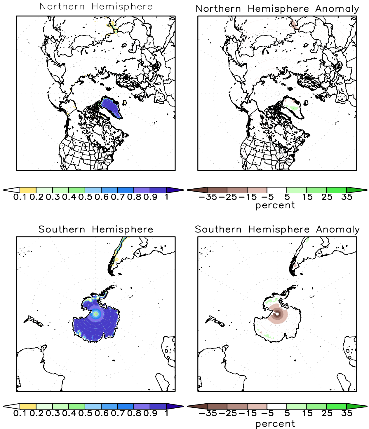
FIGURE A2.2. SSM/I derived snow cover frequency (%) (left) and snow cover anomaly (%) (right) for the month of AUG 2013 based on 1987 - 2010 base period for the Northern Hemisphere (top) and Southern Hemisphere (bottom). It is generated using the algorithm described by Ferraro et. al, 1996, Bull. Amer. Meteor. Soc., vol 77, 891-905.
