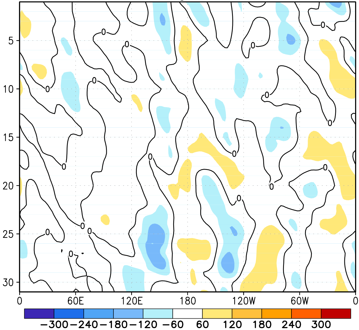
FIGURE E12. Northern Hemisphere: Daily 500-hPa height anomalies for AUG 2013 averaged over the 5° latitude band centered on 40°N. Positive values are indicated by solid contours and dark shading. Negative values are indicated by dashed contours and light shading. Contour interval is 60 m. Anomalies are departures from the 1981-2010 base period daily means.
