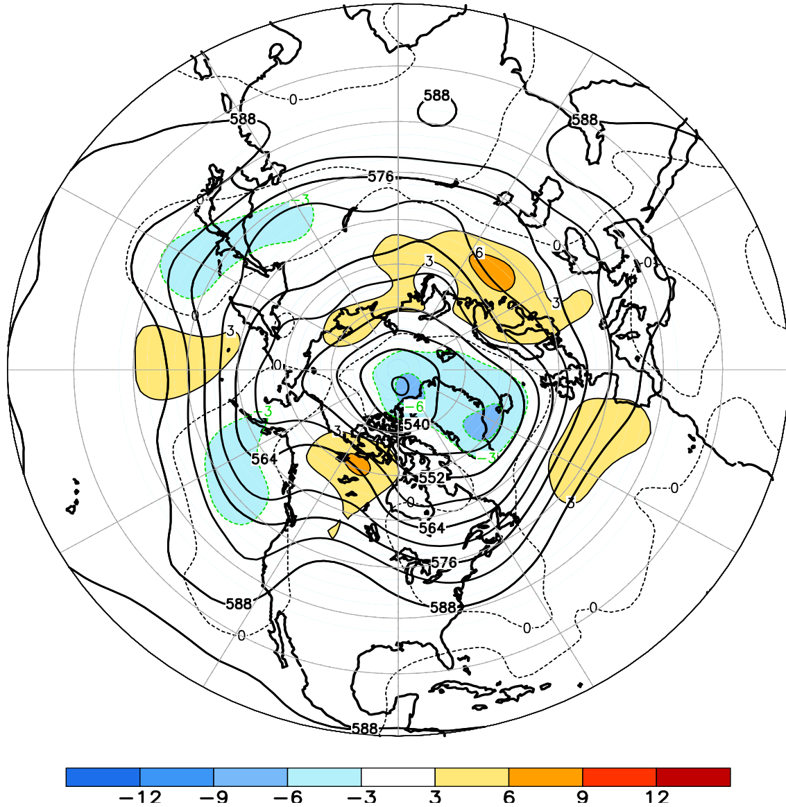
FIGURE E9. Northern Hemisphere mean and anomalous 500-hPa geopotential height (CDAS/Reanalysis) for AUG 2013. Mean heights are denoted by solid contours drawn at an interval of 6 dam. Anomaly contour interval is 3 dam with values less (greater) than -3 dam (3 dam) indicated by dark (light) shading. Anomalies are calculated as departures from the 1981-2010 base period monthly means.
