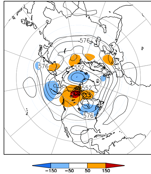
500-hPa Height (dm) & Anomalies (m) (Aug 1–15, 2013)
