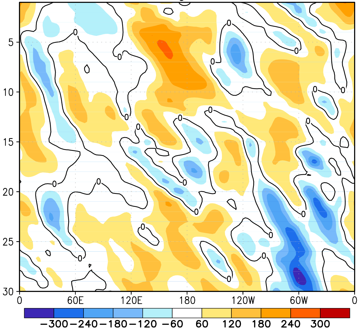
FIGURE E12. Northern Hemisphere: Daily 500-hPa height anomalies for APR 2015 averaged over the 5° latitude band centered on 40°N. Positive values are indicated by solid contours and dark shading. Negative values are indicated by dashed contours and light shading. Contour interval is 60 m. Anomalies are departures from the 1981-2010 base period daily means.
