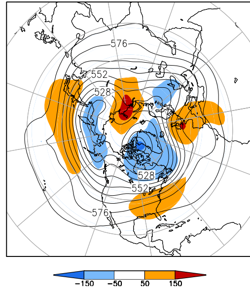
500-hPa Height (dm) & Anomalies (m) (Apr 1–15, 2015)
