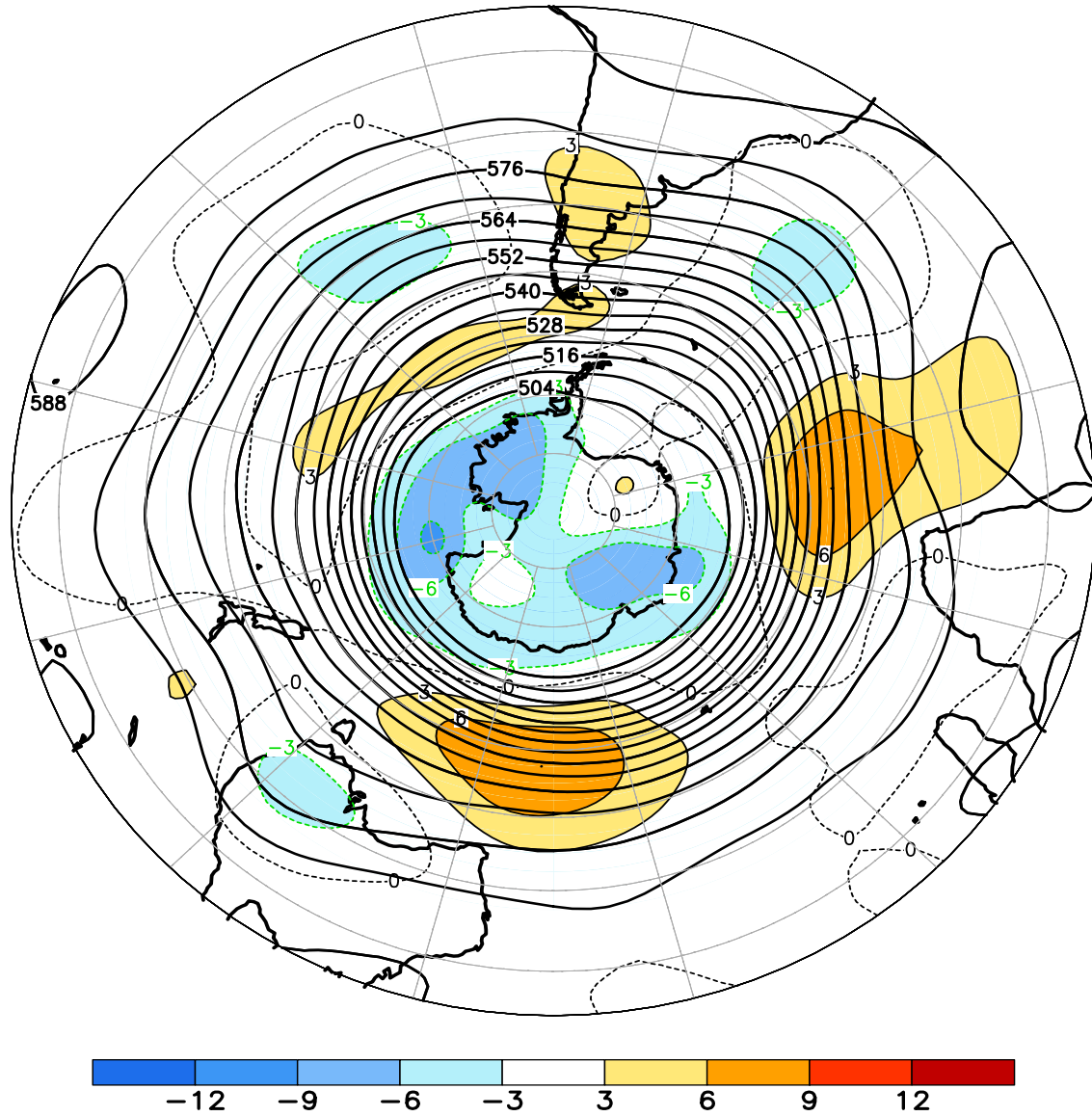
FIGURE E15. Southern Hemisphere mean and anomalous 500-hPa geopotential height (CDAS/Reanalysis) for APR 2015. Mean heights are denoted by solid contours drawn at an interval of 6 dam. Anomaly contour interval is 3 dam with values less (greater) than -3 dam (3 dam) indicated by dark (light) shading. Anomalies are calculated as departures from the 1981-2010 base period monthly means.
