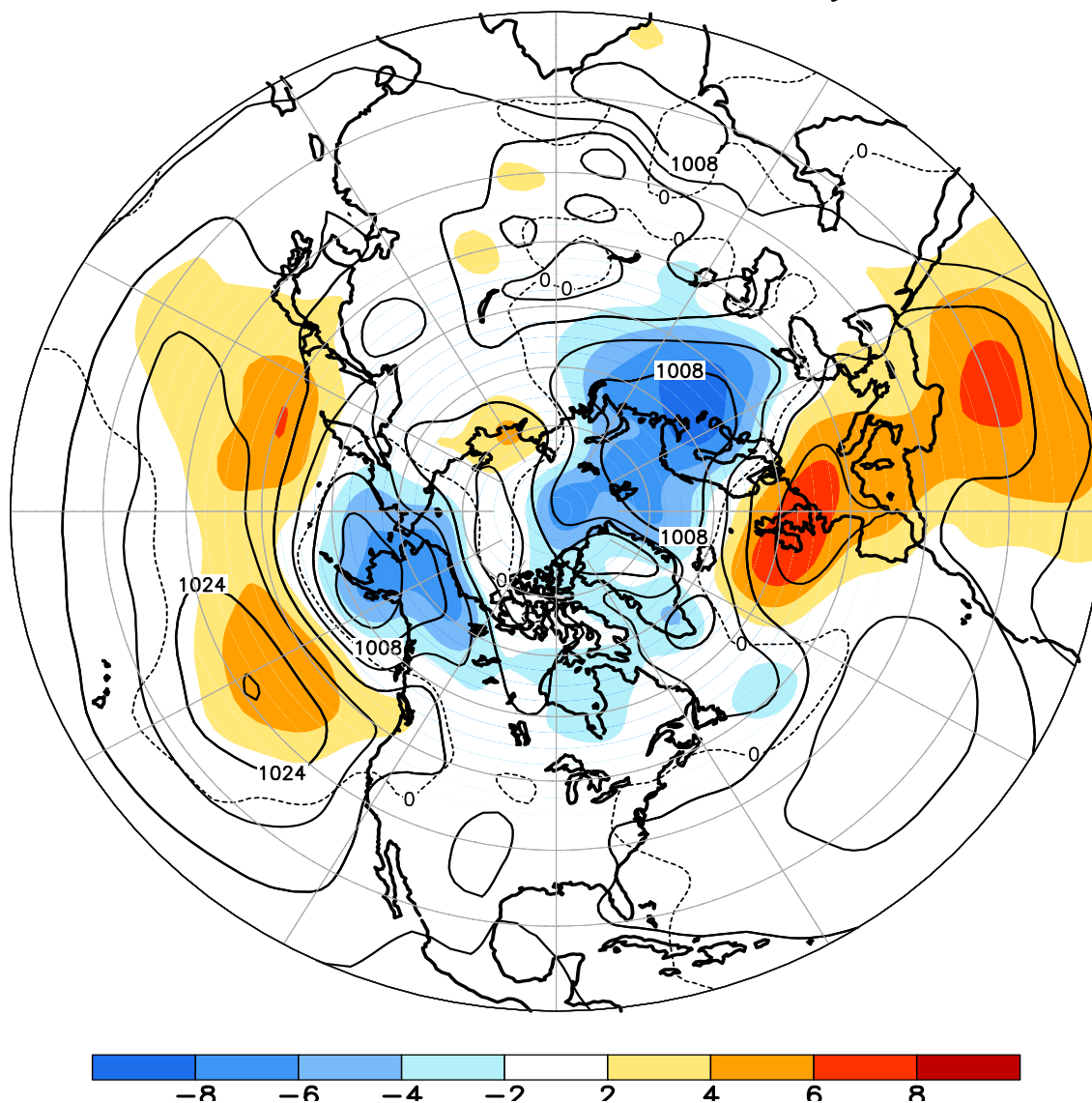
FIGURE E8. Northern Hemisphere mean and anomalous sea level pressure (CDAS/Reanalysis) for APR 2015. Mean values are denoted by solid contours drawn at an interval of 4 hPa. Anomaly contour interval is 2 hPa with values less (greater) than -2 hPa (2 hPa) indicated by dark (light) shading. Anomalies are calculated as departures from the 1981-2010 base period monthly means.
