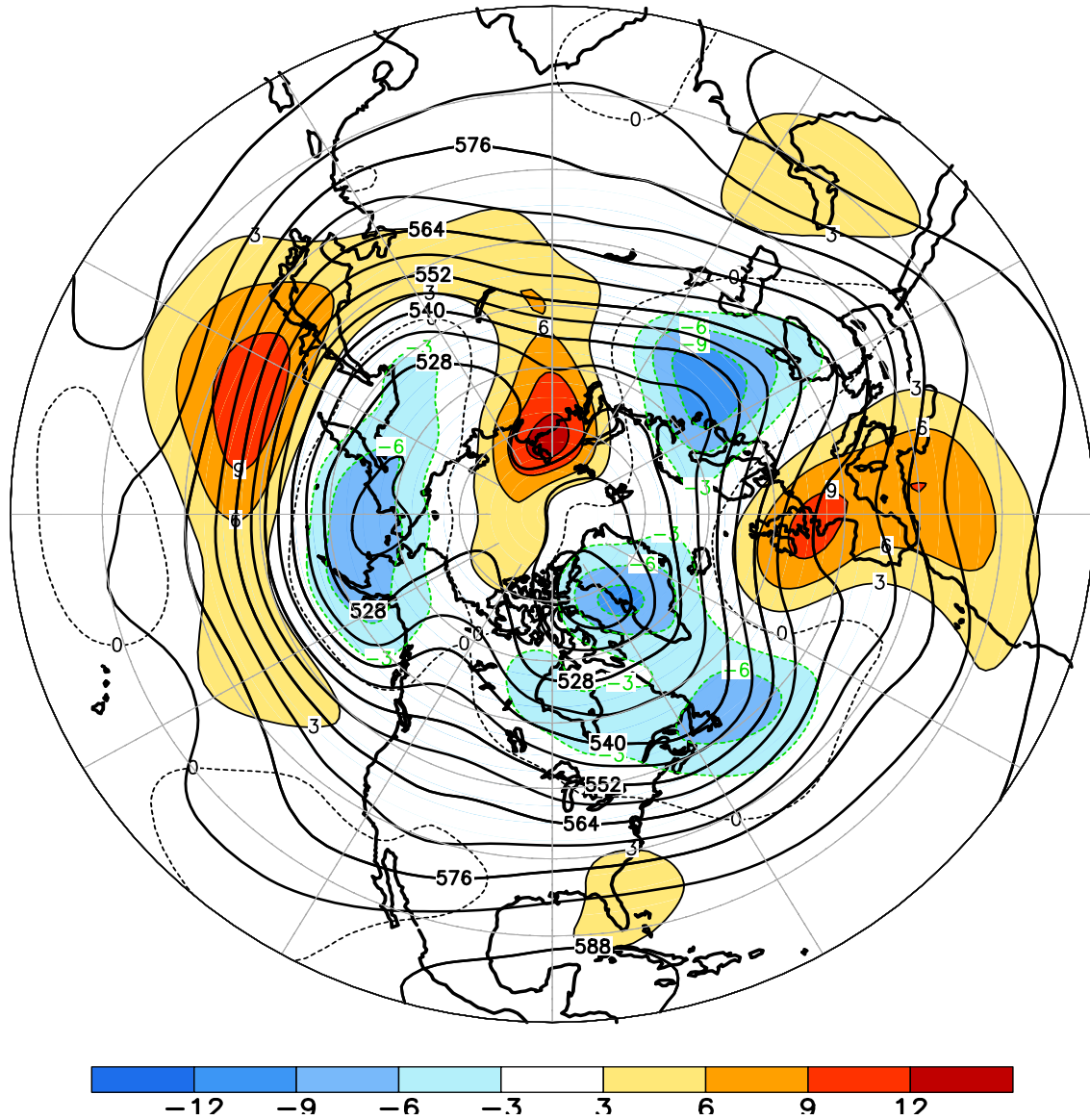
FIGURE E9. Northern Hemisphere mean and anomalous 500-hPa geopotential height (CDAS/Reanalysis) for APR 2015. Mean heights are denoted by solid contours drawn at an interval of 6 dam. Anomaly contour interval is 3 dam with values less (greater) than -3 dam (3 dam) indicated by dark (light) shading. Anomalies are calculated as departures from the 1981-2010 base period monthly means.
