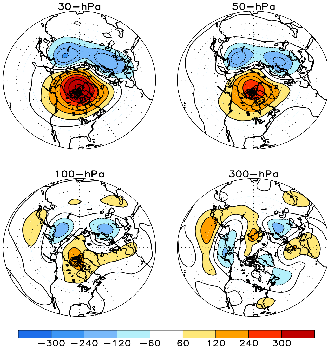
FIGURE S1. Stratospheric height anomalies (m) at selected levels for APR 2015. Positive values are indicated by solid contours and dark shading. Negative values are indicated by dashed contours and light shading. Contour interval is 60 m. Anomalies are calculated from the 1981-2010 base period means. Winter Hemisphere is shown.
