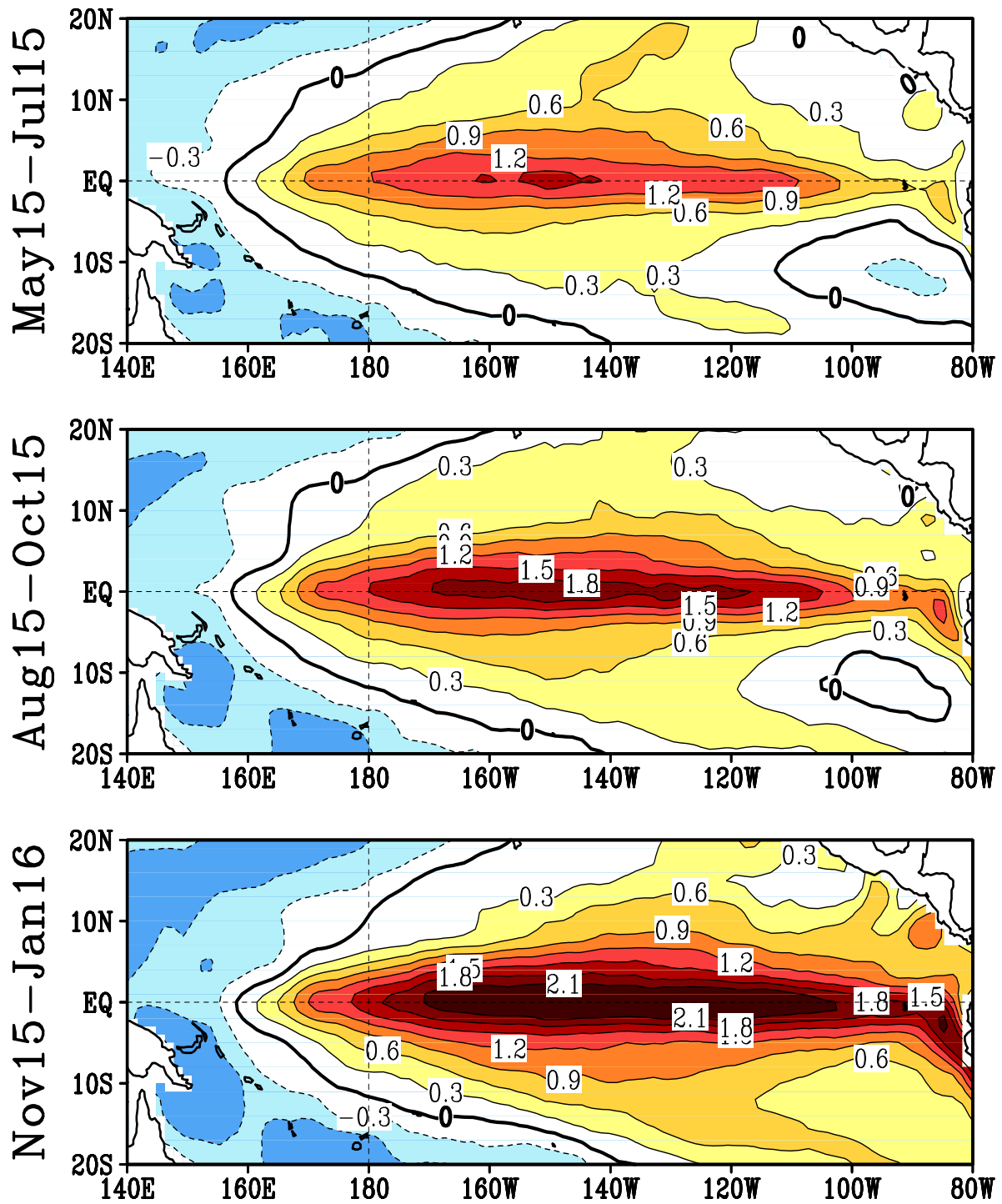
FIGURE F5. Predicted 3-month average sea surface temperature anomalies from the NCEP/CPC Markov model (Xue et al. 2000, J. Climate , 13 , 849-871). The forecast is initiated in APR 2015 . Contour interval is 0.3C and negative anomalies are indicated by dashed contours. Anomalies are calculated relative to the 1971-2000 climatology.
