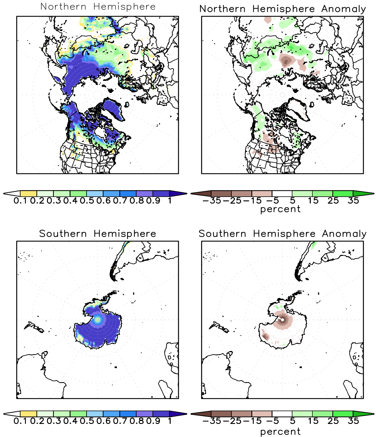
FIGURE A2.2. SSM/I derived snow cover frequency (%) (left) and snow cover anomaly (%) (right) for the month of APR 2015 based on 1987 - 2010 base period for the Northern Hemisphere (top) and Southern Hemisphere (bottom). It is generated using the algorithm described by Ferraro et. al, 1996, Bull. Amer. Meteor. Soc., vol 77, 891-905.
