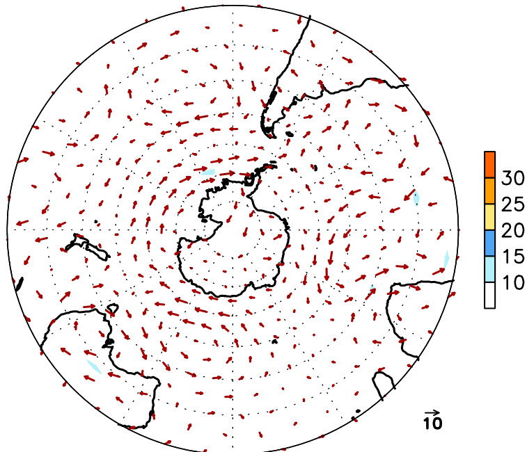
FIGURE E16. Southern Hemisphere mean (left) and anomalous (right) 300-hPa vector wind (CDAS/Reanalysis) for APR 2015. Mean (anomaly) isotach contour interval is 10 (5) \text{ms}^{-1} . Values greater than 30 \text{ms}^{-1} (left) and 10 \text{ms}^{-1} (rights) are shaded. Anomalies are departures from the 1981-2010 base period monthly means.
