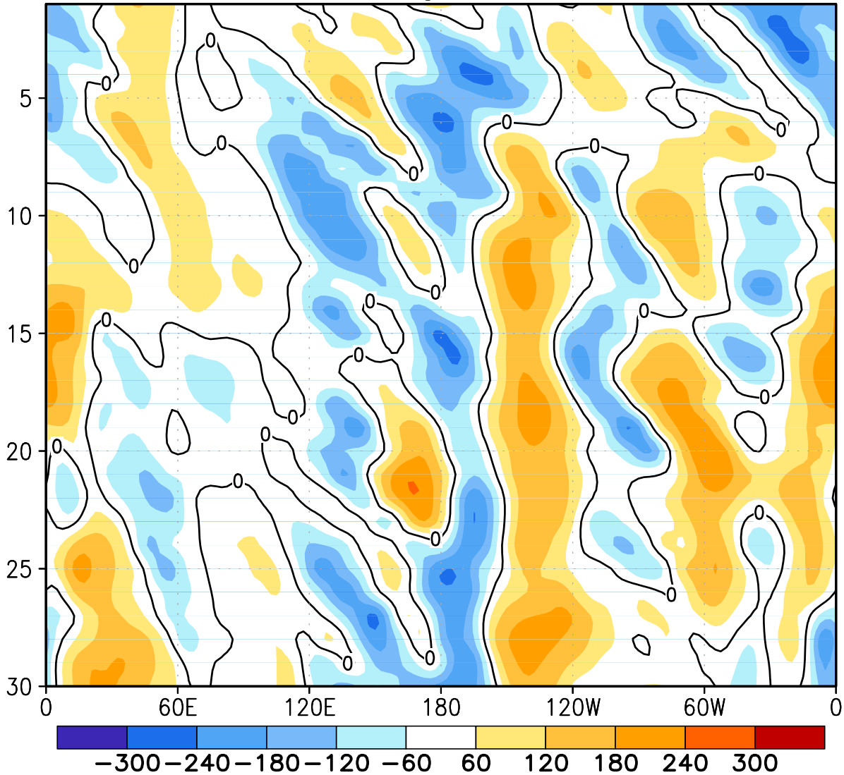
FIGURE E12. Northern Hemisphere: Daily 500-hPa height anomalies for APR 2013 averaged over the 5° latitude band centered on 40°N. Positive values are indicated by solid contours and dark shading. Negative values are indicated by dashed contours and light shading. Contour interval is 60 m. Anomalies are departures from the 1981-2010 base period daily means.
