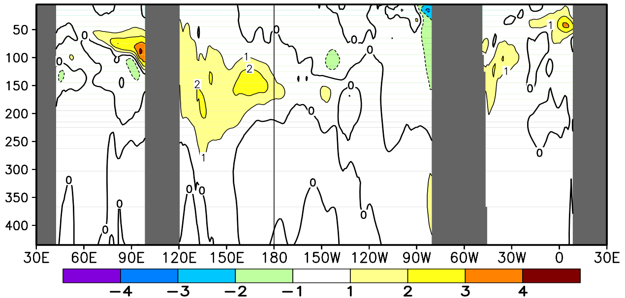
FIGURE T17. Equatorial depth–longitude section of ocean temperature (top) and ocean temperature anomalies (bottom) for APR 2013. Contour interval is 1°C. Dashed contours in bottom panel indicate negative anomalies. Data are derived from the NCEP’s global ocean data assimilation system version 2 which assimilates oceanic observations into an oceanic GCM (Xue, Y. and Behringer, D.W., 2006: Operational global ocean data assimilation system at NCEP, to be submitted to BAMS). Anomalies are departures from the 1981–2010 base period means.
