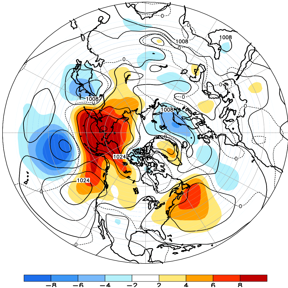
FIGURE E8. Northern Hemisphere mean and anomalous sea level pressure (CDAS/Reanalysis) for APR 2013. Mean values are denoted by solid contours drawn at an interval of 4 hPa. Anomaly contour interval is 2 hPa with values less (greater) than -2 hPa (2 hPa) indicated by dark (light) shading. Anomalies are calculated as departures from the 1981-2010 base period monthly means.
