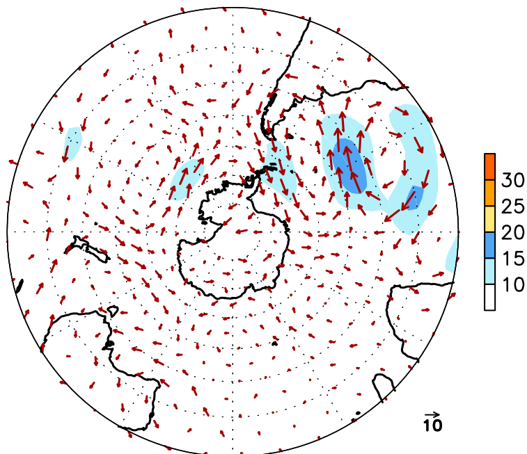
FIGURE E16. Southern Hemisphere mean (left) and anomalous (right) 300-hPa vector wind (CDAS/Reanalysis) for APR 2013. Mean (anomaly) isotach contour interval is 10 (5) \text{ms}^{-1} . Values greater than 30 \text{ms}^{-1} (left) and 10 \text{ms}^{-1} (rights) are shaded. Anomalies are departures from the 1981-2010 base period monthly means.
