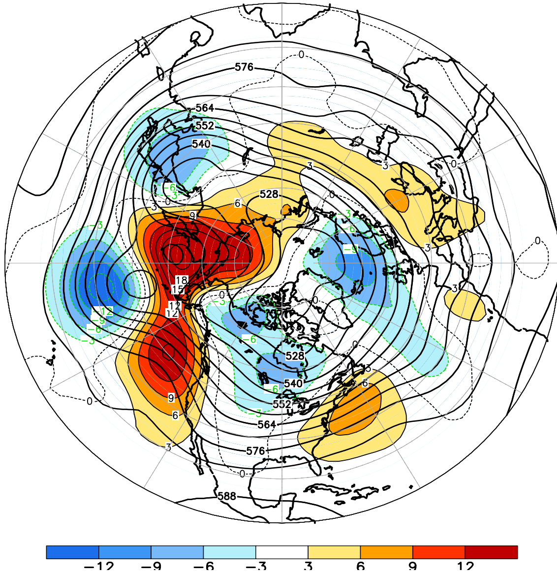
FIGURE E9. Northern Hemisphere mean and anomalous 500-hPa geopotential height (CDAS/Reanalysis) for APR 2013. Mean heights are denoted by solid contours drawn at an interval of 6 dam. Anomaly contour interval is 3 dam with values less (greater) than -3 dam (3 dam) indicated by dark (light) shading. Anomalies are calculated as departures from the 1981-2010 base period monthly means.
