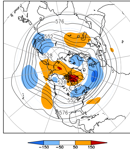
500-hPa Height (dm) & Anomalies (m) (Apr 1–15, 2013)
