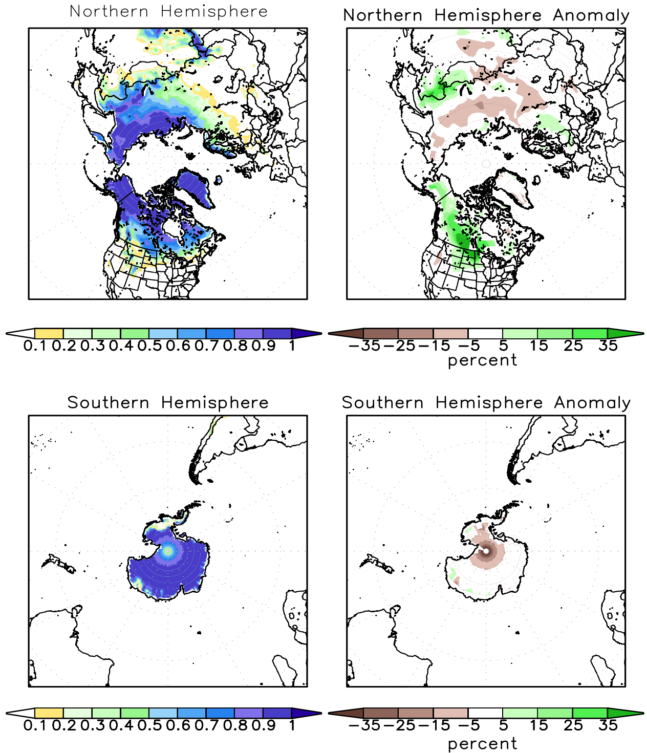
FIGURE A2.2. SSM/I derived snow cover frequency (%) (left) and snow cover anomaly (%) (right) for the month of APR 2013 based on 1987 - 2010 base period for the Northern Hemisphere (top) and Southern Hemisphere (bottom). It is generated using the algorithm described by Ferraro et. al, 1996, Bull. Amer. Meteor. Soc., vol 77, 891-905.
