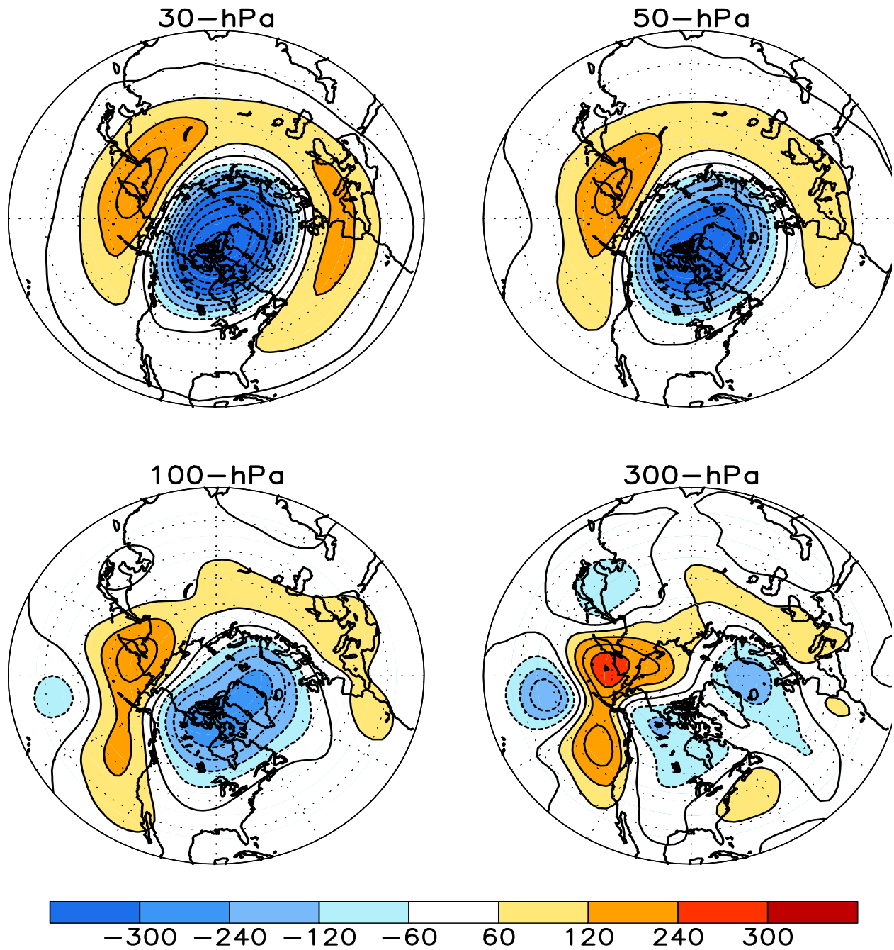
FIGURE S1. Stratospheric height anomalies (m) at selected levels for APR 2013. Positive values are indicated by solid contours and dark shading. Negative values are indicated by dashed contours and light shading. Contour interval is 60 m. Anomalies are calculated from the 1981-2010 base period means. Winter Hemisphere is shown.
