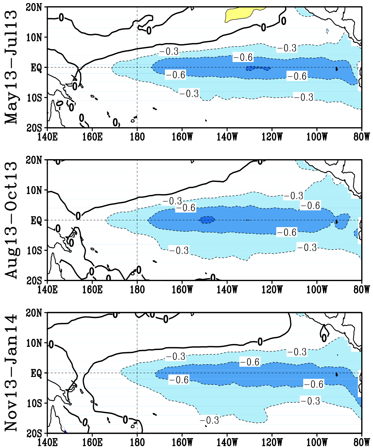
FIGURE F5. Predicted 3-month average sea surface temperature anomalies from the NCEP/CPC Markov model (Xue et al. 2000, J. Climate , 13 , 849-871). The forecast is initiated in APR 2013 . Contour interval is 0.3C and negative anomalies are indicated by dashed contours. Anomalies are calculated relative to the 1971-2000 climatology.
