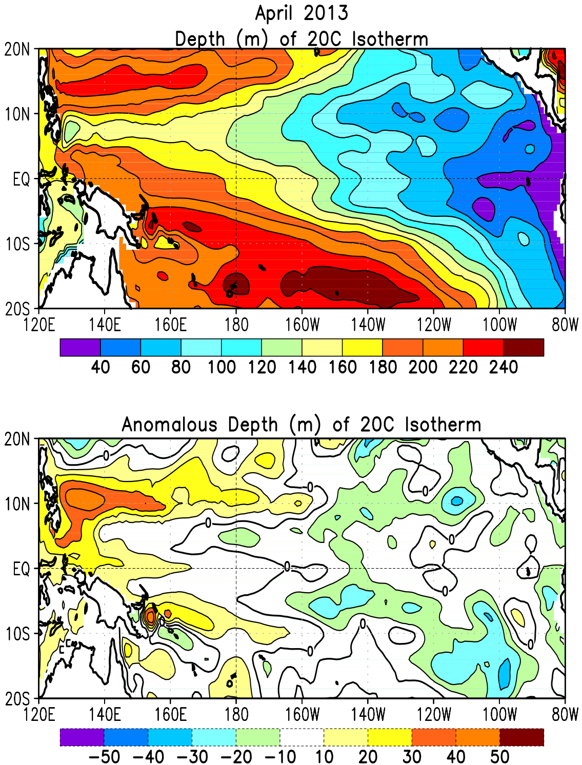
FIGURE T16. Mean (top) and anomalous (bottom) depth of the 20°C isotherm for APR 2013. Contour interval is 40 m (top) and 10 m (bottom). Dashed contours in bottom panel indicate negative anomalies. Data are derived from the NCEP’s global ocean data assimilation system version 2 which assimilates oceanic observations into an oceanic GCM (Xue, Y. and Behringer, D.W., 2006: Operational global ocean data assimilation system at NCEP, to be submitted to BAMS). Anomalies are departures from the 1981–2010 base period means.
