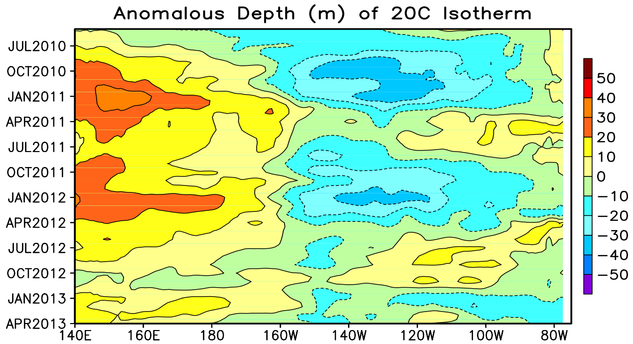
FIGURE T15. Mean (top) and anomalous (bottom) depth of the 20C isotherm averaged between 5N-5S in the Pacific Ocean. Data are derived from the NCEP's global ocean data assimilation system which assimilates oceanic observations into an oceanic GCM (Behringer, D. W., and Y. Xue, 2004: Evaluation of the global ocean data assimilation system at NCEP: The Pacific Ocean. AMS 84th Annual Meeting, Seattle, Washington, 11-15). The contour interval is 10 m. Dashed contours in bottom panel indicate negative anomalies. Anomalies are departures from the 1981-2010 base period means.
