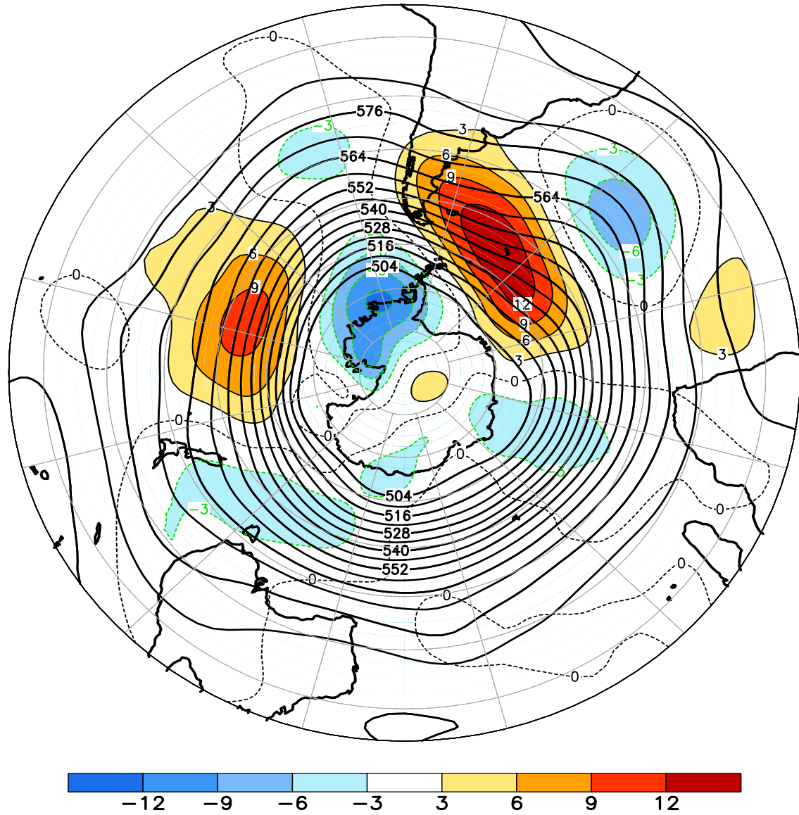
FIGURE E15. Southern Hemisphere mean and anomalous 500-hPa geopotential height (CDAS/Reanalysis) for APR 2013. Mean heights are denoted by solid contours drawn at an interval of 6 dam. Anomaly contour interval is 3 dam with values less (greater) than -3 dam (3 dam) indicated by dark (light) shading. Anomalies are calculated as departures from the 1981-2010 base period monthly means.
